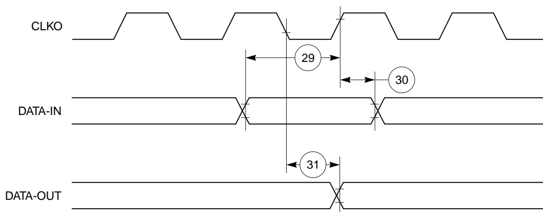
Figure 42. Parallel I/O Data-In/Data-Out Timing Diagram
