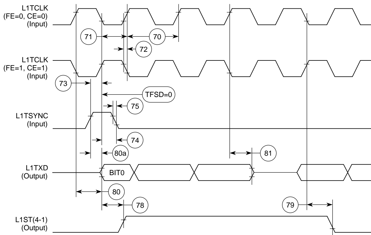
Figure 52. SI Transmit Timing Diagram (DSC = 0)
