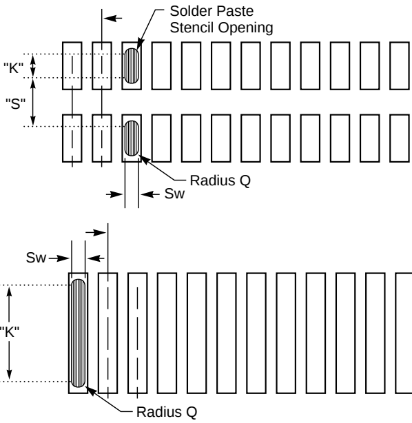
Series 752 & 753 Stencil Openings
