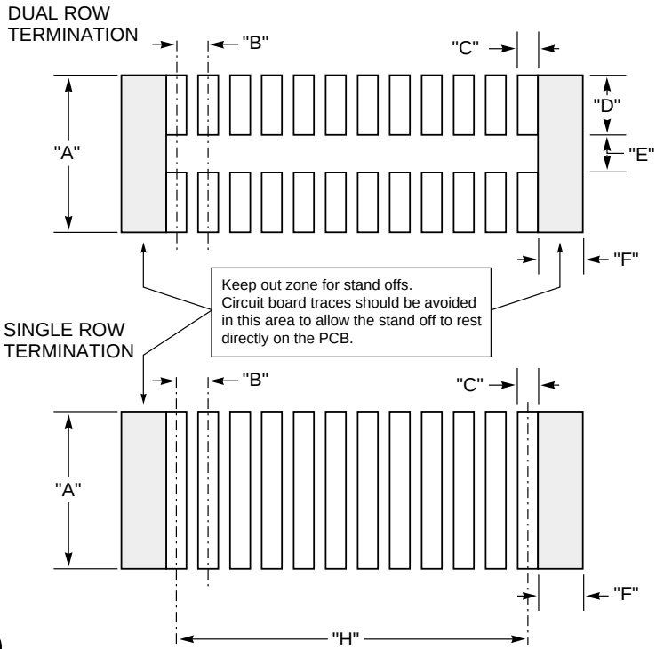
Series 752 & 753 Land Patterns
