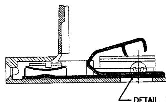
SECTION X-X
