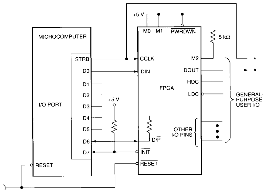
Figure 24. Slave Mode
