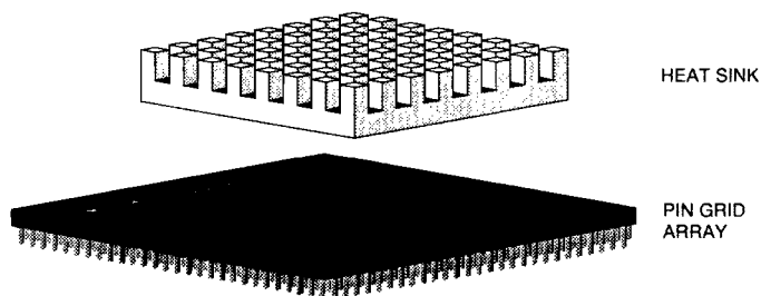
Figure 11-20. Heat Sink with Adhesive
