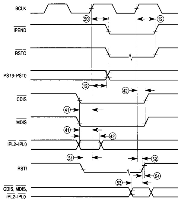
Figure 11-11. Other Signal Timing
