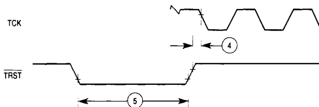
Figure 11-2. \overline{\text{TRST}} Timing Diagram
