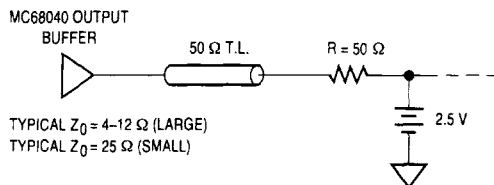
Figure 11-18. MC68040 Termination Network
