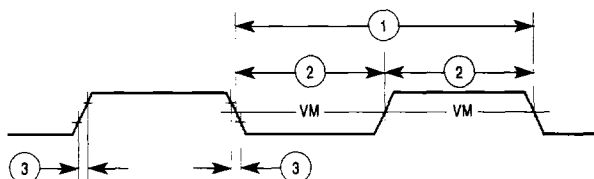
Figure 11-1. Clock Input Timing Diagram
