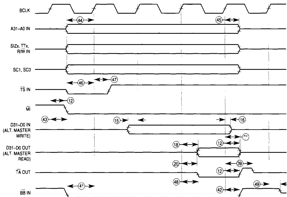
Figure 11-15. Snoop Hit Timing
