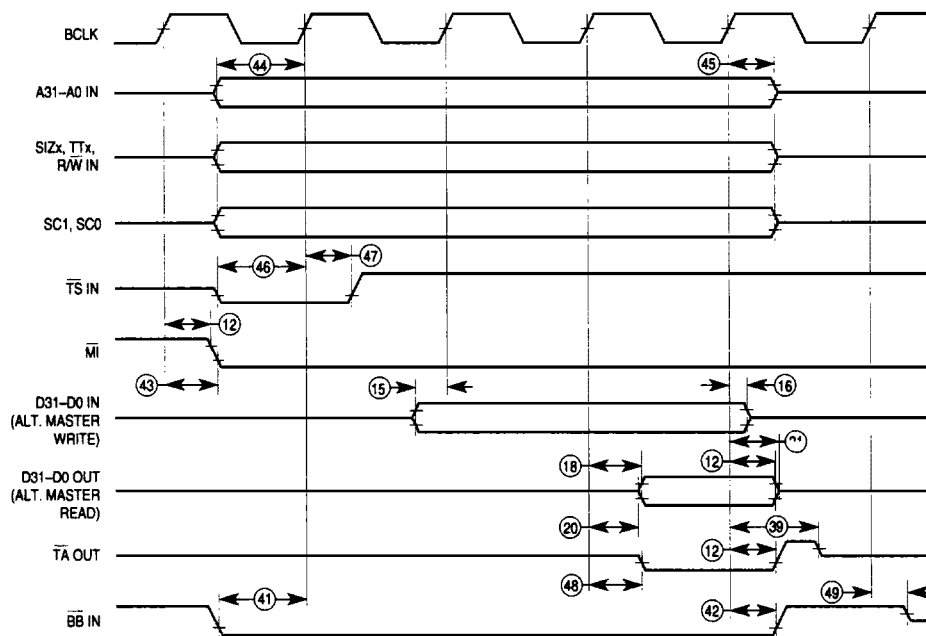
Figure 11-9. Snoop Hit Timing
