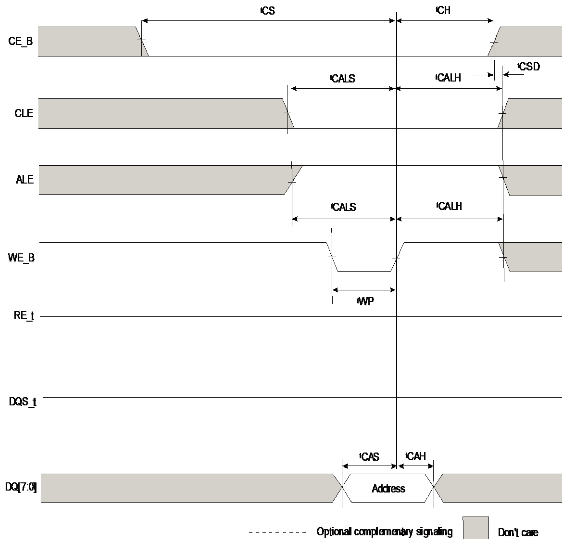
Figure 48. Address cycle
