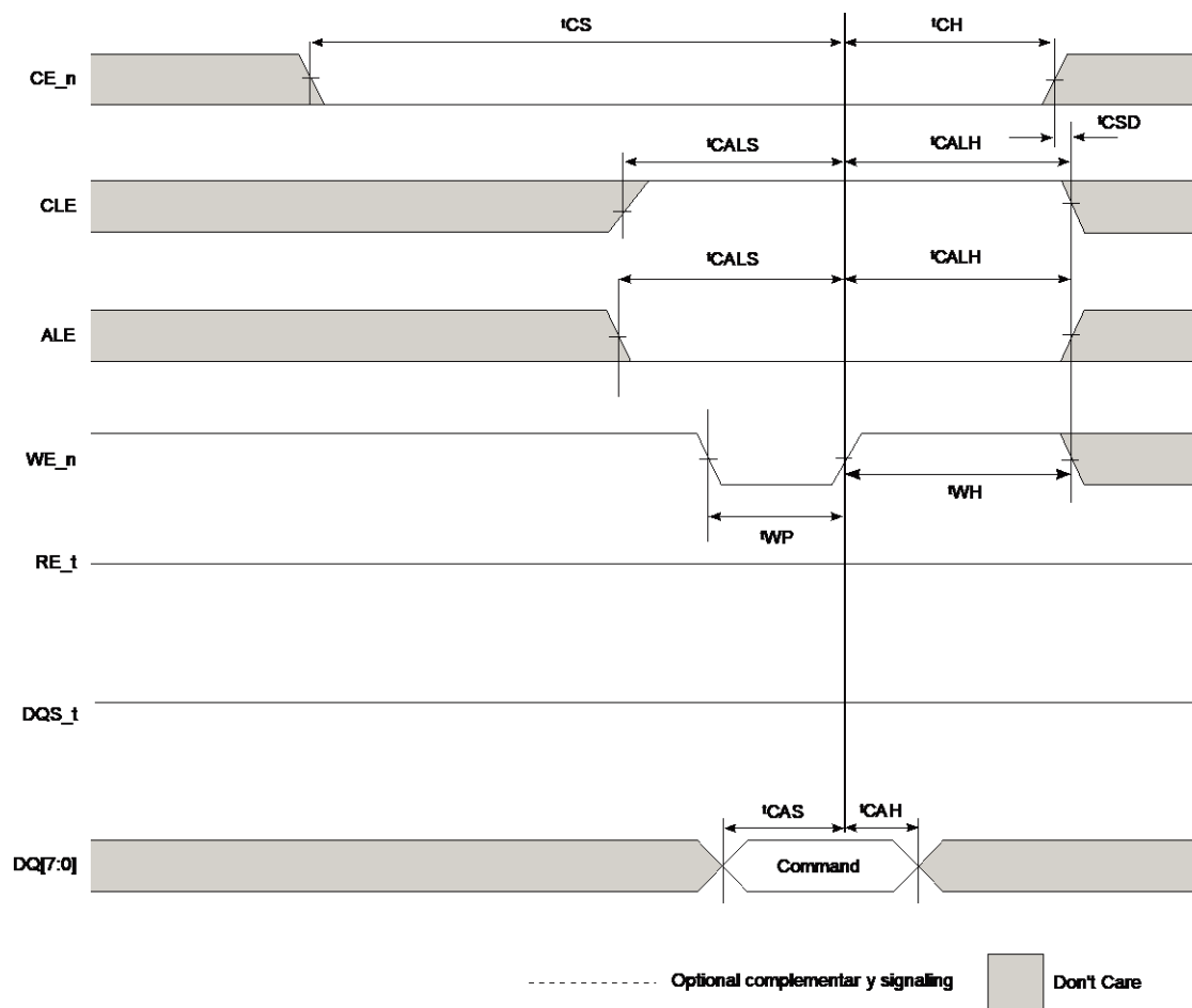
Figure 47. Command cycle
