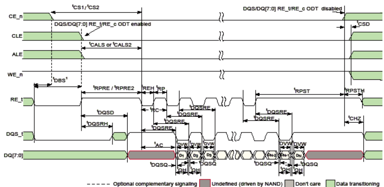
Figure 50. Read cycle
