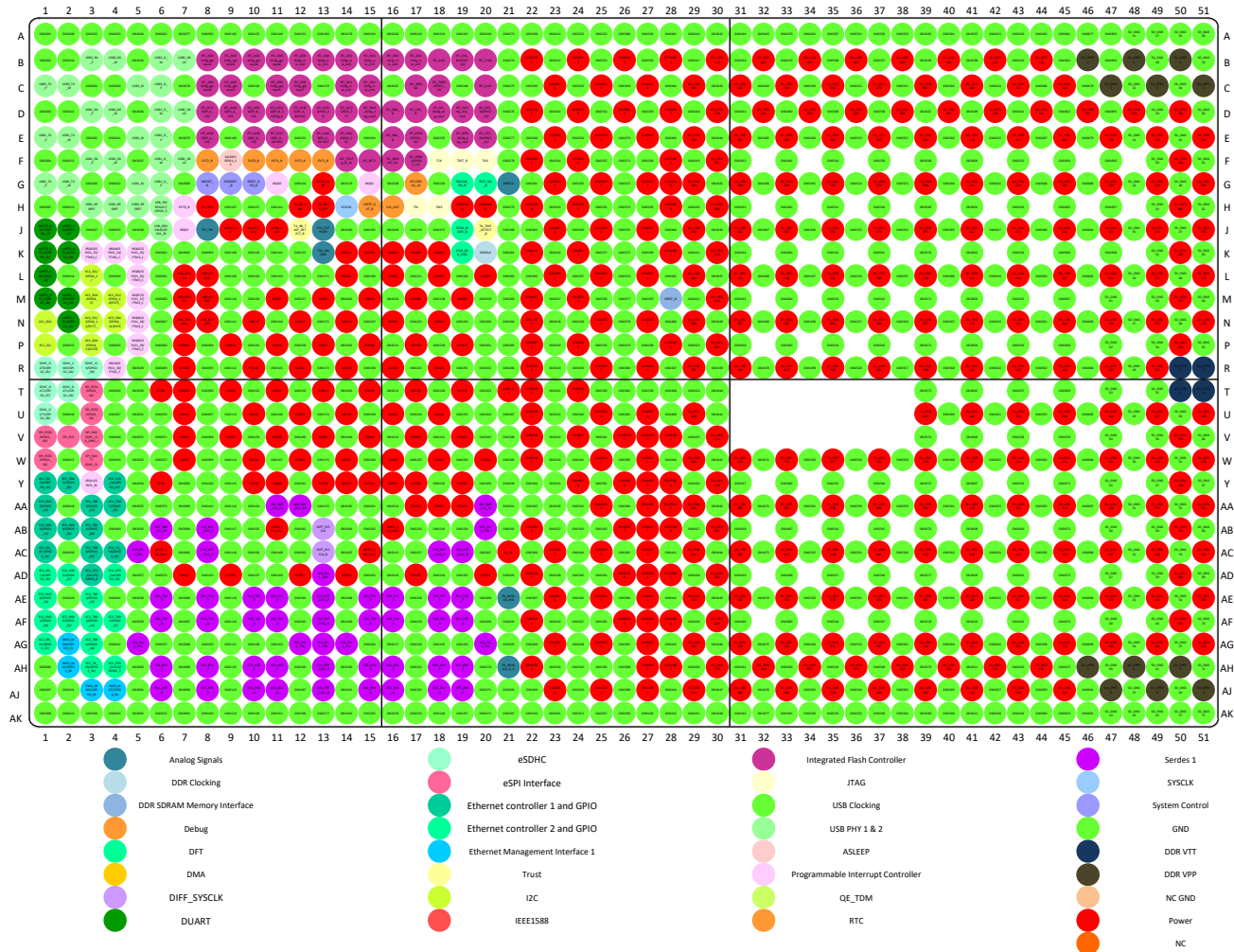
Figure 3. Complete BGA Map for the QLS1046A
