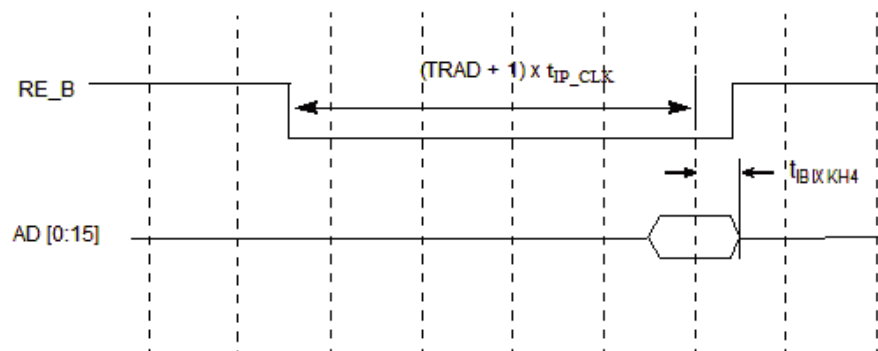
Figure 46. t_{BIXKH4} timings
