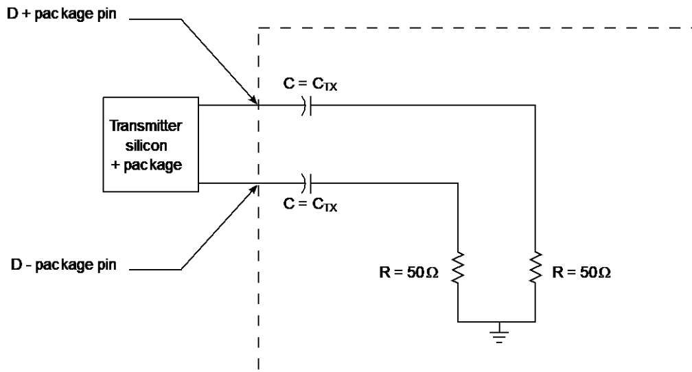
Figure 16. SGMII AC test/measurement load
