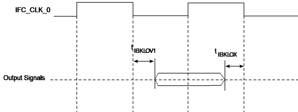
Figure 28. IFC-GPCM, IFC-GASIC signals
