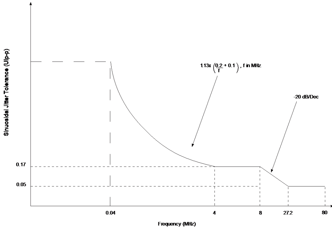
Figure 19. XFI host receiver input sinusoidal jitter tolerance
