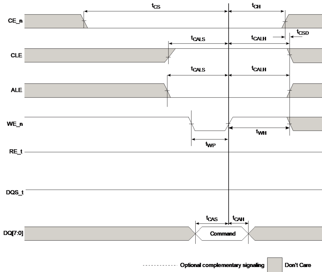
Figure 34. Command cycle
