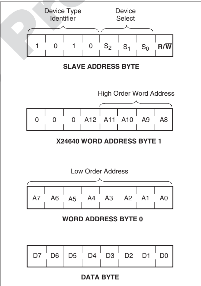
Figure 4. Device Addressing
