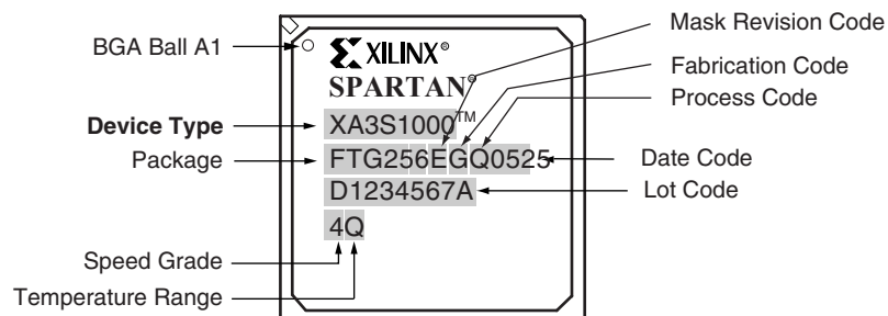
Figure 2: Spartan-3 BGA Package Marking Example for Part Number XA3S1000-4 FTG256Q
