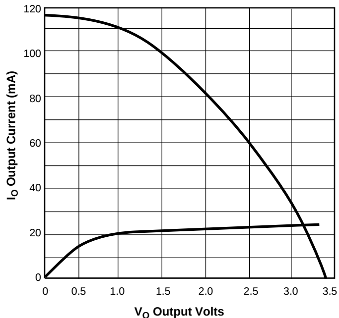
Figure 7: Typical I/O Output for LVC MOS33
