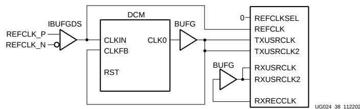
Figure 5: Using RXRECCLK to Generate RXUSRCLK and RXUSRCLK2
