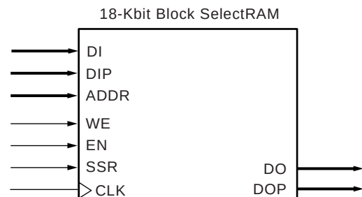
Figure 49: 18 Kb Block SelectRAM+ Memory in Single-Port Mode
