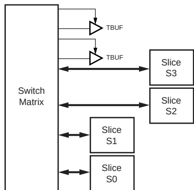
Figure 47: Virtex-II Pro X 3-State Buffers
