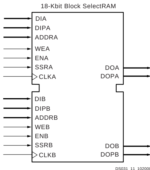
Figure 50: 18 Kb Block SelectRAM+ in Dual-Port Mode
