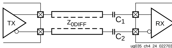
Figure 11: AC-Coupled Serial Link
