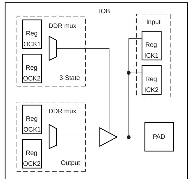
Figure 21: Virtex-II Pro X IOB Block
