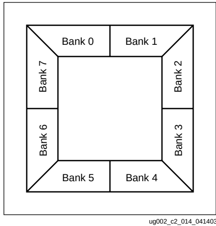
Figure 26: I/O Banks: Wire-Bond Packages (FG) Top View
