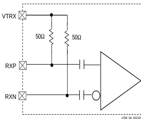
Figure 10: Receive Termination
