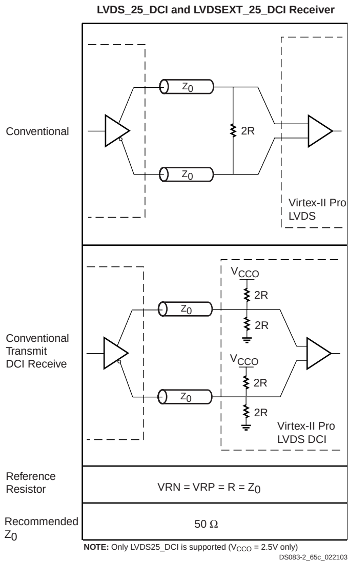
Figure 32: LVDS DCI Usage Examples
