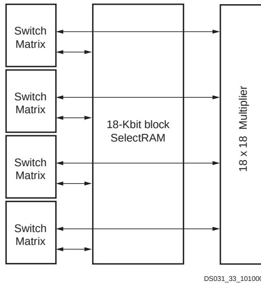
Figure 55: SelectRAM+ and Multiplier Blocks
