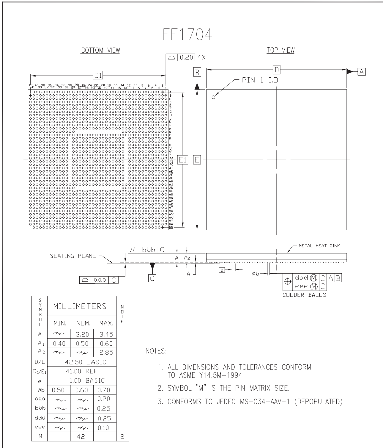
Figure 2: FF1704 Flip-Chip Fine-Pitch BGA Package Specifications
