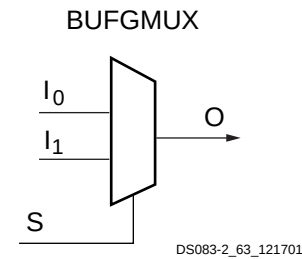
Figure 62: Virtex-II Pro X BUFGMUX Function
