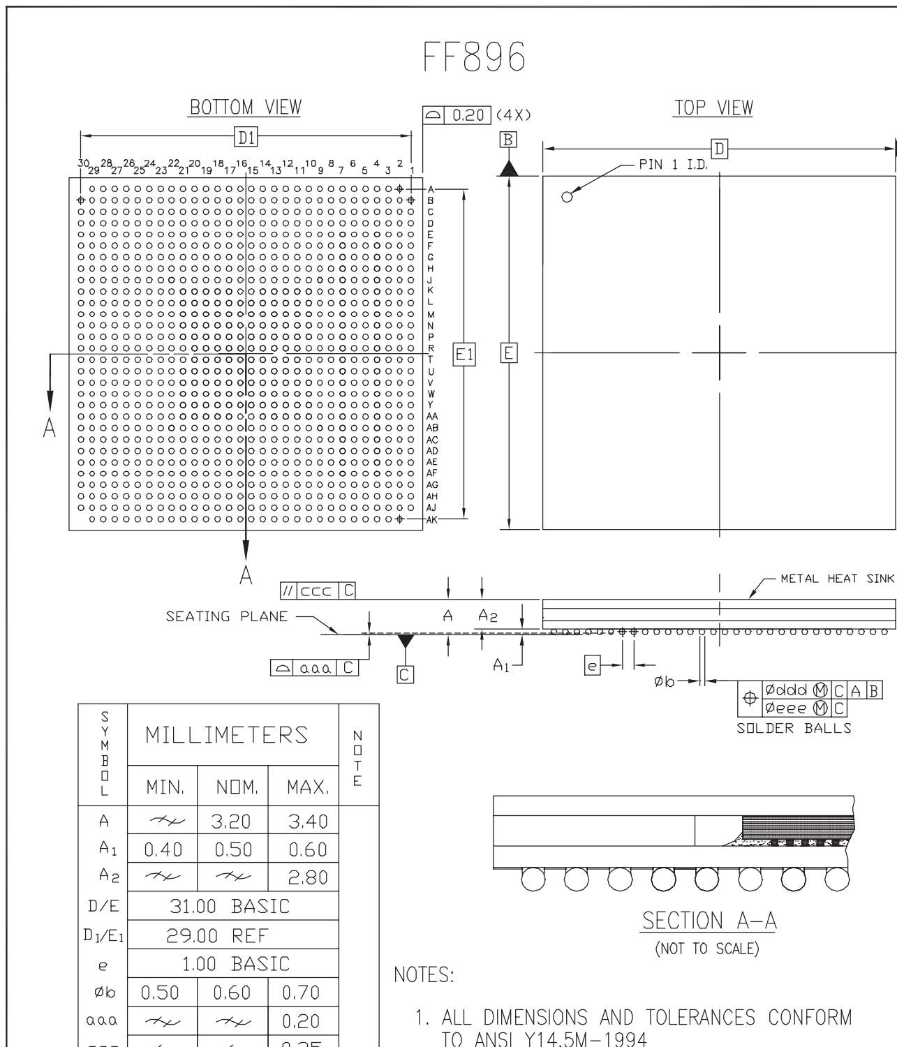
Figure 1: FF896 Flip-Chip Fine-Pitch BGA Package Specifications
