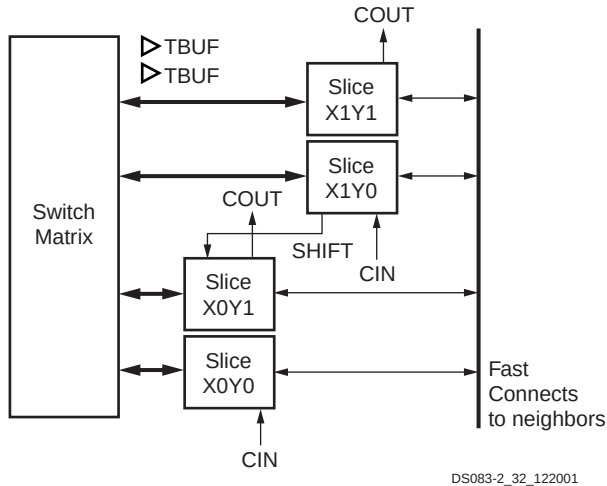
Figure 34: Virtex-II Pro X CLB Element
