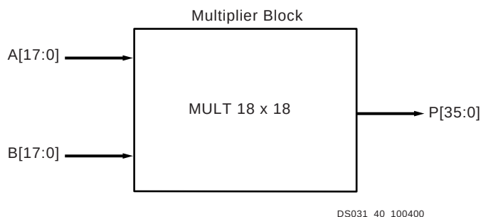
Figure 56: Multiplier Block
