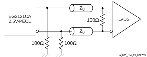
Figure 13: Reference Clock Oscillator Interface up to 400 MHz
