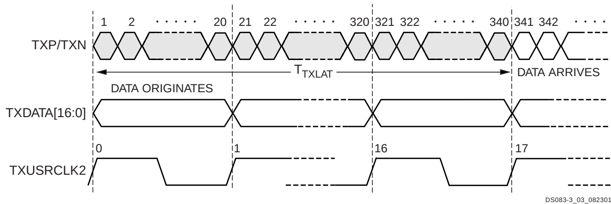
Figure 5: Transmit Latency (Maximum)
