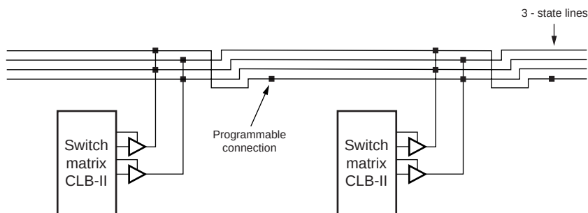
Figure 48: 3-State Buffer Connection to Horizontal Lines
