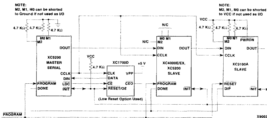
Figure 29: Master/Slave Serial Mode Circuit Diagram
