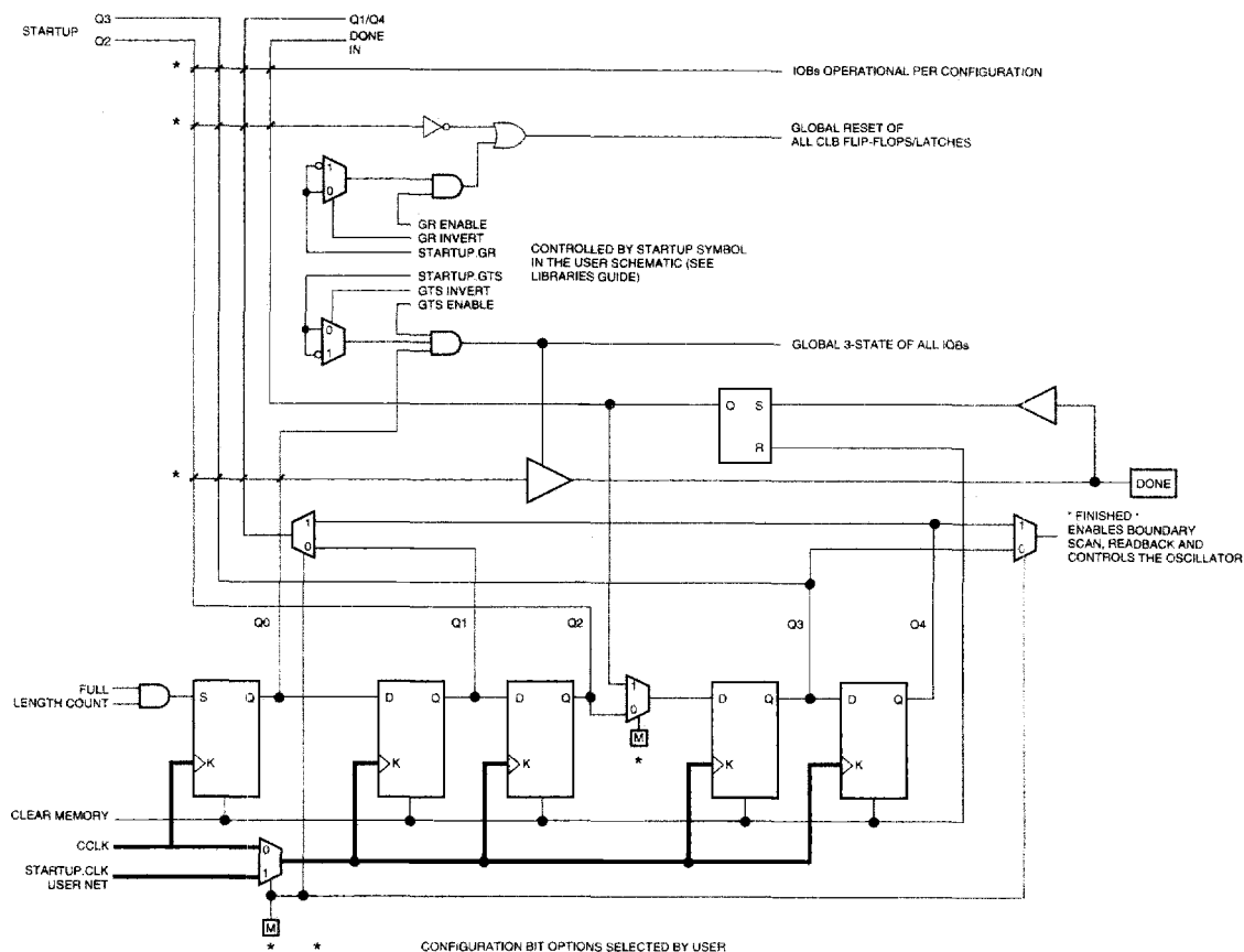
Figure 27: Start-up Logic
