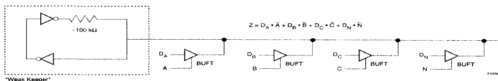
Figure 11: 3-State Buffers Implement a Multiplexer
