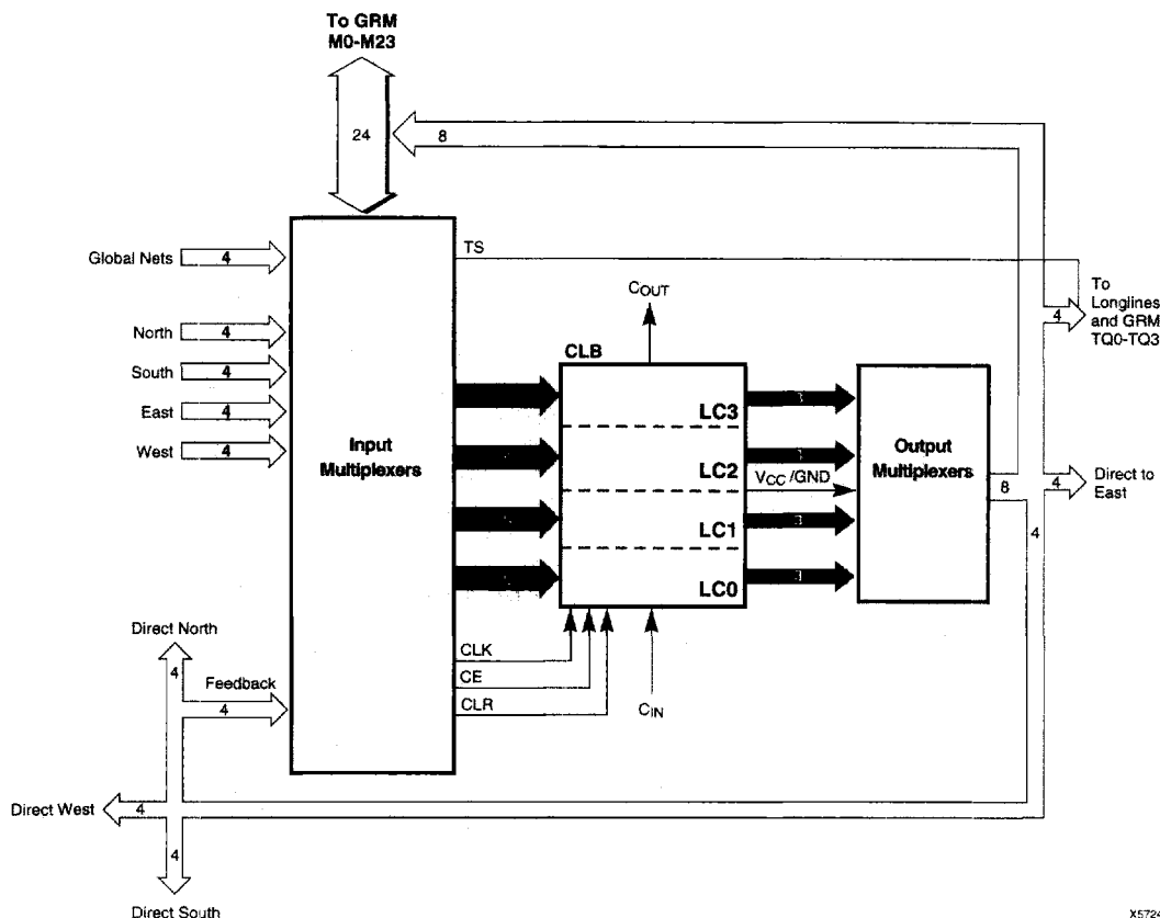
Figure 15: VersaBlock Details
