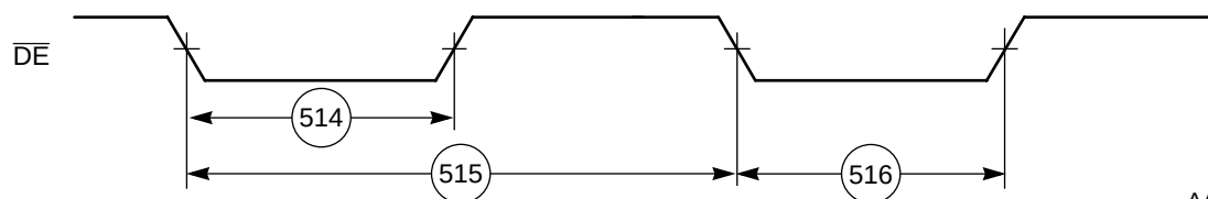
Figure 2-43 OnCE—Debug Request
