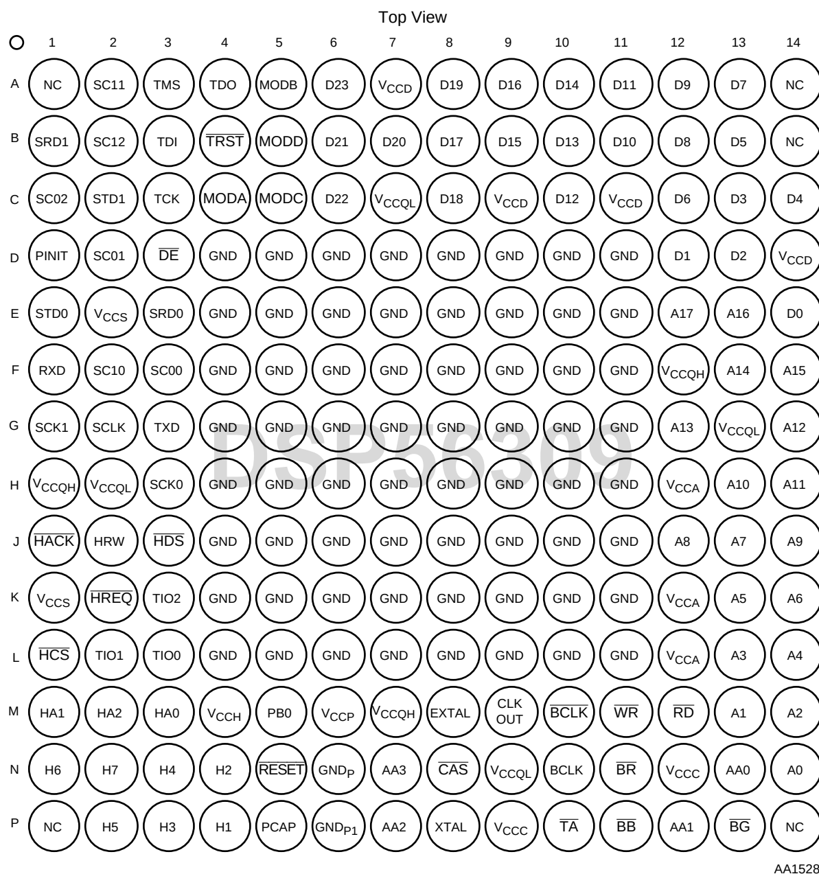
Figure 3-4 DSP56309 Plastic Ball Grid Array (PBGA), Top View
