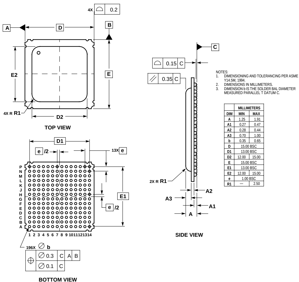
Figure 3-6 DSP56309 Mechanical Information, 196-pin PBGA Package
