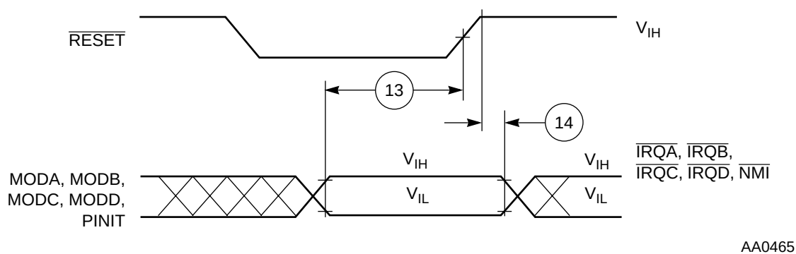
Figure 2-8 Operating Mode Select Timing
