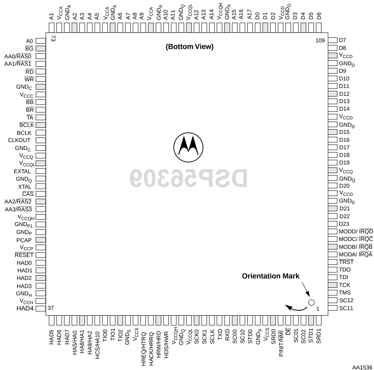
Figure 3-2 DSP56309 Thin Quad Flat Pack (TQFP), Bottom View
