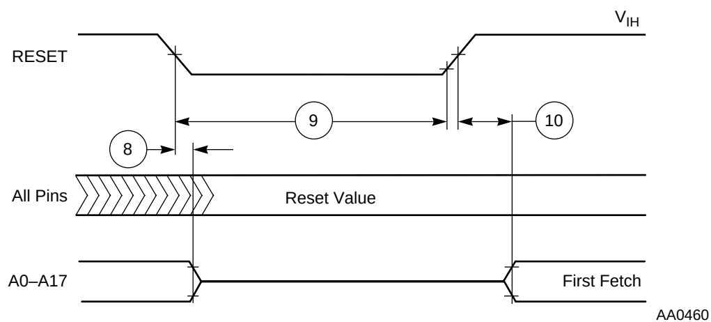
Figure 2-3 Reset Timing
