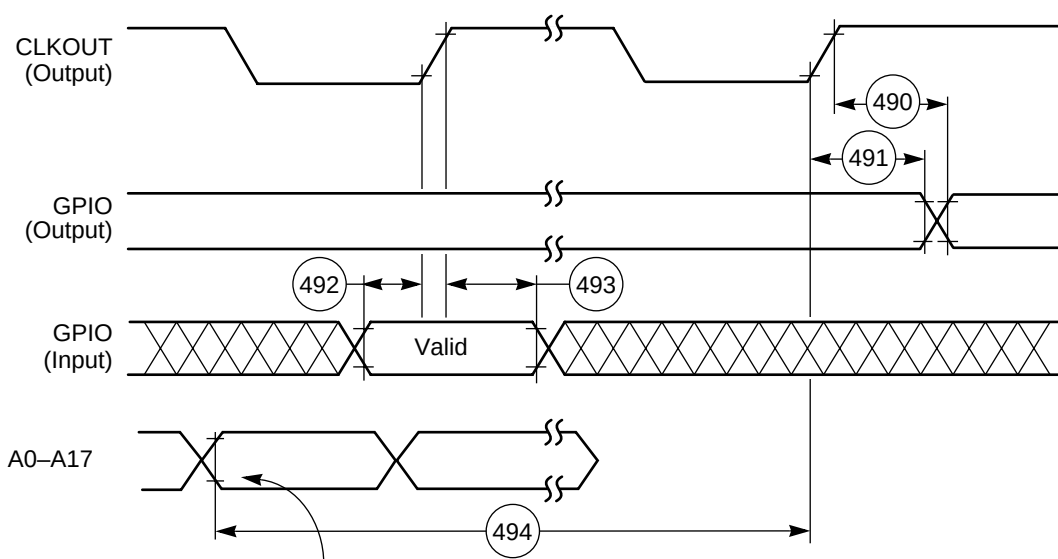
Figure 2-38 GPIO Timing
