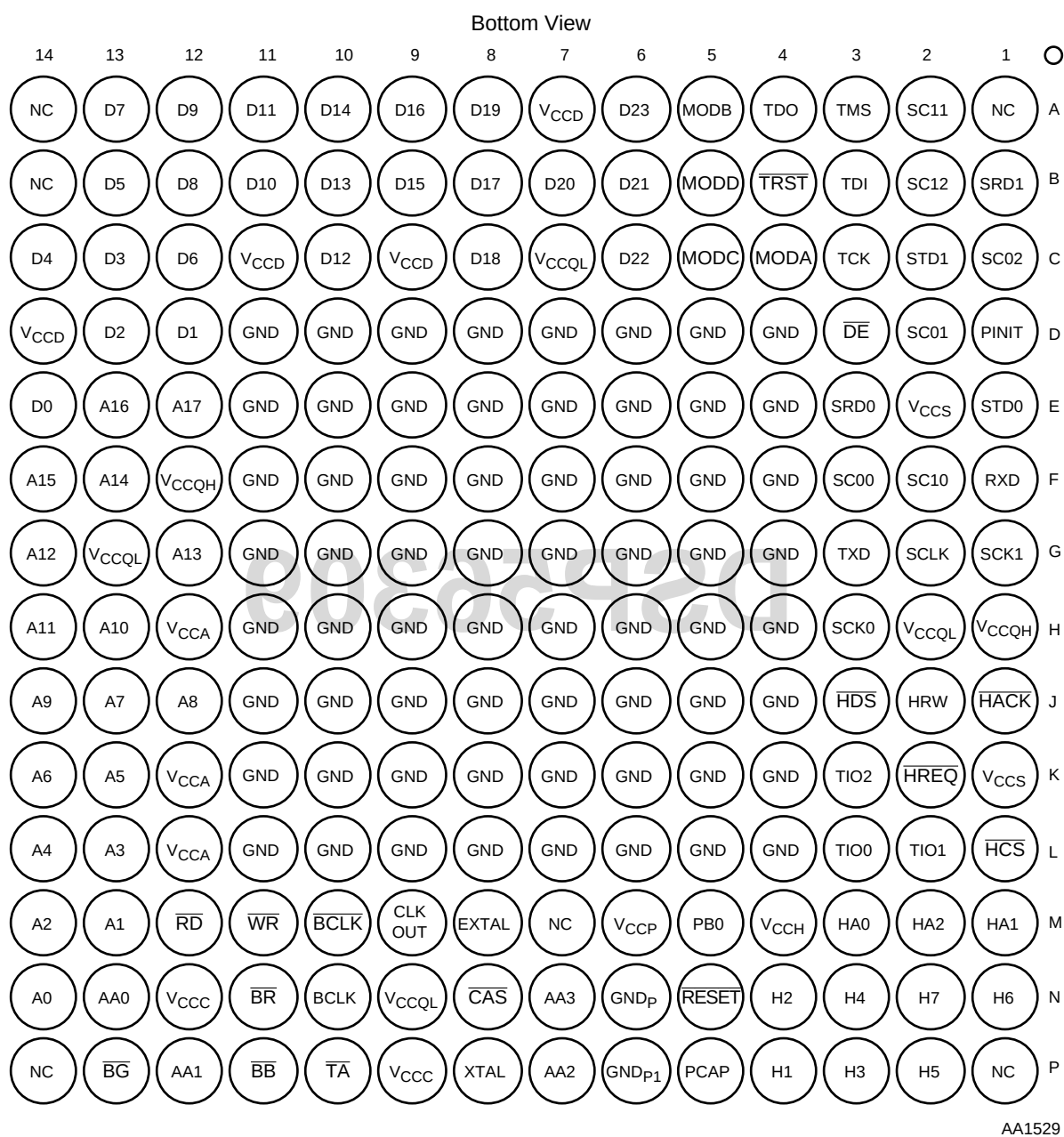
Figure 3-5 DSP56309 Plastic Ball Grid Array (PBGA), Bottom View
