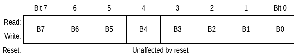
Figure 3-3. Accumulator B (B)
