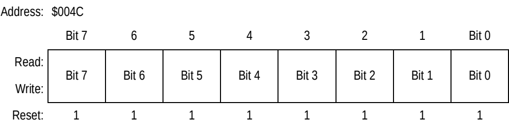
Figure 11-16. PWM Channel Period Register 0 (PWPER0)
