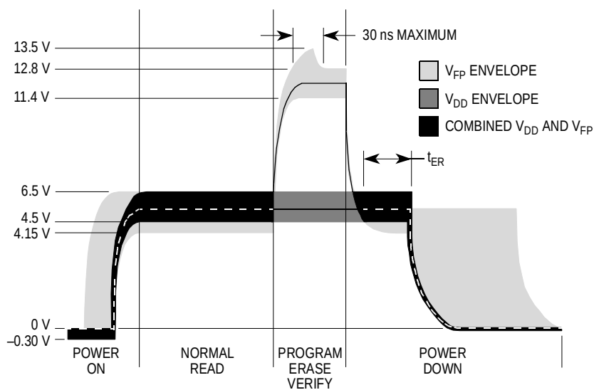
Figure 19-2. V_{FP} Operating Range
