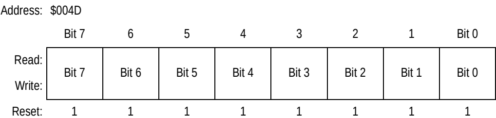
Figure 11-17. PWM Channel Period Register 1 (PWPER1)
