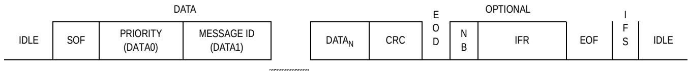
Figure 15-4. J1850 Bus Message Format (VPW)
