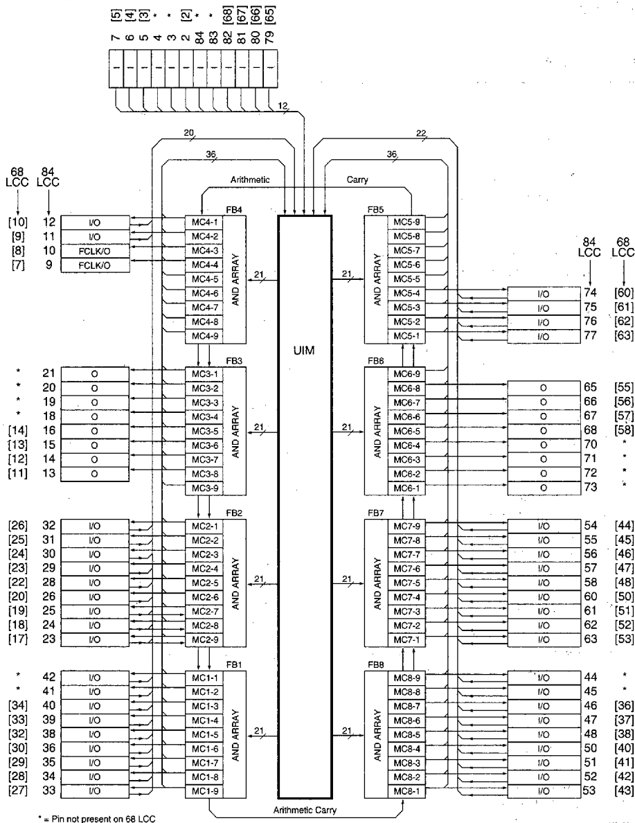
Figure 1: XC7272A Architecture
