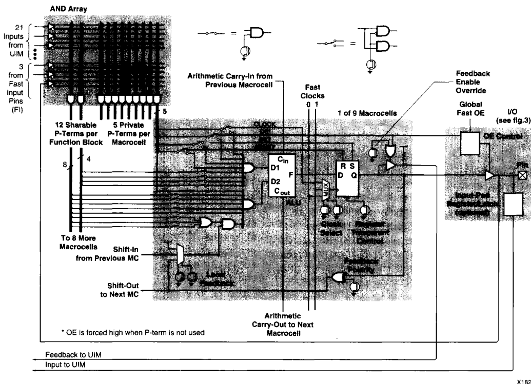
Figure 2: FB and macrocell Schematic
