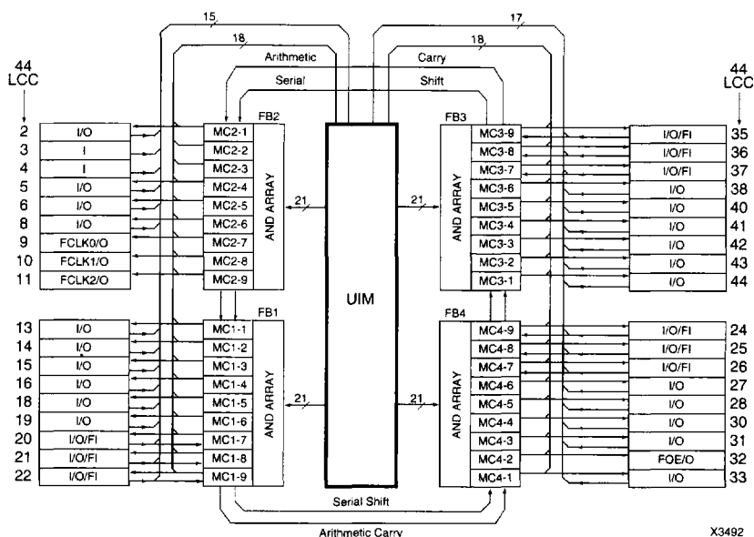
Figure 1: XC7236A Architecture
