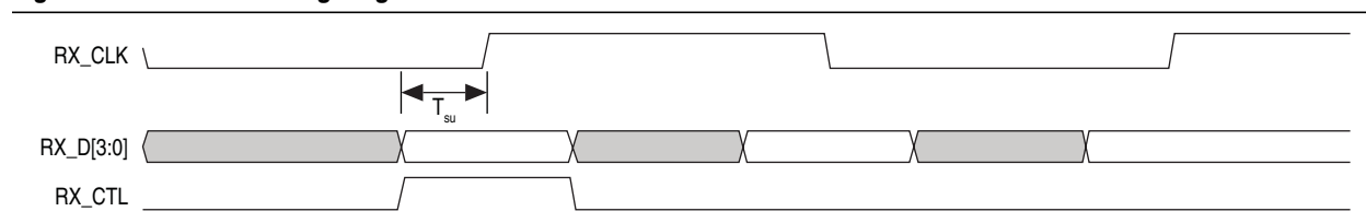
Figure 10. RGMII RX Timing Diagram
