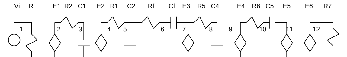
Figure 7. SPICE Model
