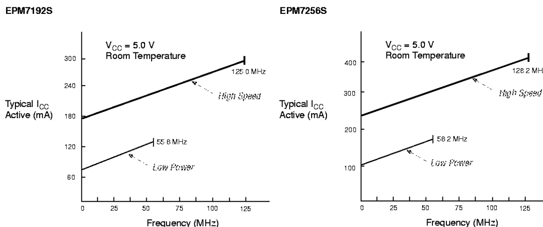
Figure 15. I_{CC} vs. Frequency for MAX 7000S Devices (Part 2 of 2)
