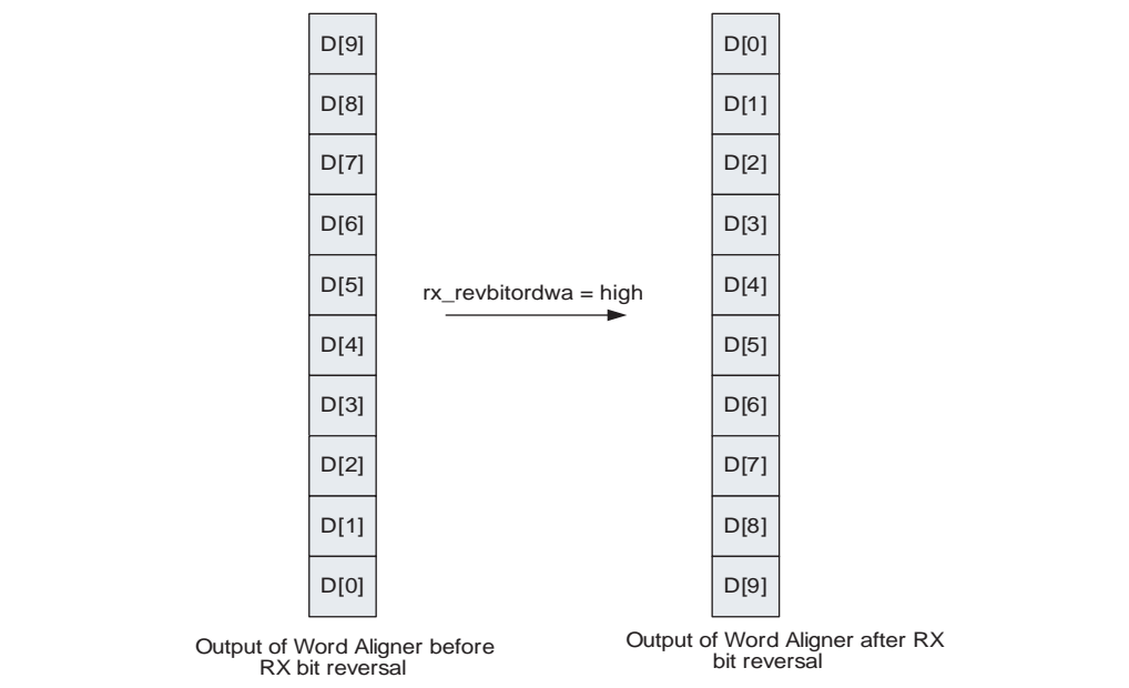
Figure 1-47. 10-Bit Receiver Bit Reversal in Single-Width Mode
