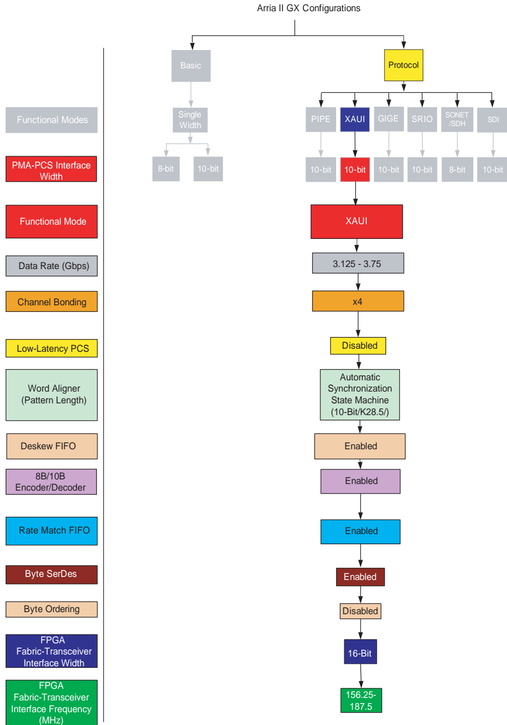
Figure 1-83. Arria II GX XAUI Mode Configuration
