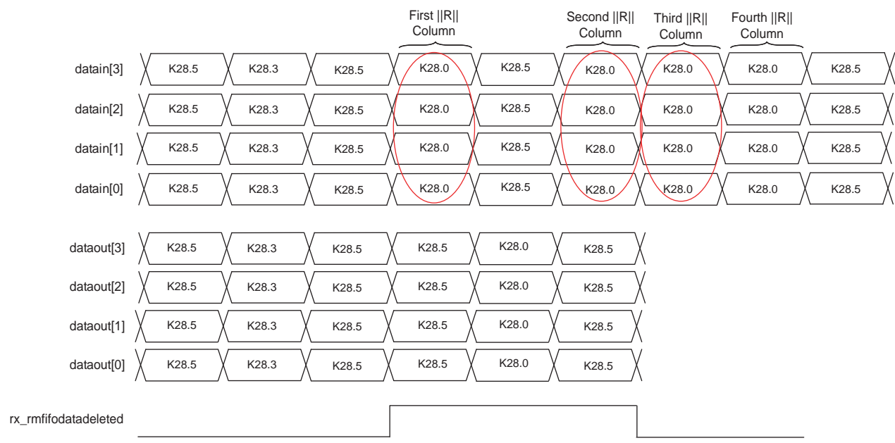
Figure 1-89. Example of Rate Match Deletion in XAUI Mode
