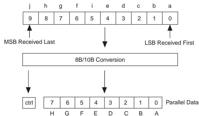
Figure 1-63. 8B/10B Decoder in Single-Width Mode
