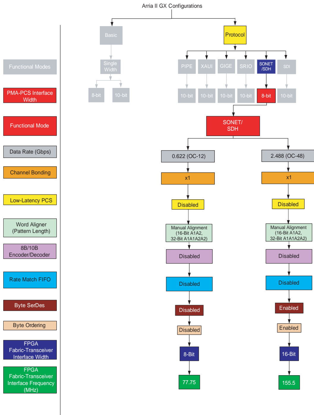
Figure 1-100. SONET/SDH Mode Configurations in Arria II GX Devices
