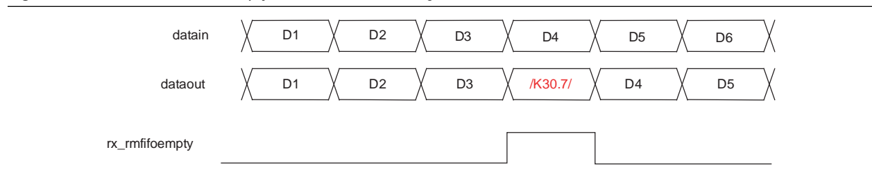
Figure 1-61. Rate Match FIFO Empty Condition in Basic Single-Width Mode
