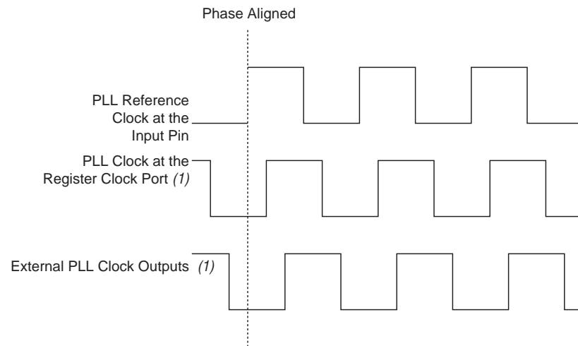
Figure 5-17. Phase Relationship Between PLL Clocks in No Compensation Mode
