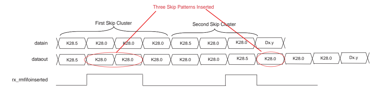
Figure 1-59. Example of Rate Match Insertion in Basic Single-Width Mode
