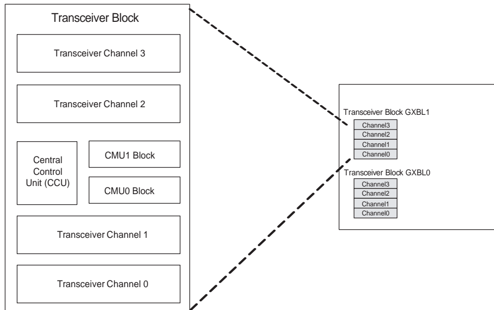
Figure 1-5. Top-Level View of a Transceiver Block
