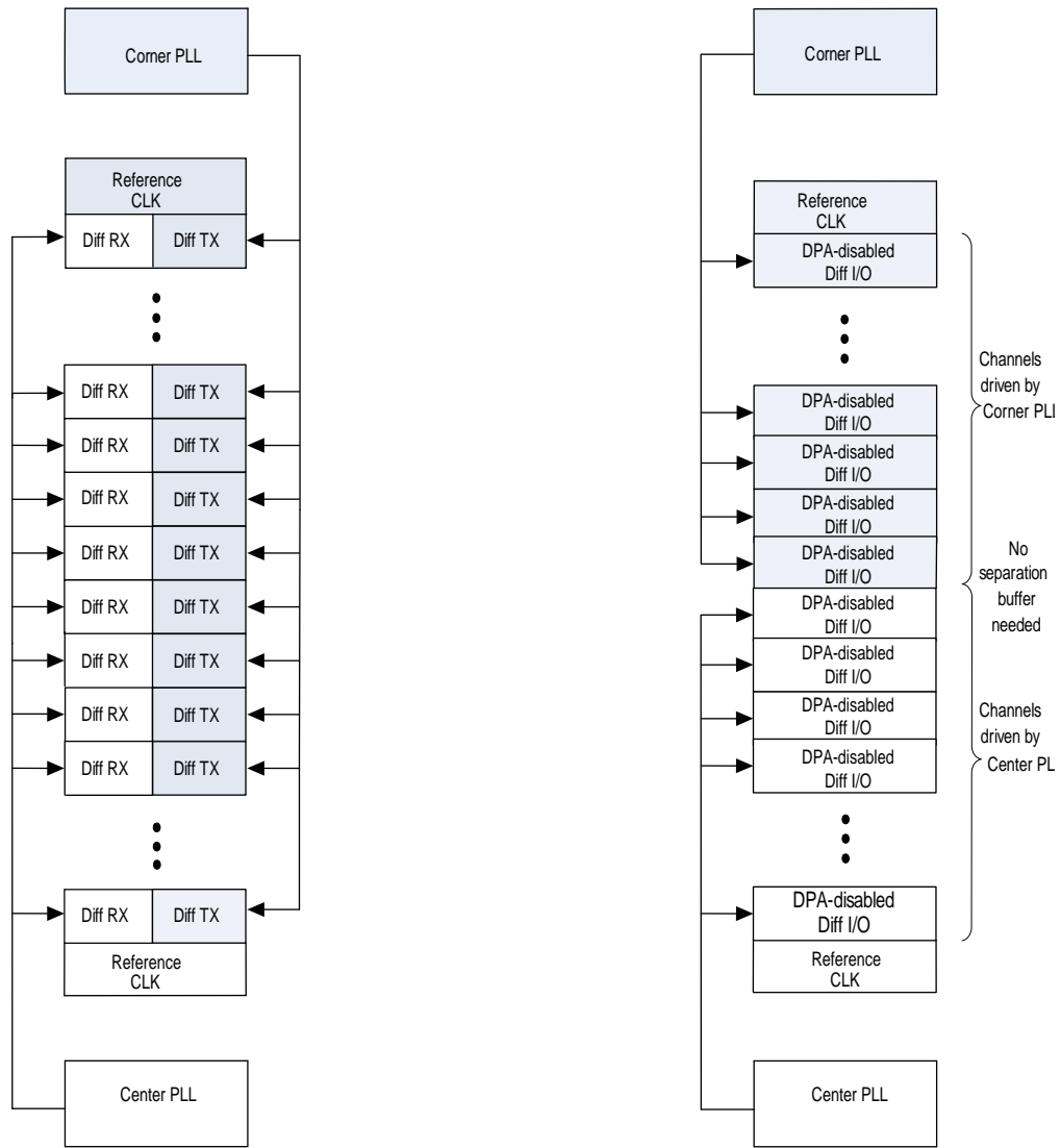
Figure 8-25. Corner and Center PLLs Driving DPA-Disabled Differential I/Os in the Same Bank
