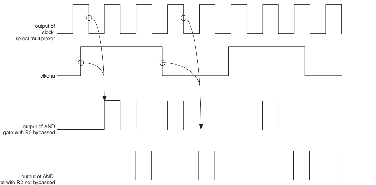
Figure 5-11. clkena Signals
