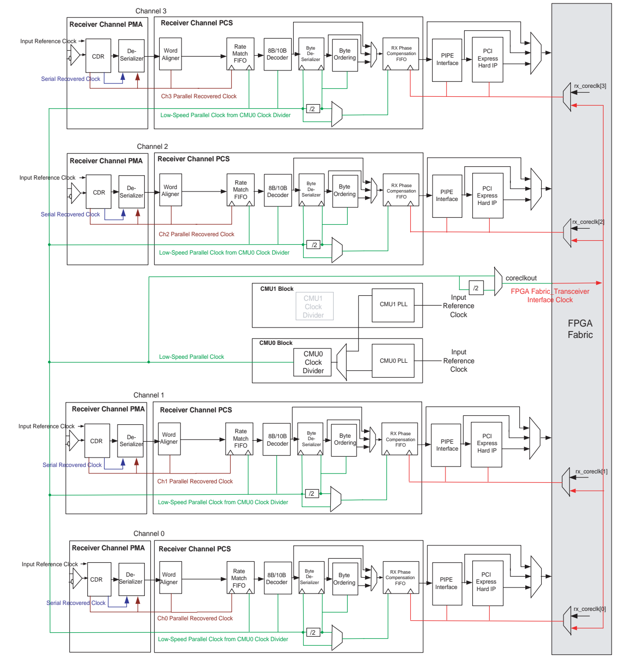
Figure 2-14. Receiver Datapath Clocking in x4 Bonded Channel Configurations without Deskew FIFO
