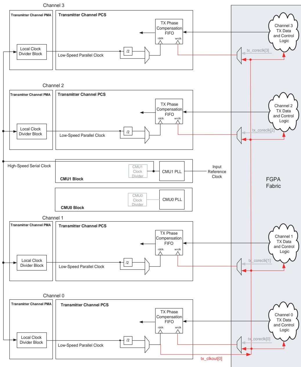
Figure 2-16. Four Identical Channels in a Transceiver Block for Example 1
