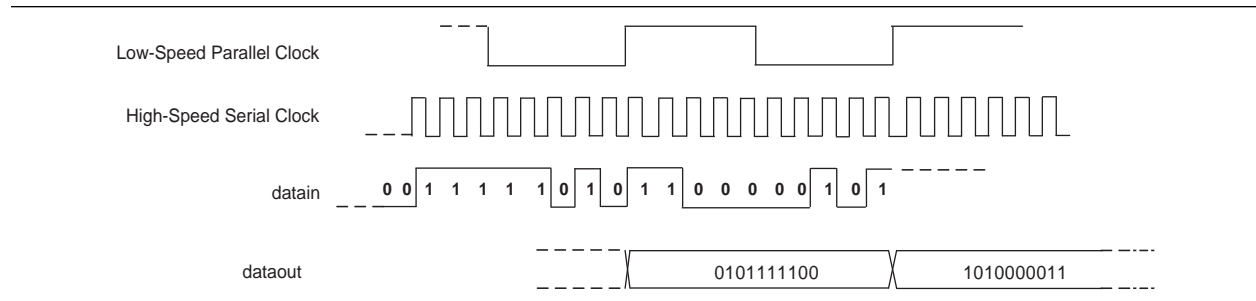
Figure 1-41. 10-Bit Deserializer Bit Order in Single-Width Mode
