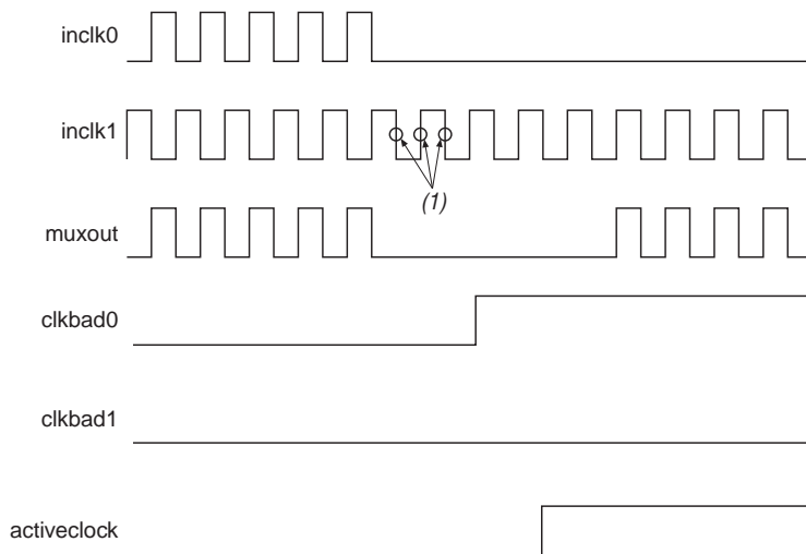
Figure 5-23. Automatic Switchover Upon Loss of Clock Detection
