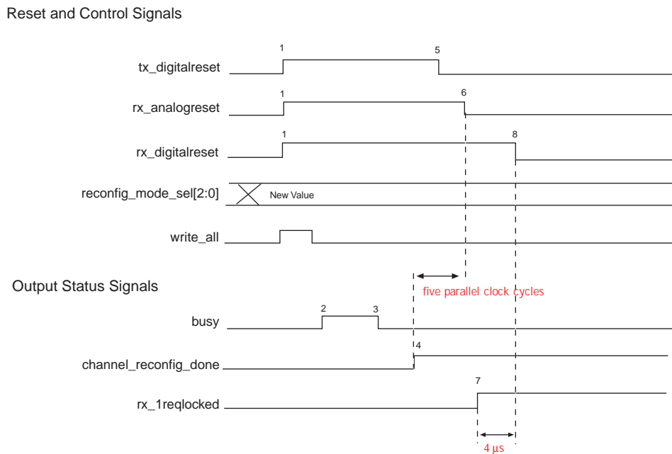
Figure 4-12. Reset Sequence in Basic 1 Mode with Receiver CDR in Automatic Lock Mode (Channel and TX PLL select/reconfig Option)
