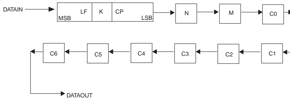
Figure 5–29. Scan-Chain Order of PLL Components for Arria II GX PLLs
