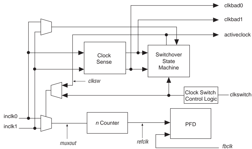
Figure 5–22. Automatic Clock Switchover Circuit Block Diagram
