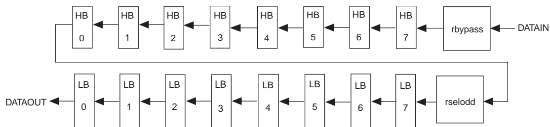
Figure 5–30. Scan-Chain Bit-Order Sequence for Post-Scale Counters in Arria II GX PLLs
