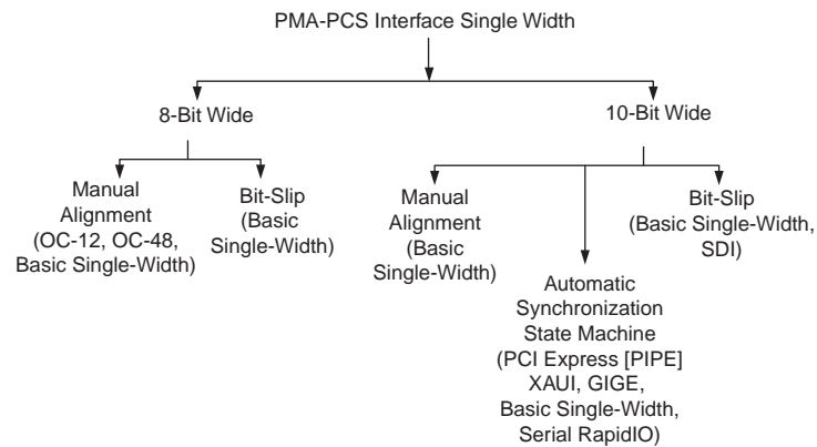
Figure 1-42. Word Aligner in All Supported Configurations
