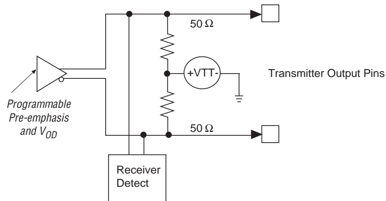
Figure 1-26. Transmitter Output Buffer
