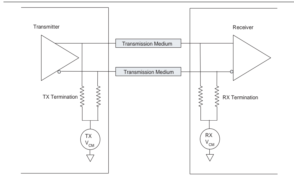
Figure 1-32. DC-Coupled Link
