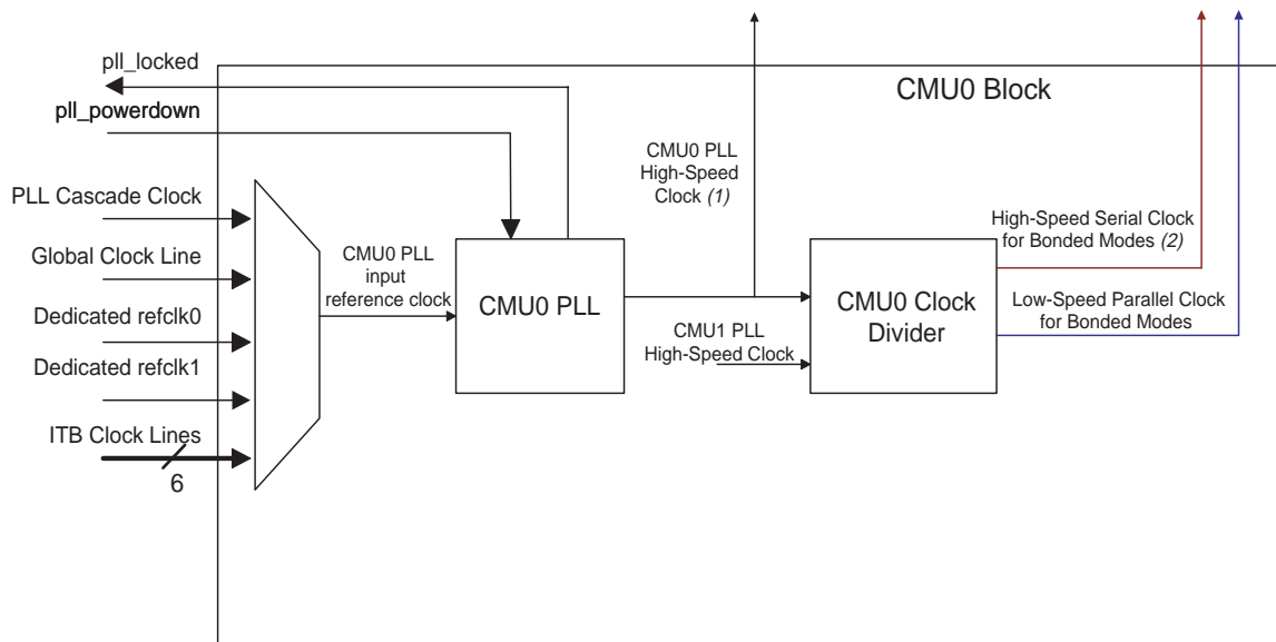
Figure 1-8. Diagram of CMU0 Block
