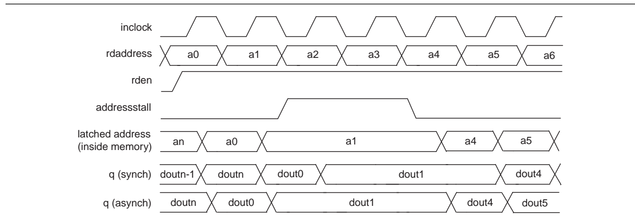
Figure 3-3. Arria II GX Address Clock Enable during Read Cycle Waveform
