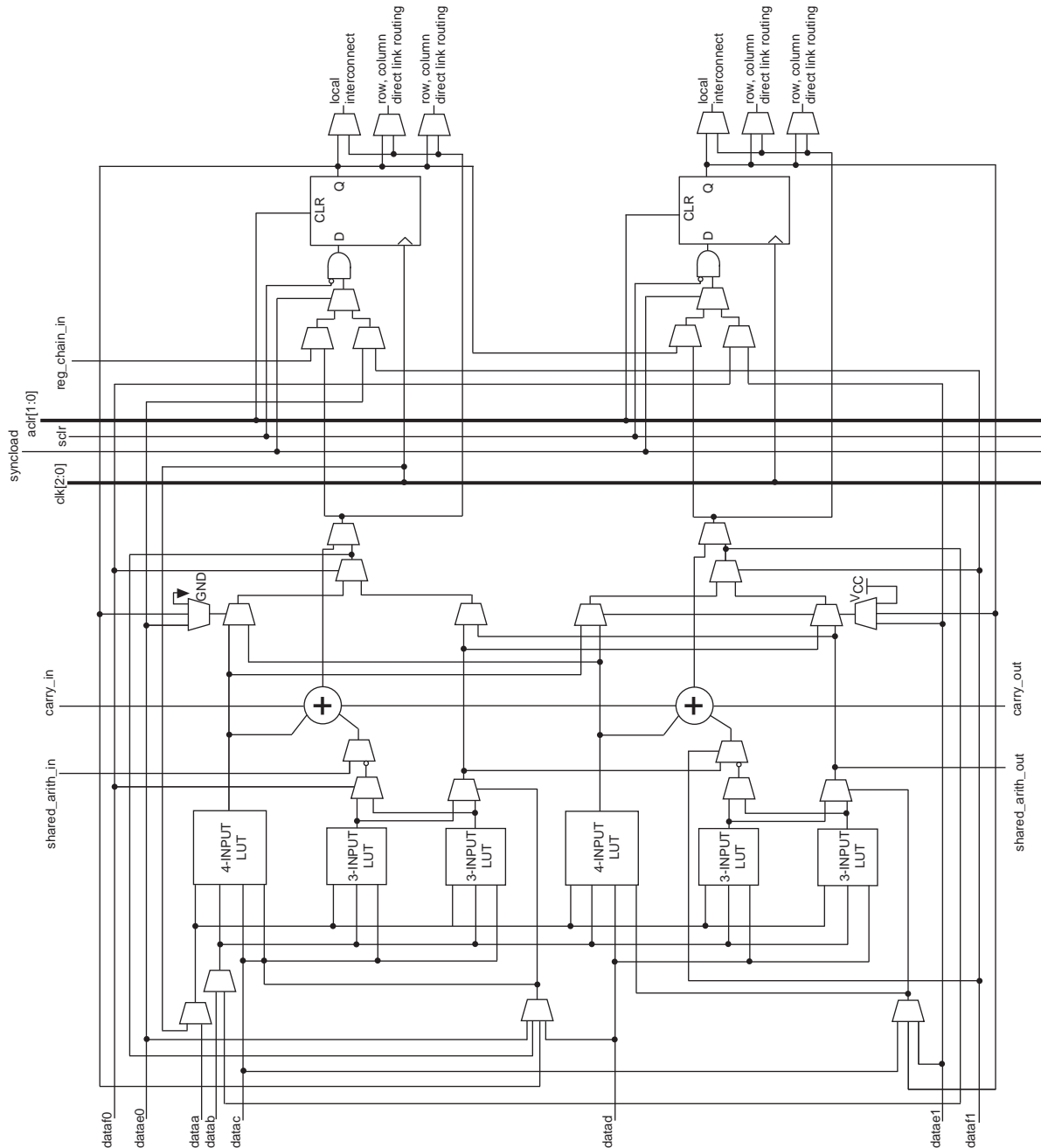
Figure 2-6. Arria II GX ALM Details
