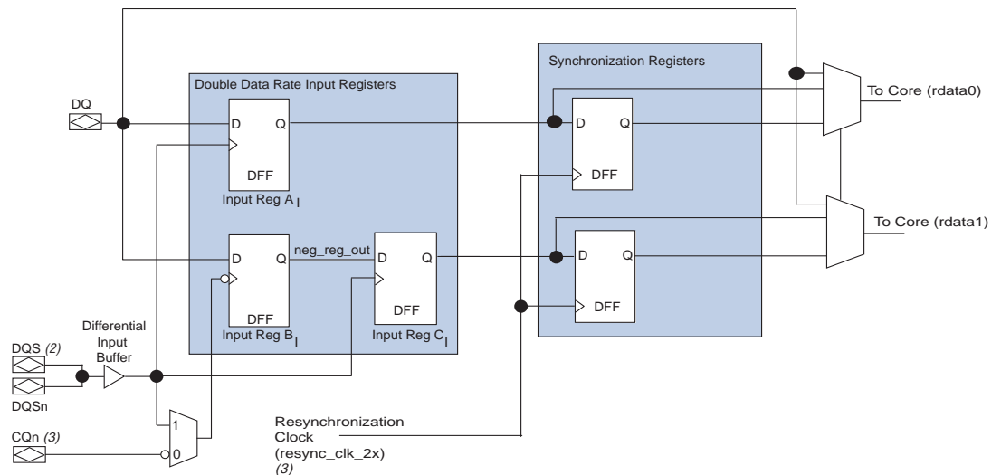
Figure 7-17. Arria II GX IOE Input Registers (Note 1)
