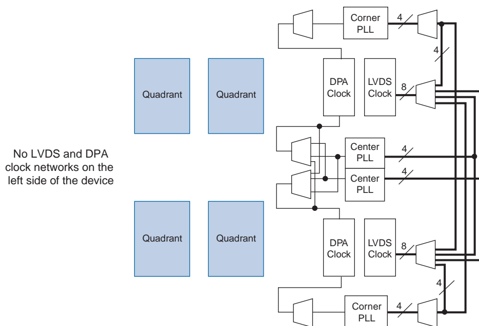
Figure 8-17. LVDS and DPA Clock Networks in the Arria II GX Family with Center PLLs
