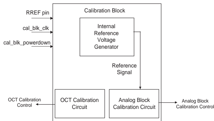
Figure 1-116. Input Signals to the Calibration Blocks (Note 1)
