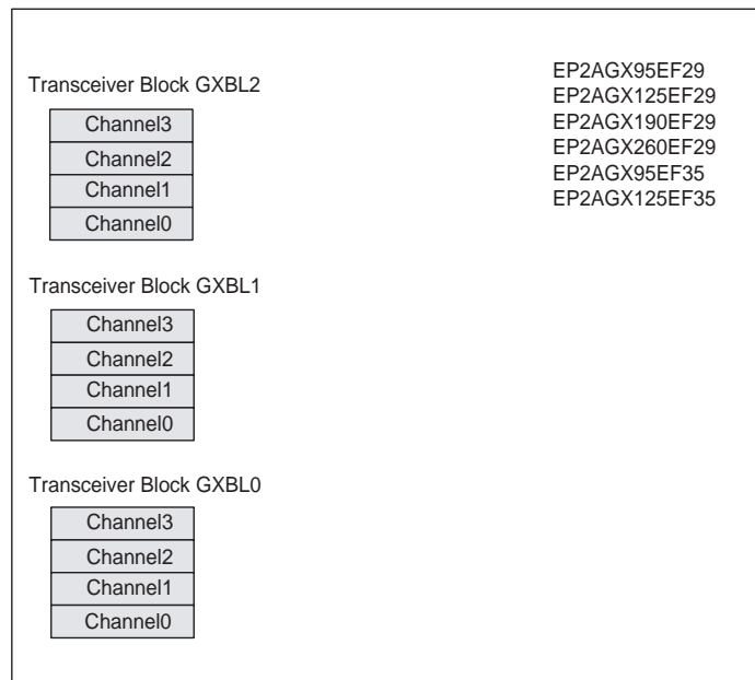
Figure 1-3. Arria II GX Devices with Twelve Transceiver Channels
