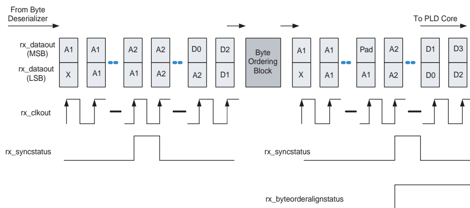
Figure 1-103. OC-48 Byte Ordering in Automatic Mode
