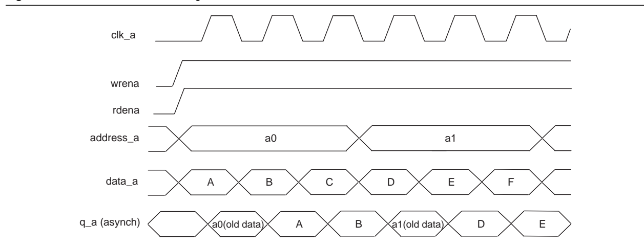
Figure 3-15. Same Port Read-During-Write: Old Data Mode
