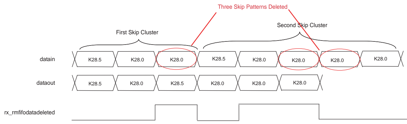
Figure 1-58. Example of Rate Match Deletion in Basic Single-Width Mode
