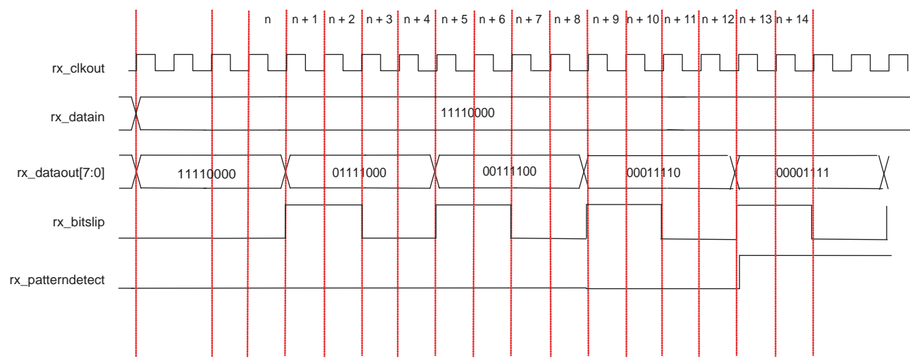
Figure 1-44. Example of Word Aligner Configured in Bit-Slip Mode
