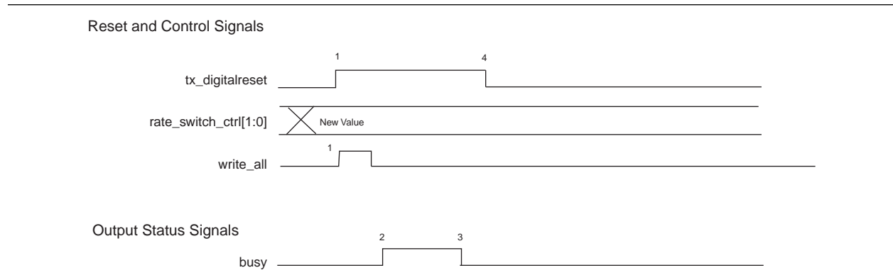
Figure 4-11. Reset Sequence in Basic 1 Mode with the Receiver CDR in Automatic Lock Mode (TX Option)
