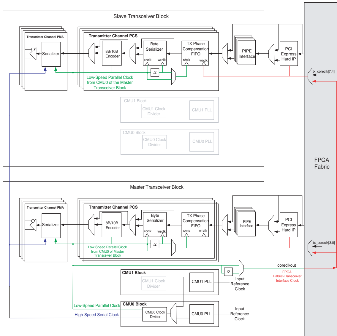
Figure 2-7. Transmitter Datapath Clocking in a ×8 Bonded Configuration
