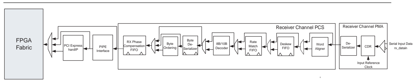
Figure 1-29. Receiver Channel Datapath
