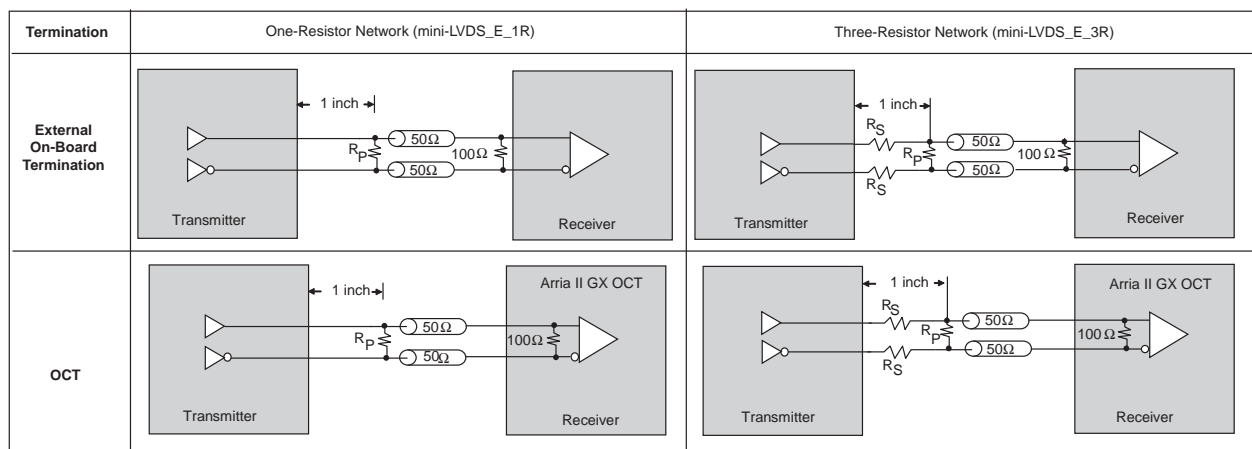
Figure 6-14. Arria II GX mini-LVDS I/O Standard Termination ( Note 1 )
