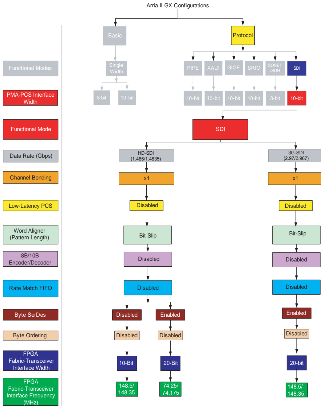
Figure 1-104. SDI Mode
