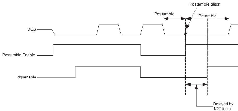
Figure 7-16. Avoiding Glitch on a Non-Consecutive Read Burst Waveform
