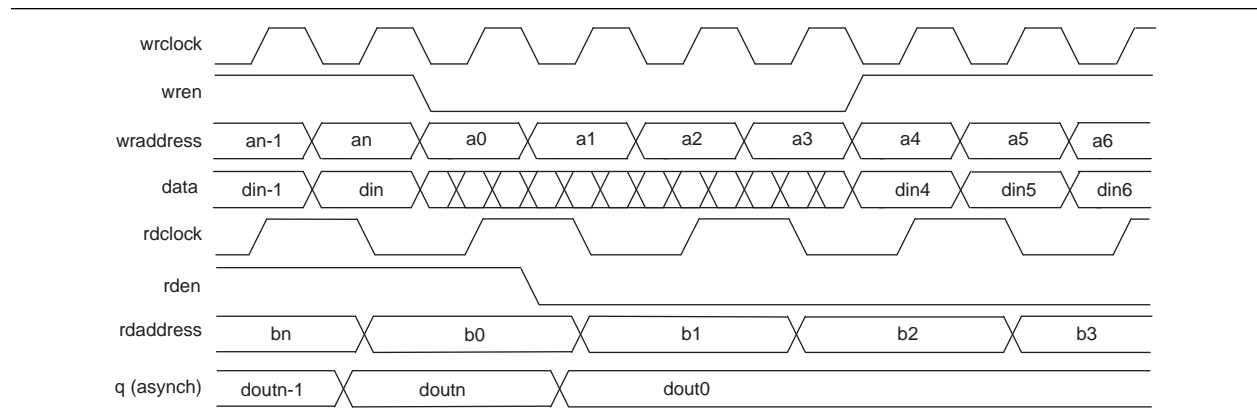
Figure 3-9. Arria II GX Simple Dual-Port Timing Waveforms
