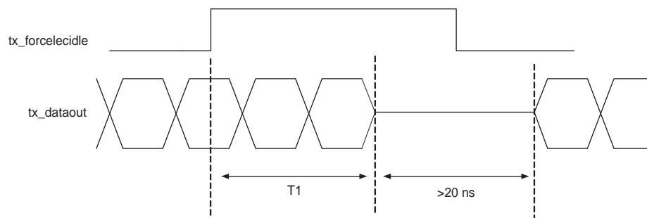
Figure 1-74. Transmitter Buffer Electrical Idle State
