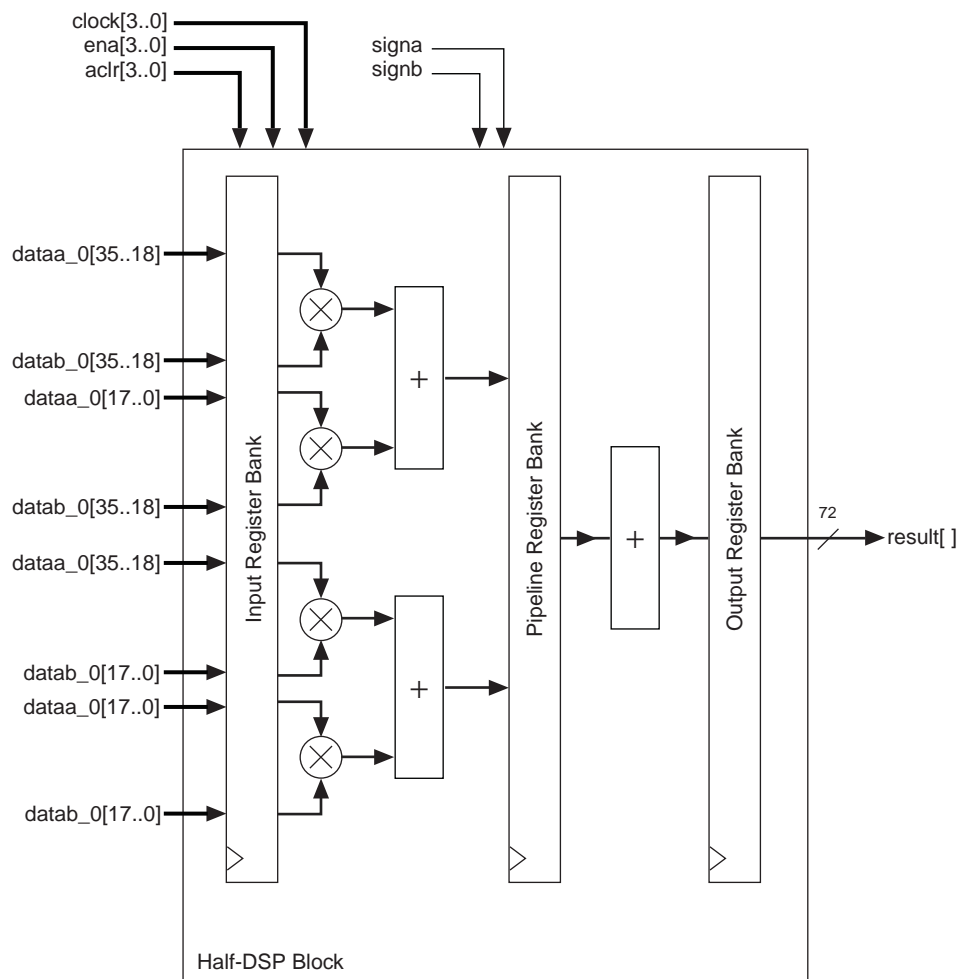
Figure 4-9. 36-Bit Independent Multiplier Mode Shown for Half-DSP Block
