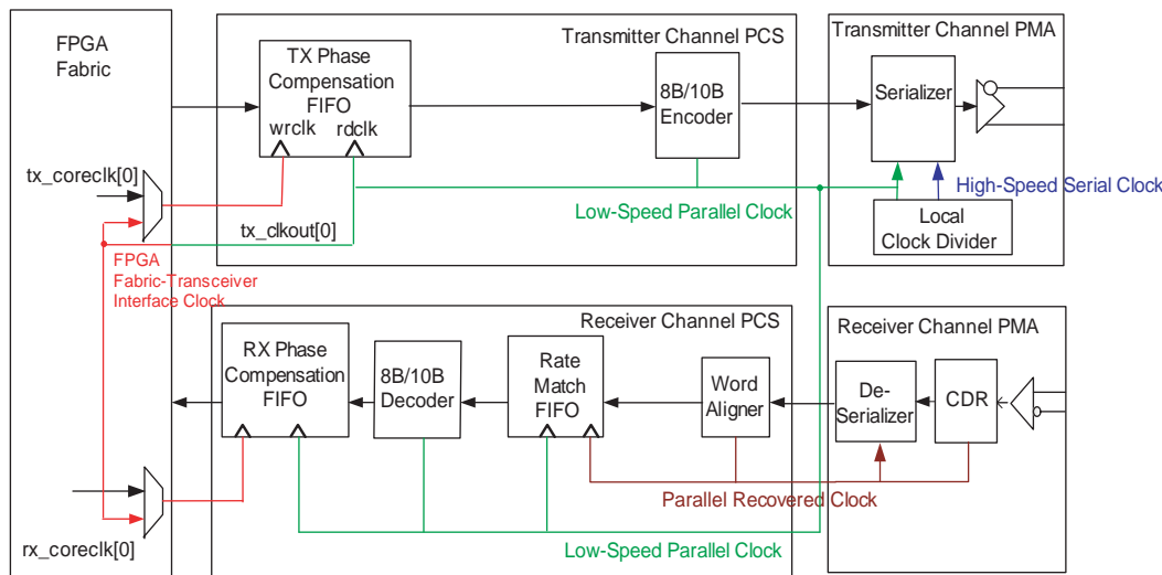
Figure 1-93. GIGE Mode Datapath
