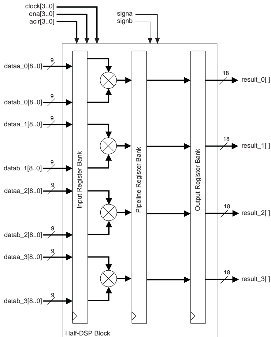
Figure 4-8. 9-Bit Independent Multiplier Mode Shown for Half-Block
