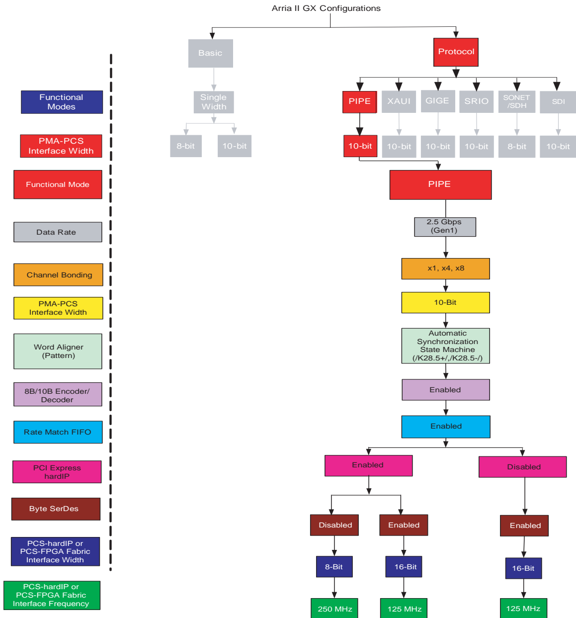
Figure 1-72. Arria II GX Transceivers in PCI Express (PIPE) Functional Mode
