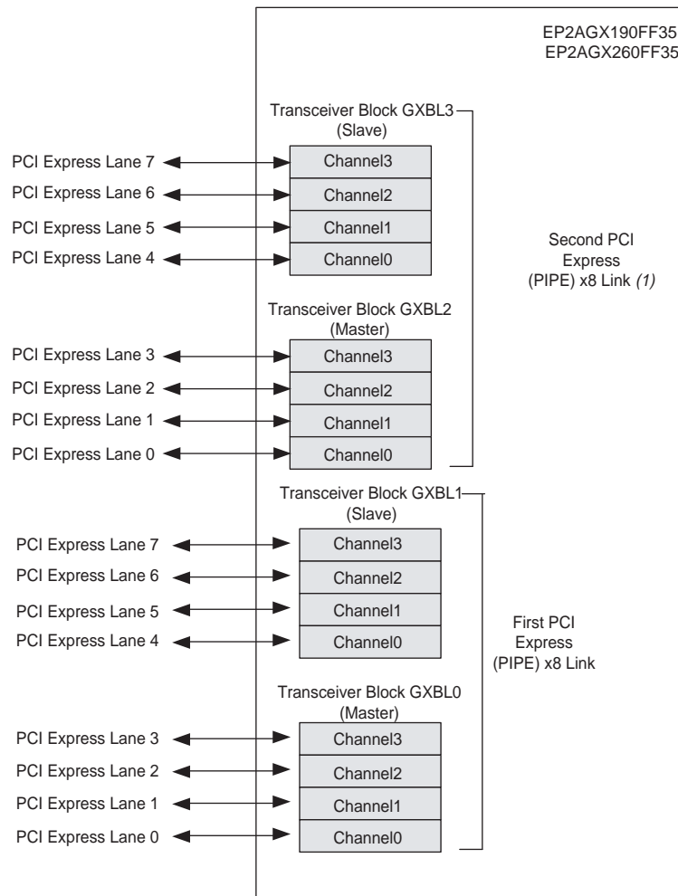
Figure 2-10. Two PCI Express (PIPE) \times 8 Link in Four Transceiver Block Devices
