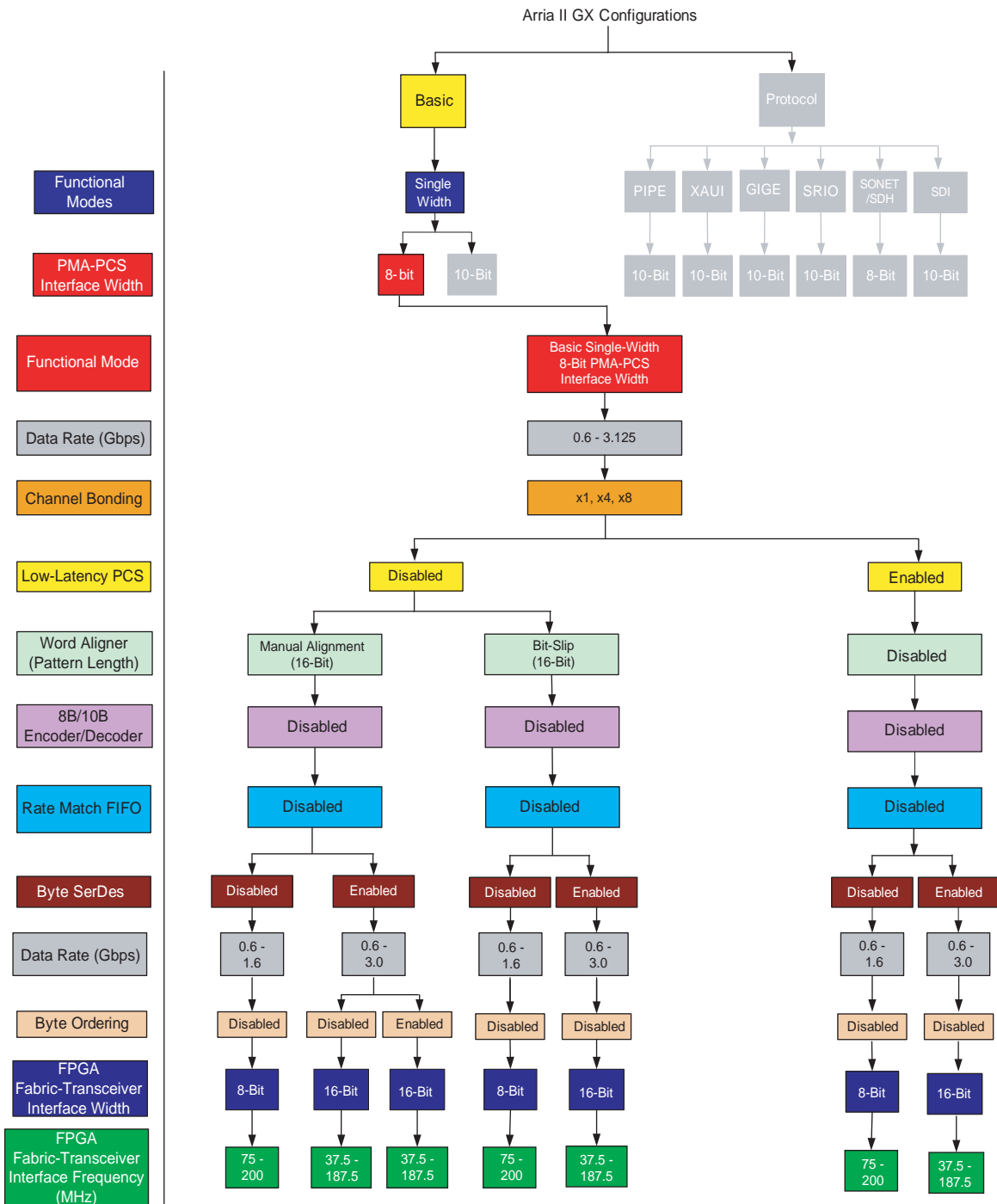
Figure 1-69. Transceiver Configurations in Basic Single-Width Mode with an 8-Bit Wide PMA-PCS Interface
