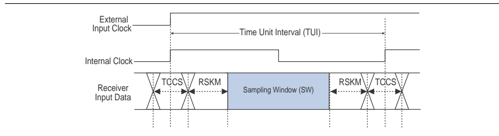
Figure 8–20. Differential High-Speed Timing Diagram and Timing Budget for Non-DPA
