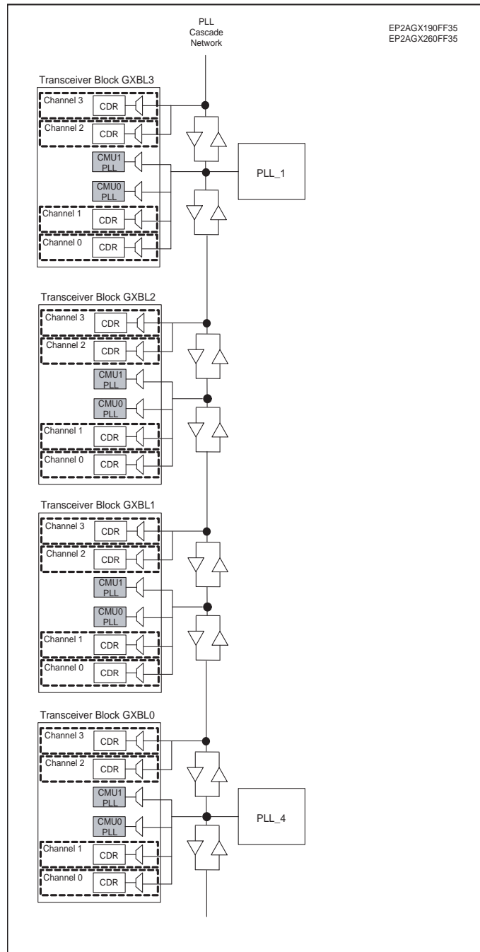
Figure 2-32. FPGA Fabric PLLs-Transceiver PLLs Cascading Option Allowed in the EP2AGX190FF35 and EP2AGX260FF35 Devices
