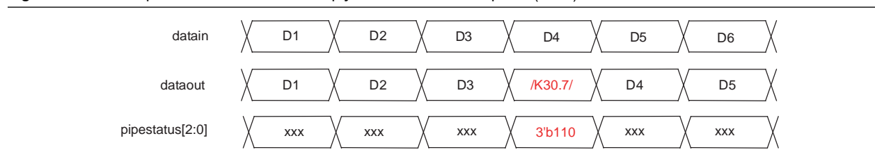
Figure 1–53. Example of Rate Match FIFO Empty Condition in PCI Express (PIPE) Mode
