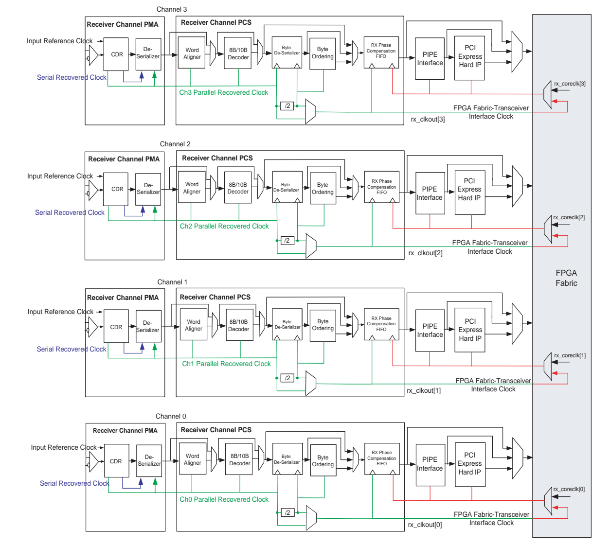
Figure 2-11. Receiver Datapath Clocking in Non-Bonded Configurations without Rate Matcher
