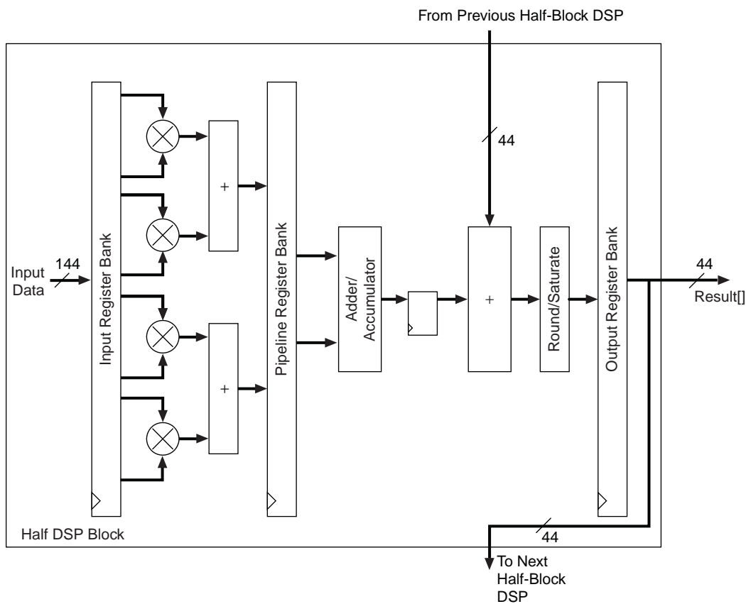
Figure 4-3. Output Cascading Feature for FIR Structures
