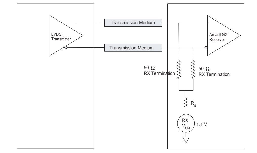
Figure 1–36. LVDS Transmitter to Arria II GX Receiver (PCML) DC-Coupled Link
