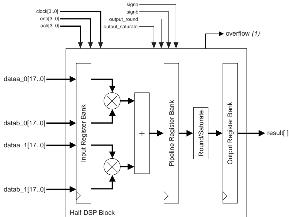
Figure 4-11. Two-Multiplier Adder Mode Shown for Half-DSP Block (Note 2)
