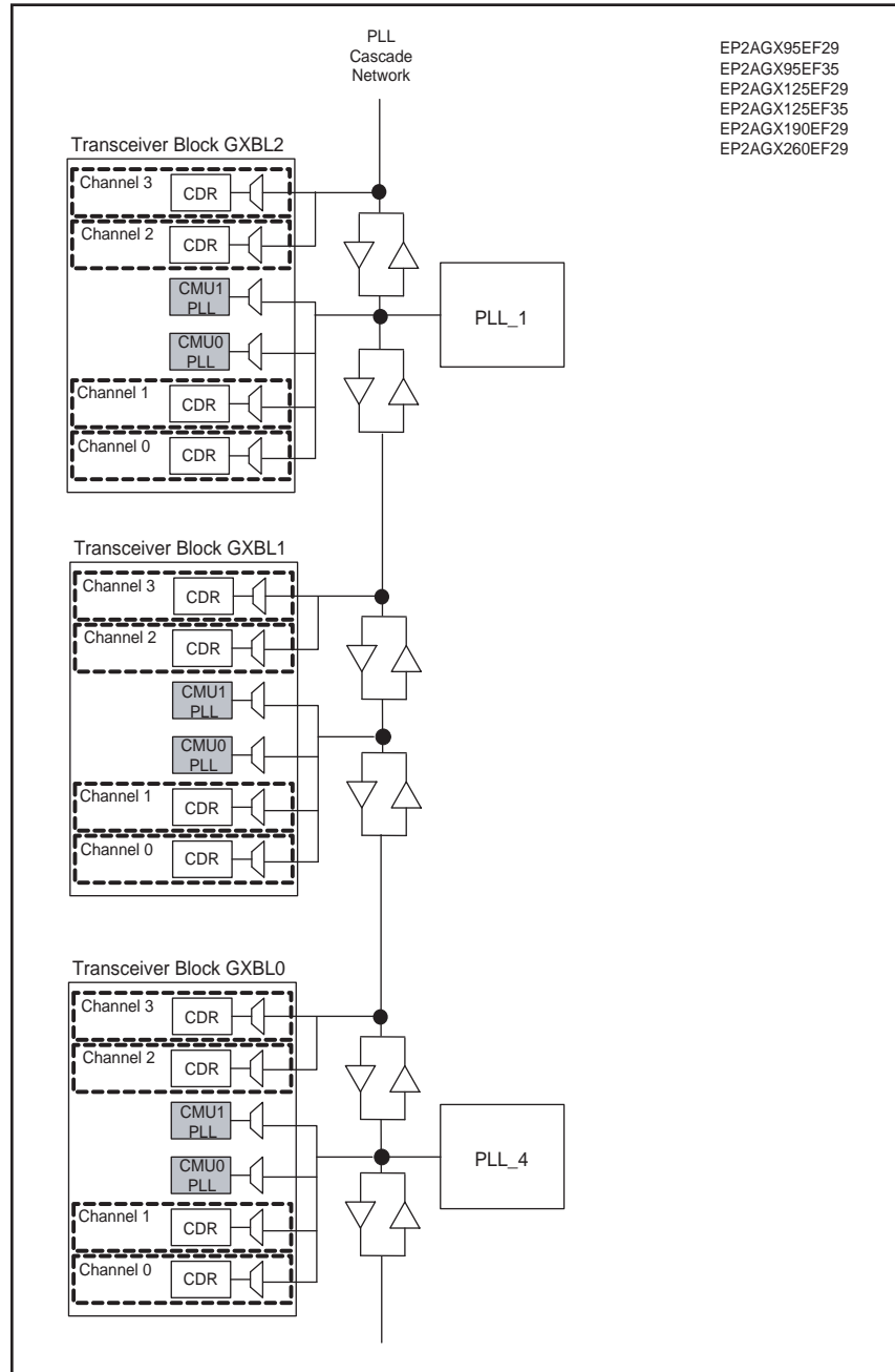
Figure 2-31. FPGA Fabric PLLs Transceiver PLLs Cascading Option Allowed in the EP2AGX95EF29, EP2AGX95EF35, EP2AGX125EF29, EP2AGX125EF35, EP2AGX190EF29, and EP2AGX260EF29 Devices
