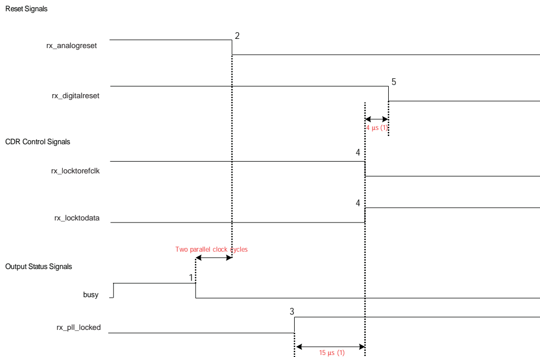
Figure 4-7. Sample Reset Sequence of Receiver-Only Channel—Receiver CDR in Manual Lock Mode
