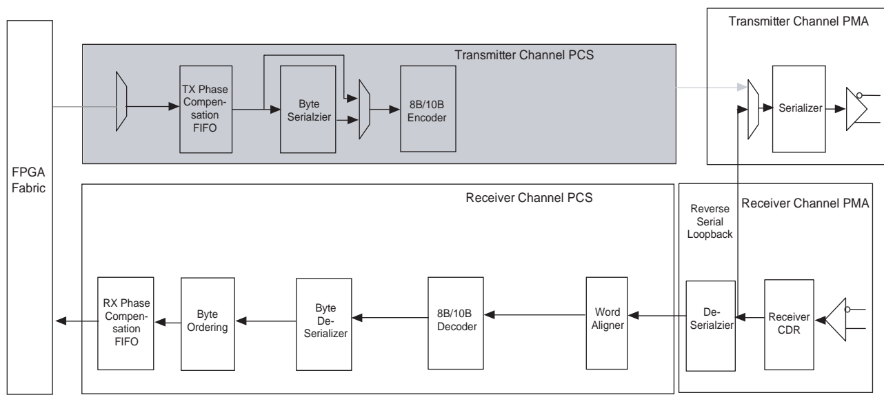
Figure 1-110. Reverse Serial Loopback Datapath (Grayed-Out Blocks are Not Active in this Mode)
