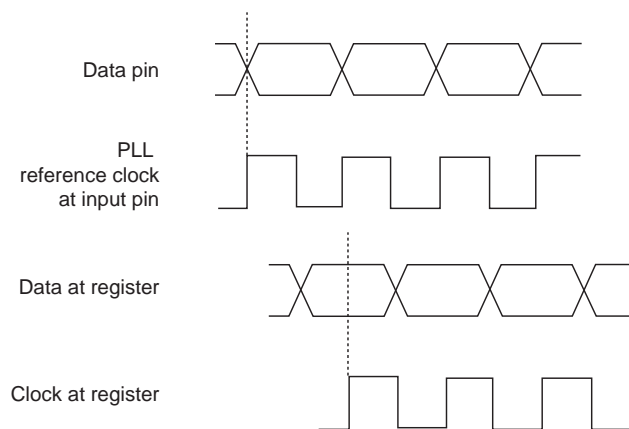
Figure 5-16. Source-Synchronous Mode for LVDS Compensation
