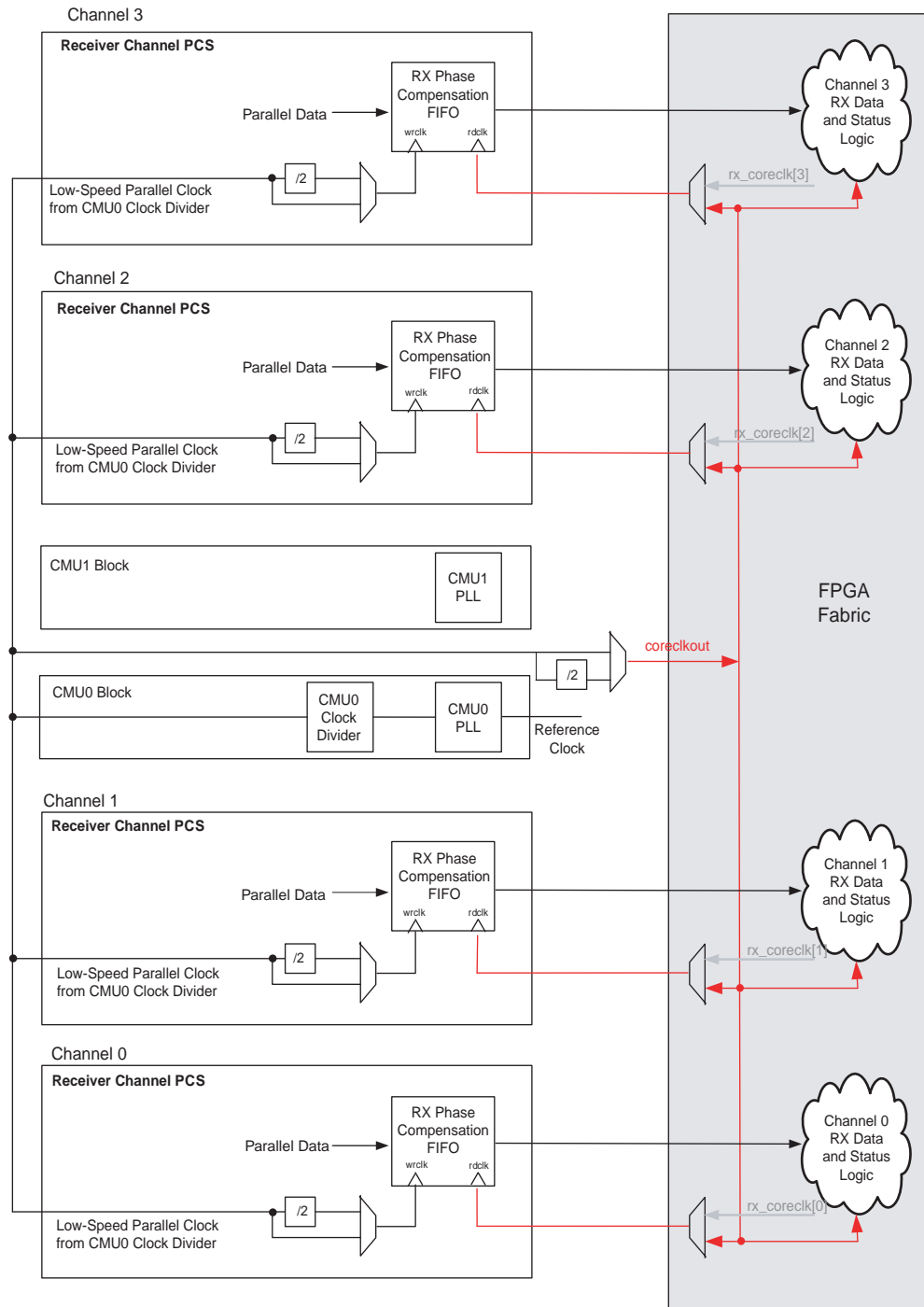
Figure 2-25. FPGA Fabric-Receiver Interface Clocking in an ×4 Bonded Channel Configuration
