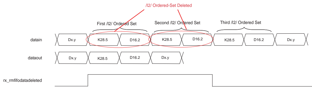
Figure 1-56. Example of Rate Match Deletion in GIGE Mode
