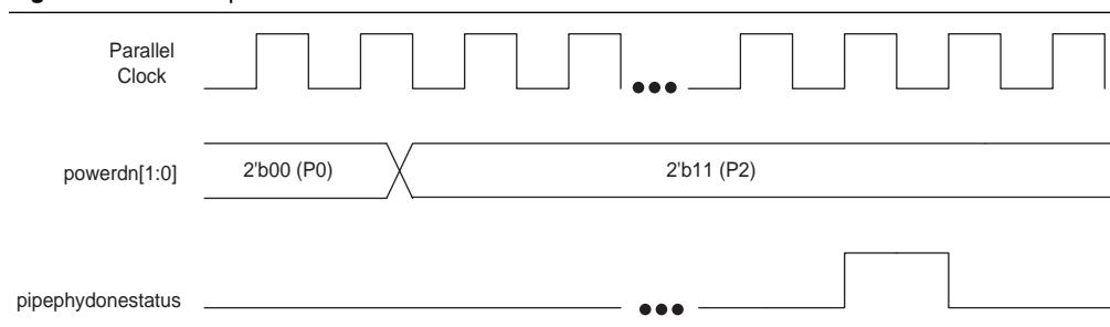
Figure 1-79. Example of Power State Transition from P0 to P2
