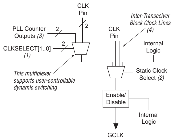
Figure 5-7. Arria II GX Global Clock Control Block
