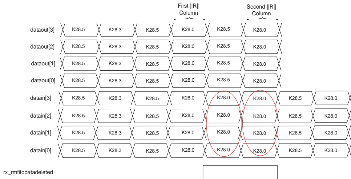
Figure 1-90. Example of Rate Match Insertion in XAUI Mode
