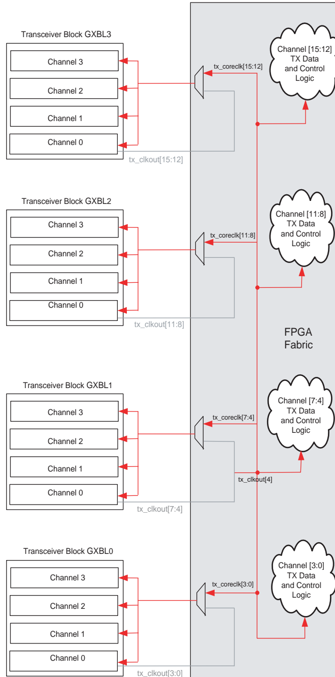
Figure 2-21. Sixteen Identical Channels across Four Transceiver Blocks for Example 5
