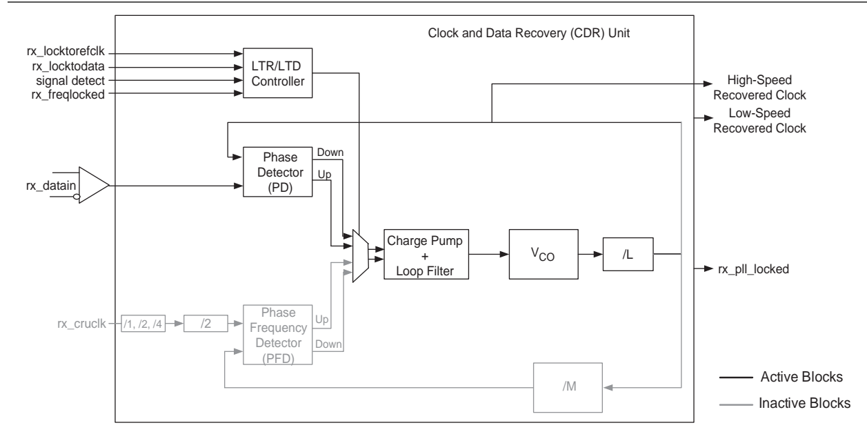
Figure 1-39. CDR in Lock-To-Data Mode
