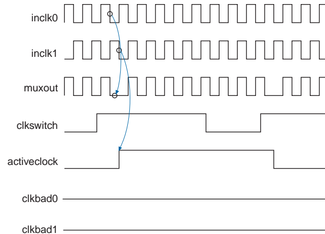
Figure 5–24. Clock Switchover Using the clkswitch (Manual) Control (Note 1)
