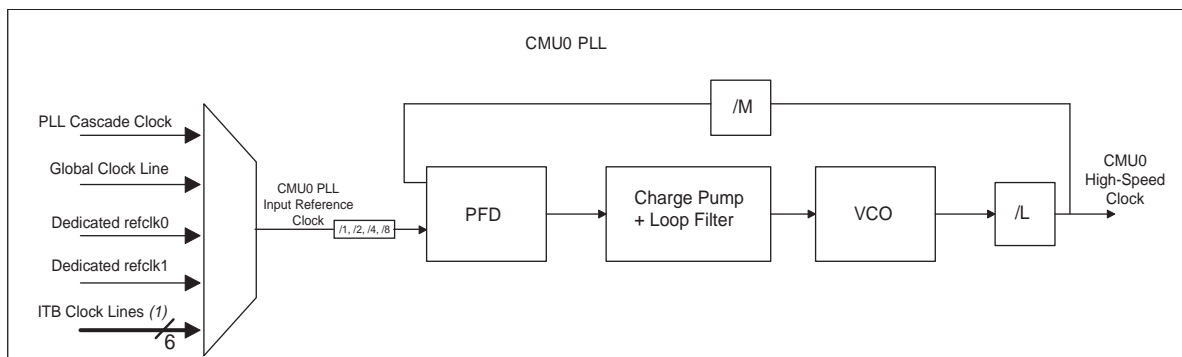
Figure 1-9. Diagram of the CMU0 PLL
