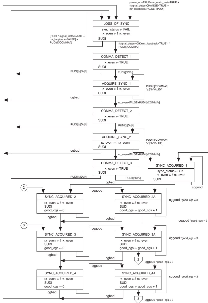
Figure 1-86. IEEE 802.3ae PCS Synchronization State Diagram (Note 1)
