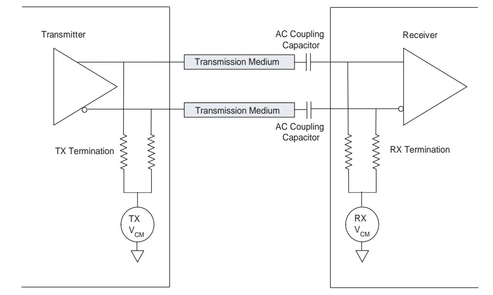
Figure 1-31. AC-Coupled Link
