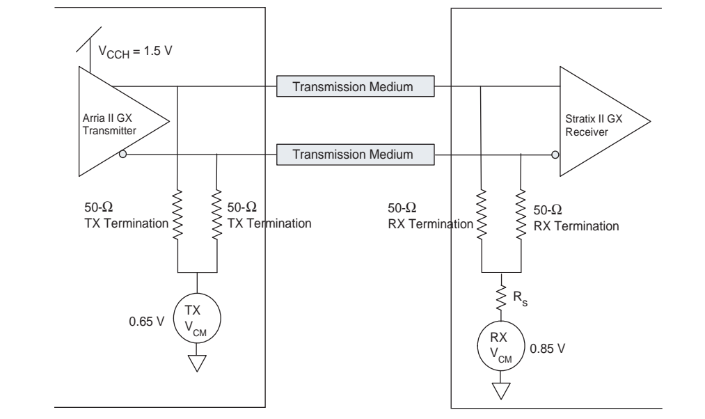
Figure 1-35. Arria II GX Transmitter (PCML) to Stratix II GX Receiver (PCML) DC-Coupled Link
