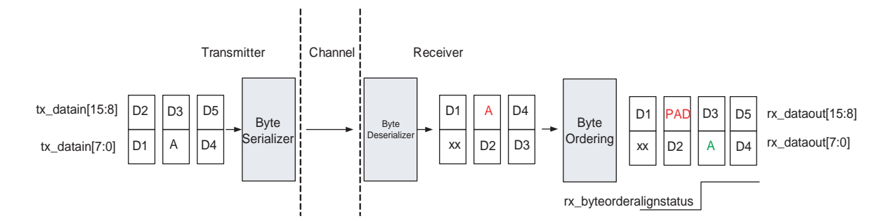
Figure 1-68. Example of Byte Ordering in Single-Width Modes
