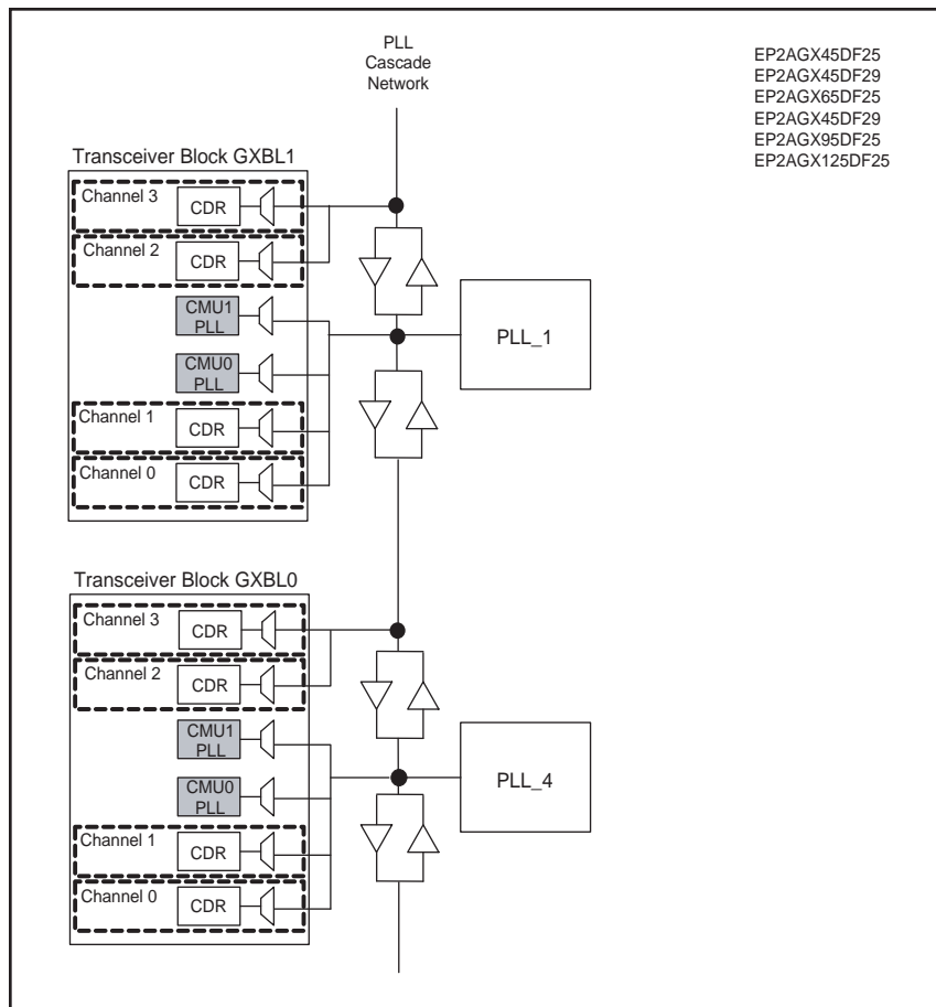
Figure 2-30. FPGA Fabric PLLs-Transceiver PLLs Cascading Option Allowed in the EP2AGX45DF25, EP2AGX45DF29, EP2AGX65DF25, EP2AGX45DF29, EP2AGX95DF25, and EP2AGX125DF25 Devices
