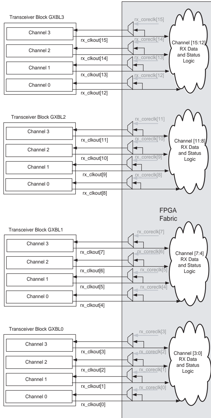
Figure 2-26. Sixteen Non-Bonded Receiver Channels without Rate Matcher for Example 8
