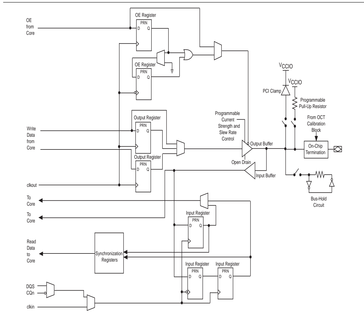
Figure 6-2. Arria II GX IOE Structure
