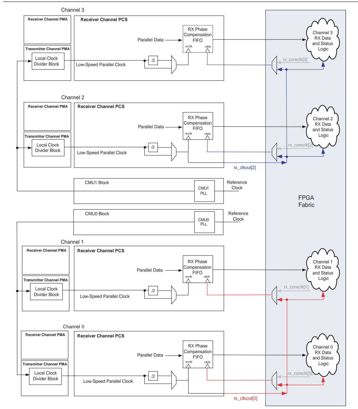
Figure 2-23. FPGA Fabric-Receiver Interface Clocking for Example 7
