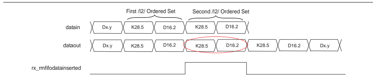
Figure 1–57. Example of Rate Match Insertion in GIGE Mode
