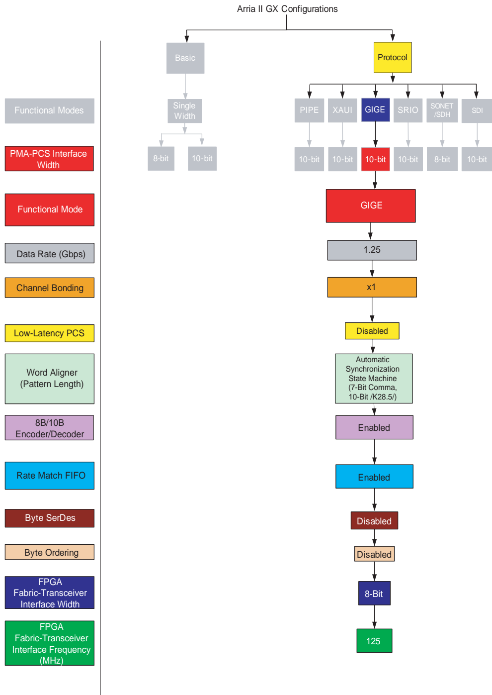
Figure 1-92. GIGE Mode
