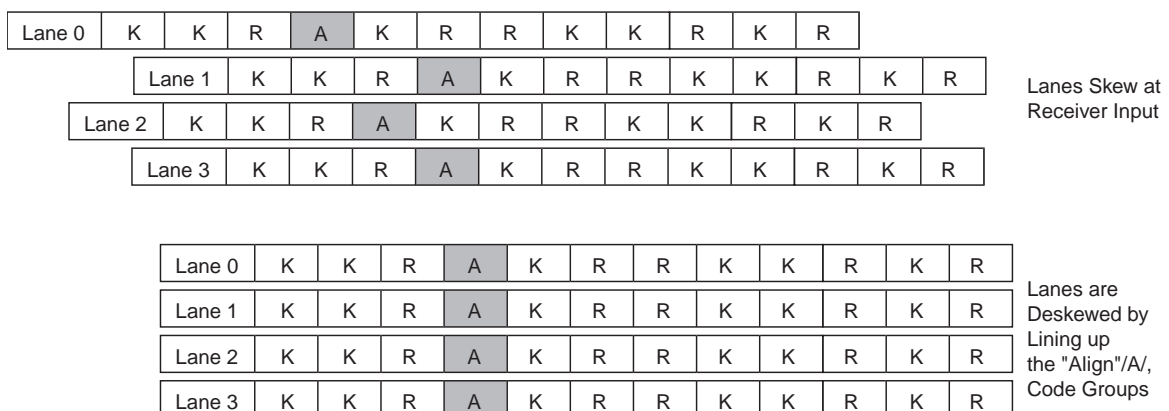
Figure 1-87. Receiver Input Lane Skew in XAUI Mode
