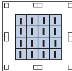
Figure 5-4. Sixteen Independent Sub-Regional Clock Regions (Note 1)
