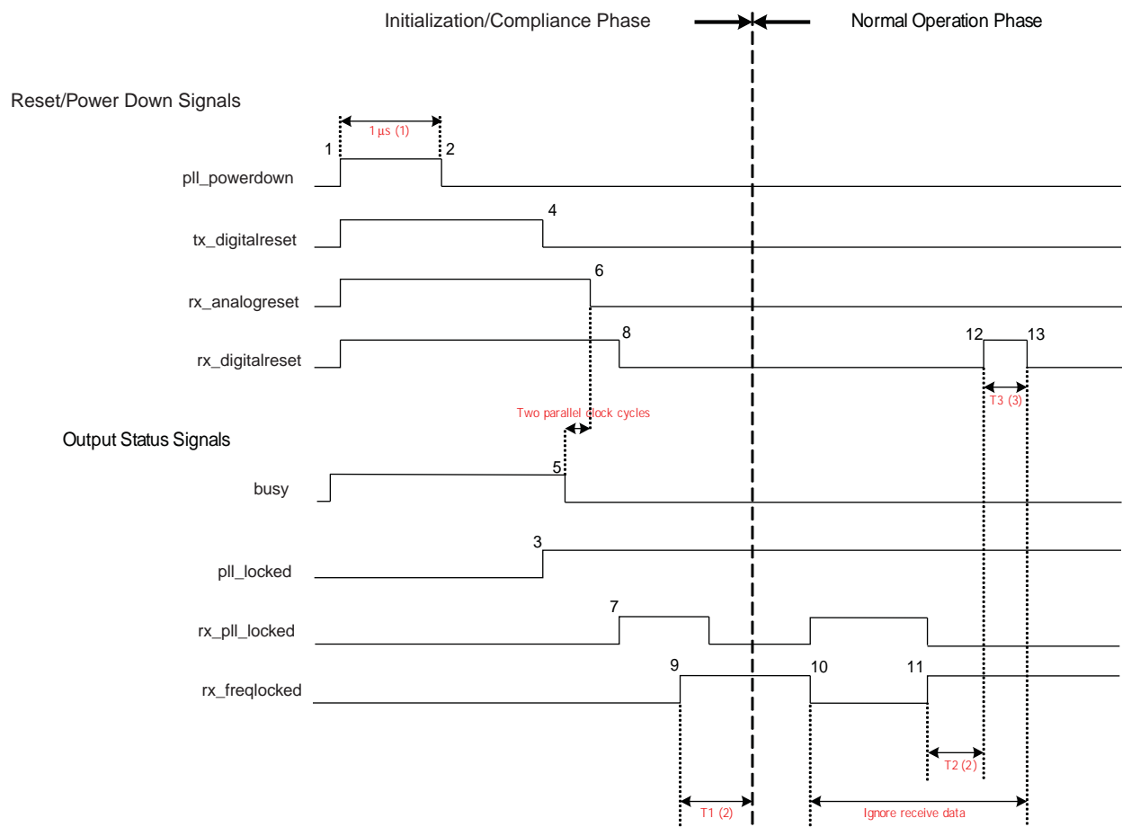
Figure 4-10. Reset Sequence of PCI Express (PIPE) Functional Mode
