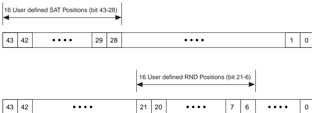
Figure 4-17. Round and Saturation Locations
