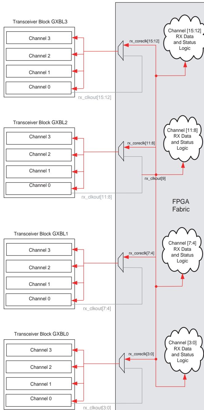
Figure 2-28. Sixteen Channels across Four Transceiver Blocks for Example 10
