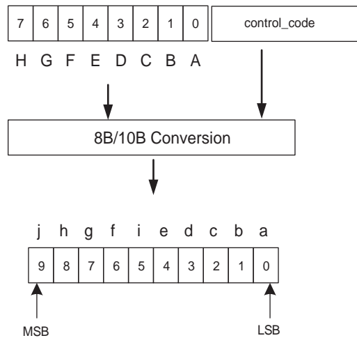
Figure 1-18. 8B/10B Conversion Format
