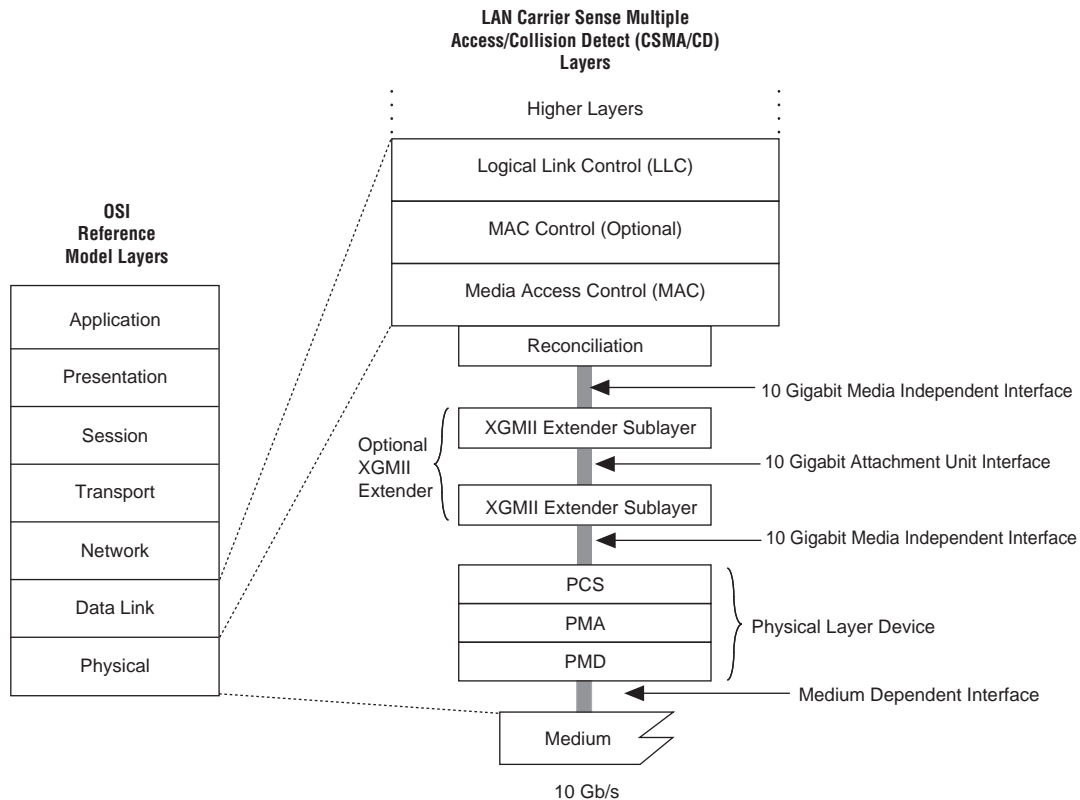
Figure 1-81. XAUI and XGMII Layers
