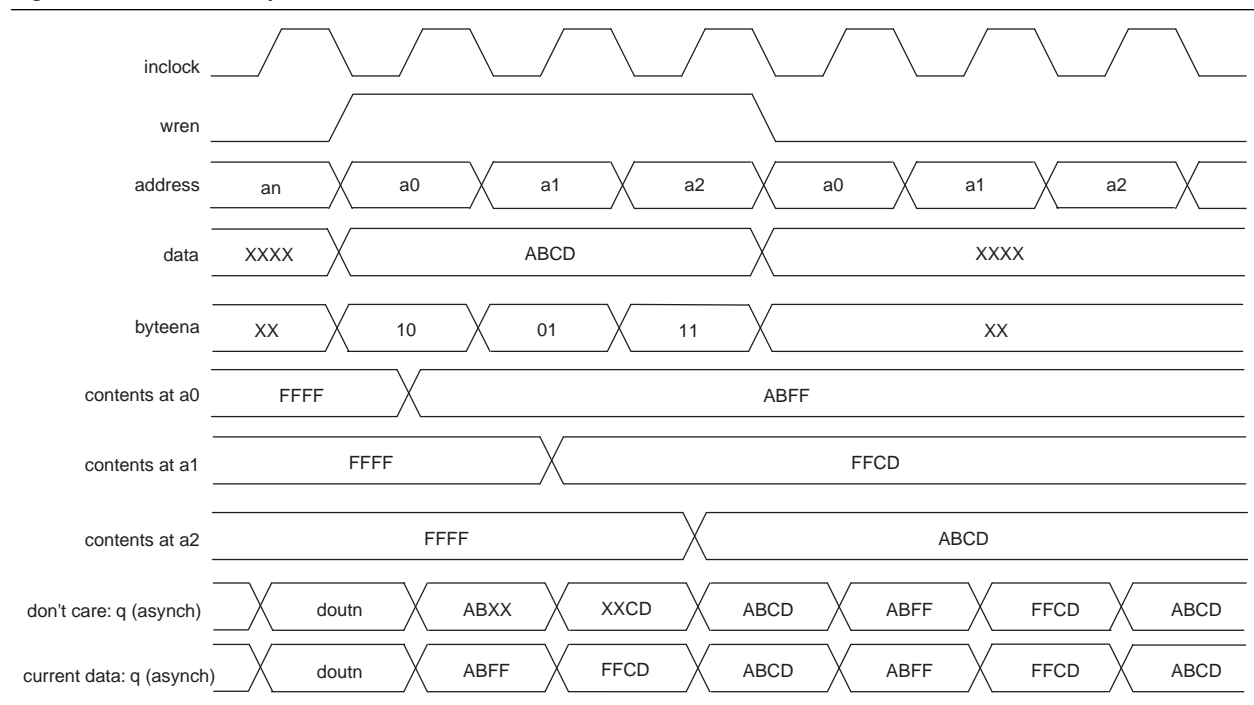
Figure 3-1. Arria II GX Byte Enable Functional Waveform
