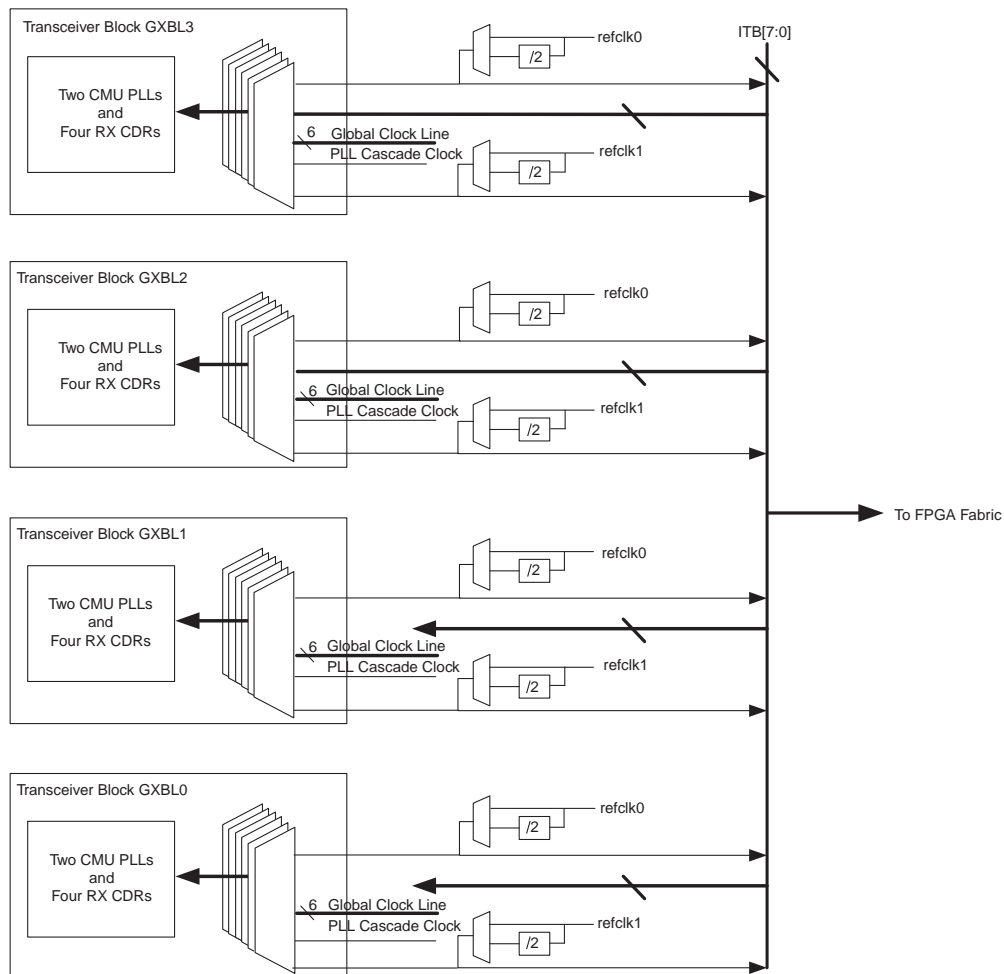
Figure 2-4. Inter-Transceiver Block Clock Lines (Note 1)
