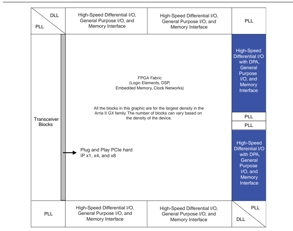
Figure 1-1. Arria II GX Device Architecture Overview
