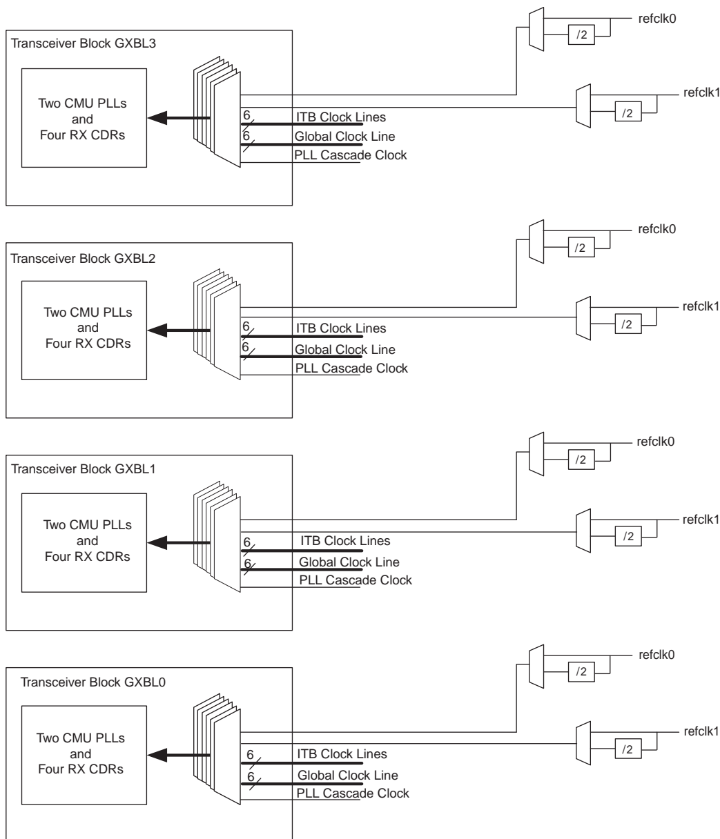
Figure 2-2. Input Reference Clock Sources across Transceiver Blocks
