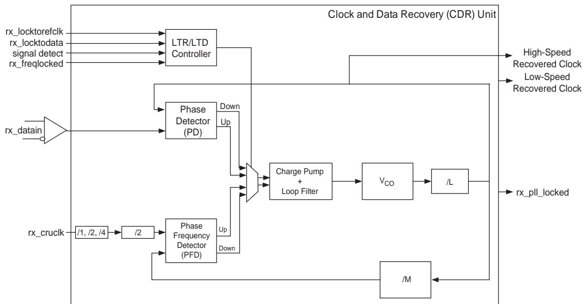
Figure 1–37. CDR Unit
