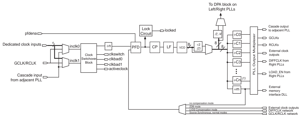
Figure 5-13. Arria II GX PLL Block Diagram
