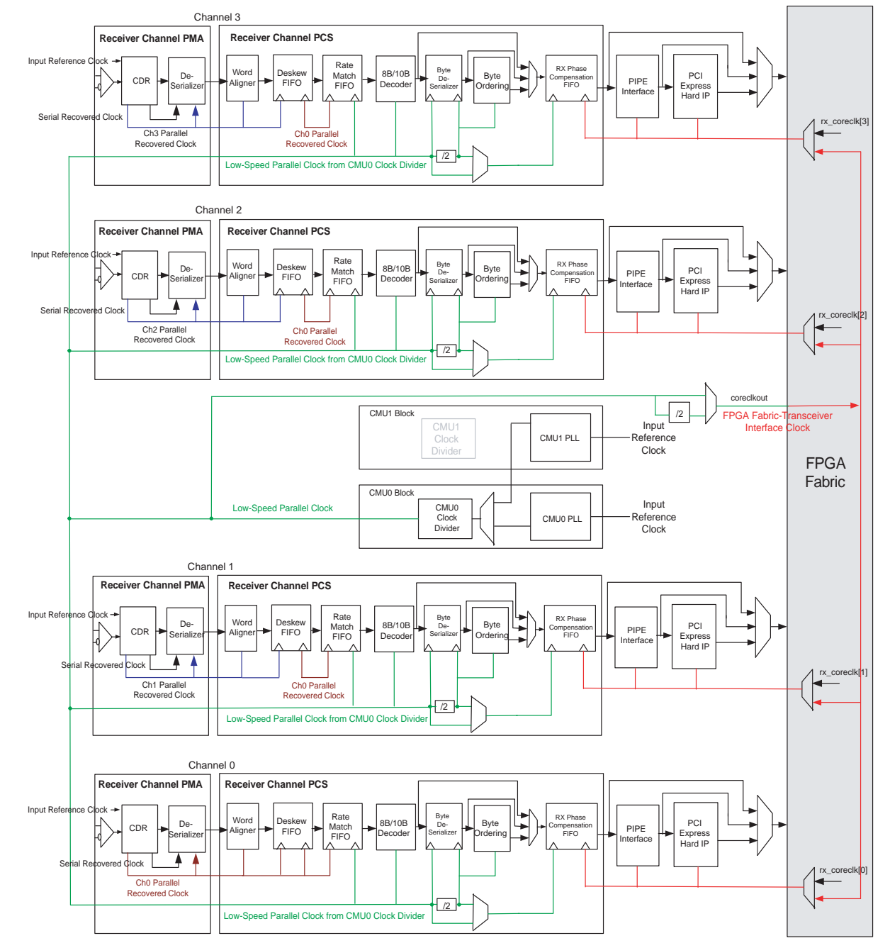
Figure 2-13. Receiver Datapath Clocking in \times 4 Bonded Channel Configuration with Deskew FIFO
