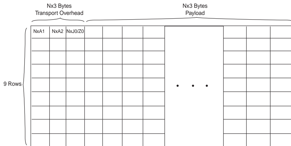
Figure 1-99. SONET/SDH Mode
