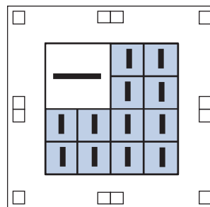
Figure 5-6. Twelve Independent Sub-Regional + One Regional Clock Region (Note 1)
