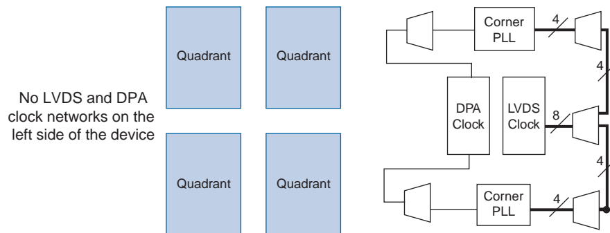
Figure 8-16. LVDS and DPA Clock Networks in the Arria II GX Family without Center PLLs
