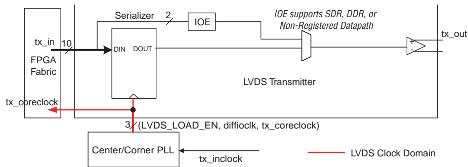
Figure 8-3. Arria II GX LVDS Transmitter Block Diagram (Note 1), (2)
