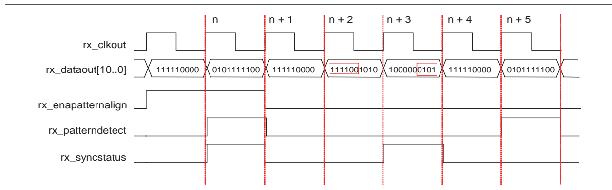
Figure 1-45. Word Aligner in 10-Bit PMA-PCS Manual Alignment Mode
