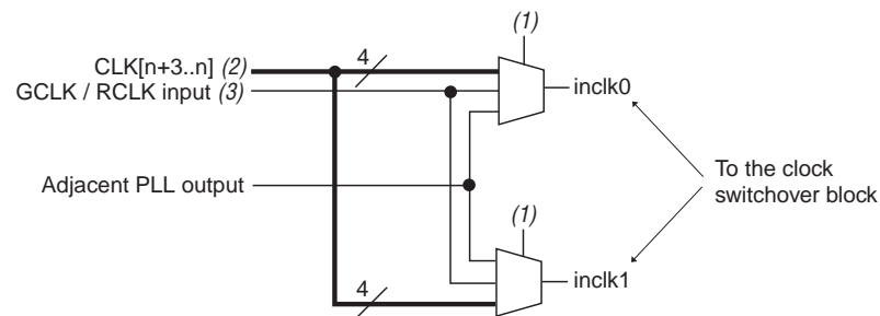
Figure 5-12. Clock Input Multiplexer Logic for Arria II GX PLLs
