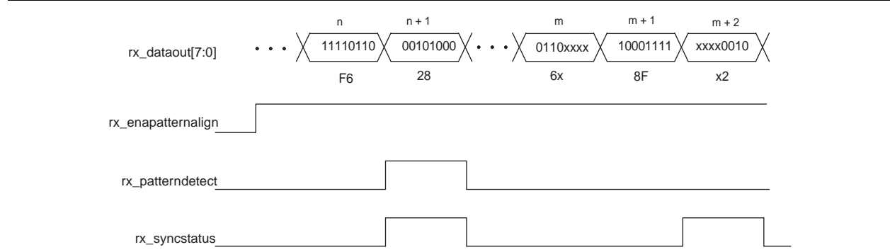
Figure 1-43. Bit-Slip Mode in 8-Bit PMA-PCS Interface Mode
