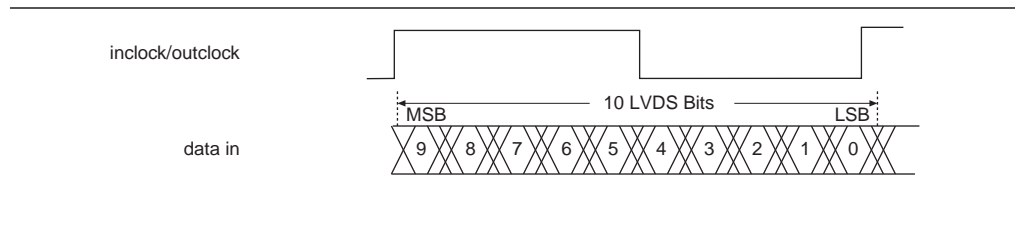
Figure 8-18. Bit Orientation
