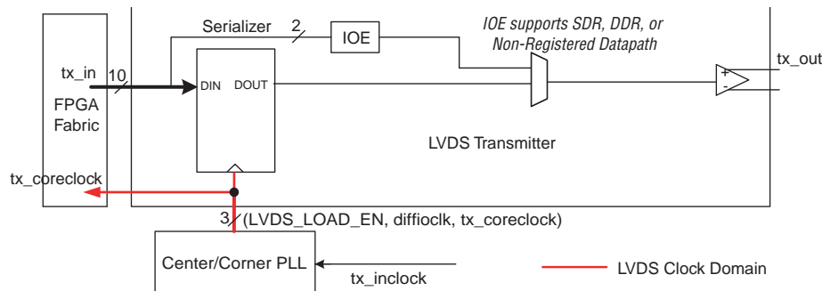
Figure 8-4. Arria II GX Serializer Bypass (Note 1), (2), (3)
