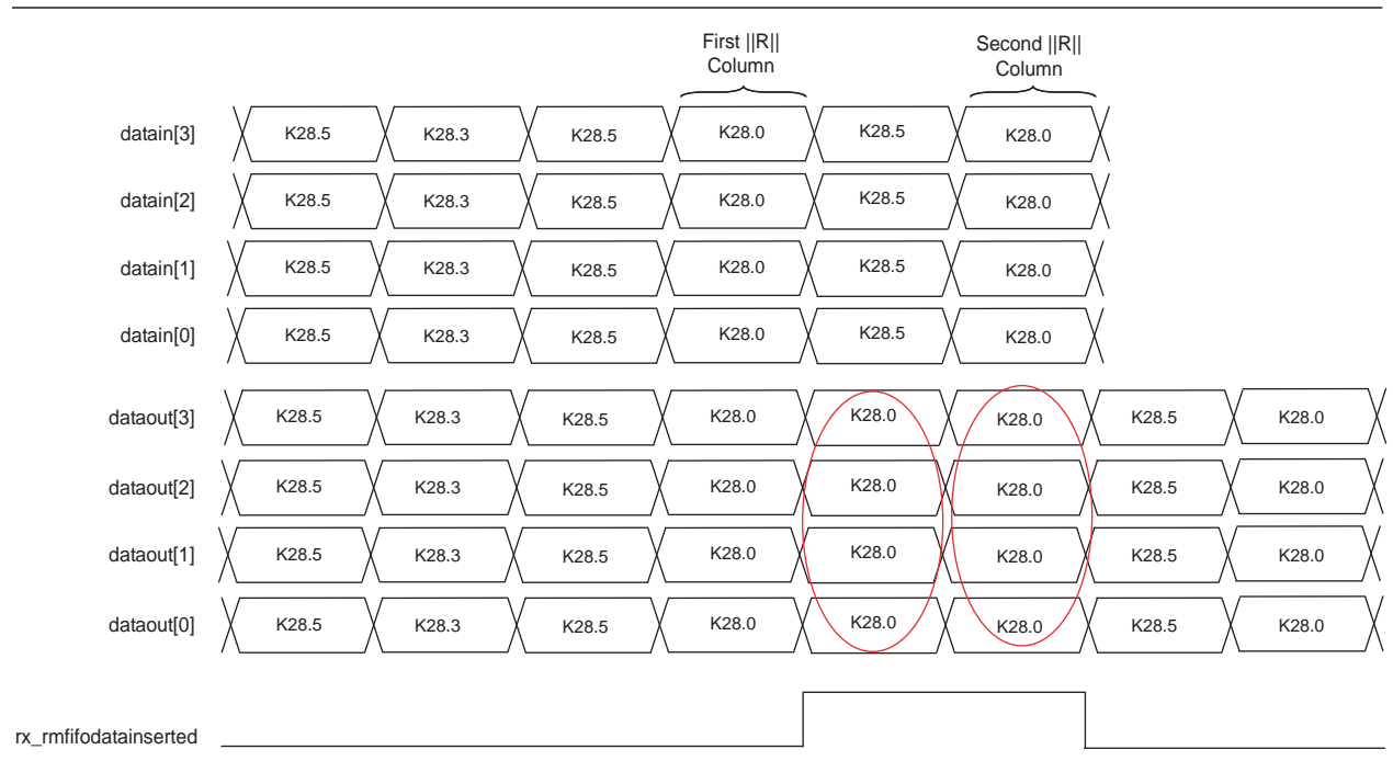
Figure 1-55. Example of Rate Match Insertion in XAUI Mode
