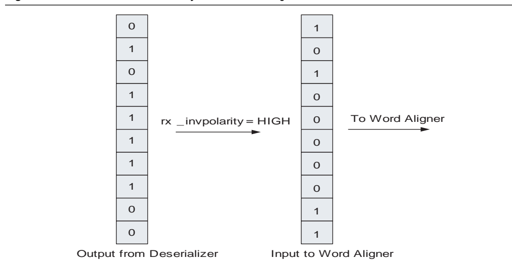
Figure 1-46. 10-Bit Receiver Polarity Inversion in Single-Width Mode
