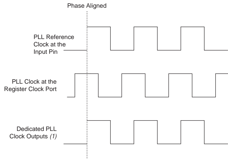
Figure 5-19. Phase Relationship Between PLL Clocks in Zero Delay Buffer Mode
