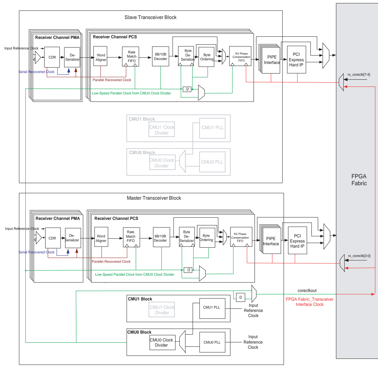
Figure 2-15. Receiver Datapath Clocking in \times 8 Bonded Channel Configuration
