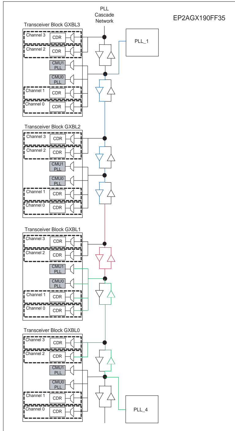
Figure 2-33. Illegal FPGA Fabric-Transceiver PLL Cascading Configuration
