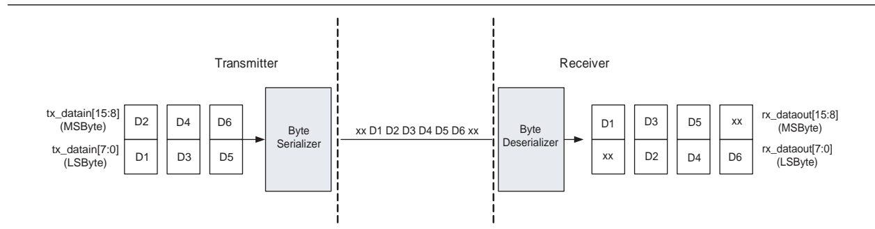
Figure 1-67. MSByte and LSByte of the Two-Byte Transmitter Data Straddled Across Two Word Boundaries
