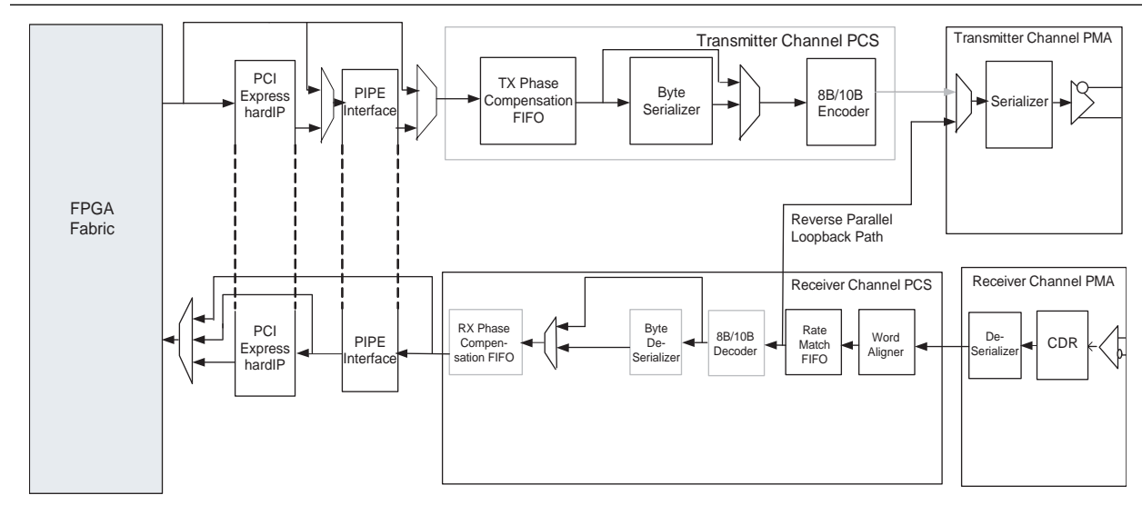
Figure 1-112. PCI Express (PIPE) Reverse Parallel Loopback Mode Datapath
