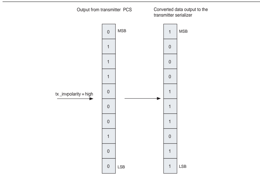
Figure 1–22. Transmitter Polarity Inversion in Single-Width Mode
