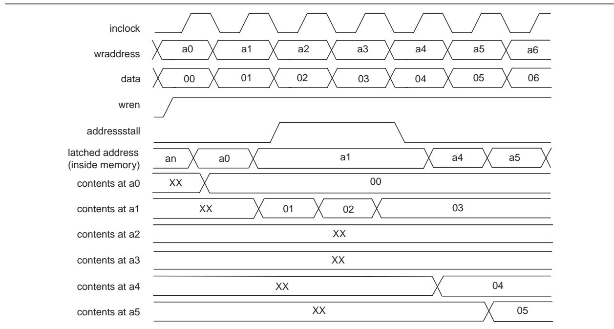
Figure 3-4. Arria II GX Address Clock Enable during Write Cycle Waveform
