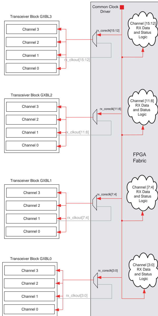
Figure 2-27. Sixteen Identical Channels across Four Transceiver Blocks for Example 9
