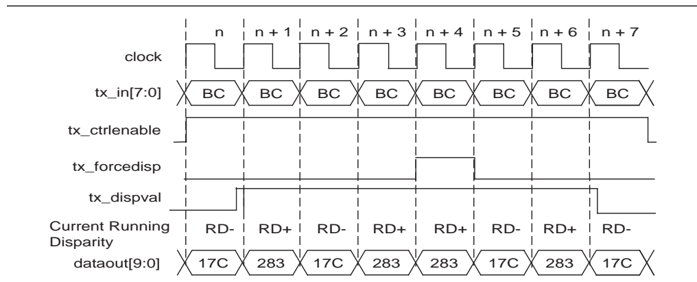
Figure 1-21. 8B/10B Encoder Force Running Disparity Operation in Single-Width Mode
