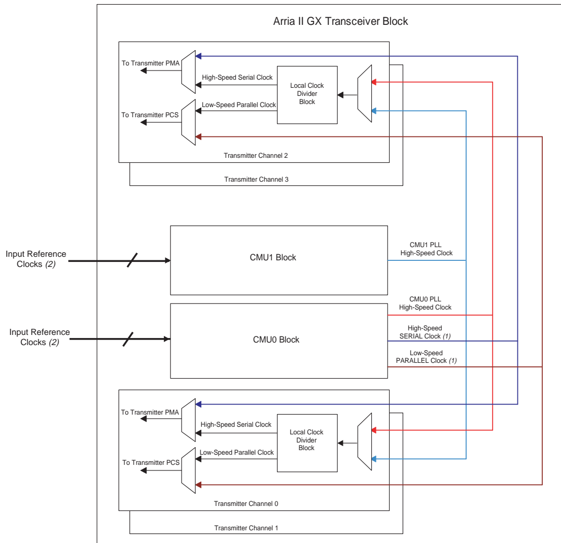
Figure 1-7. Top-Level Diagram of CMU Channels in a Transceiver Block
