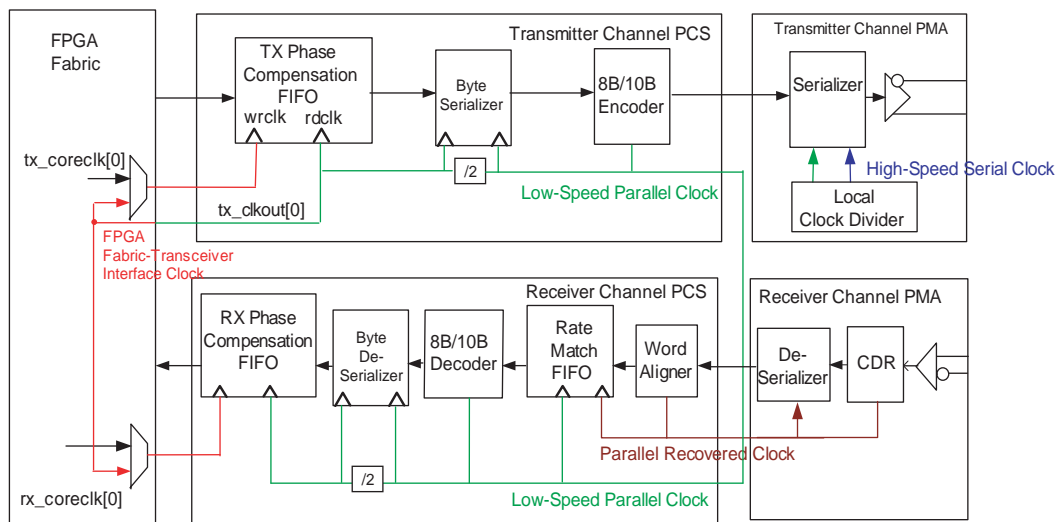
Figure 1-106. Serial RapidIO Mode Datapath
