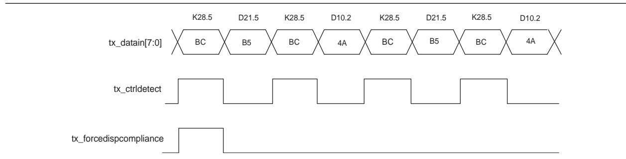
Figure 1-77. Compliance Pattern Transmission Support, 8-Bit Wide Channel Configurations
