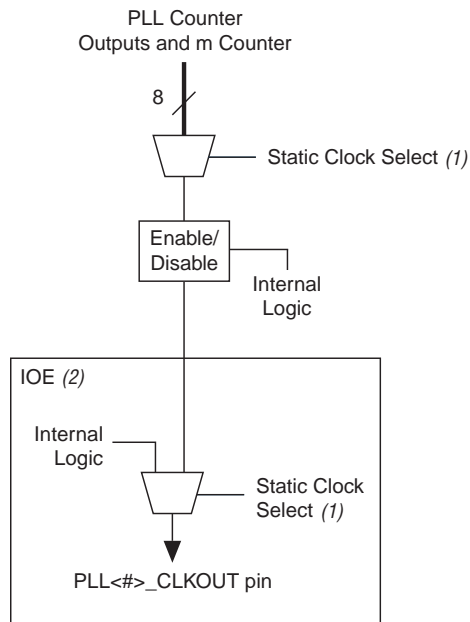
Figure 5-9. Arria II GX External PLL Output Clock Control Block
