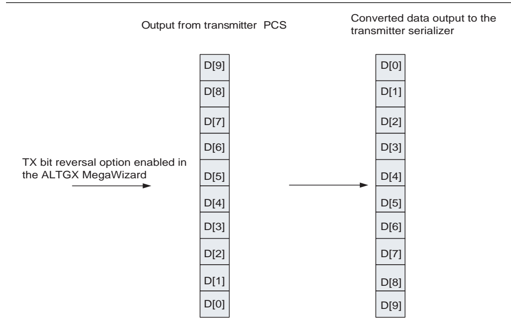
Figure 1-23. Transmitter Bit Reversal Operation in Basic Single-Width Mode
