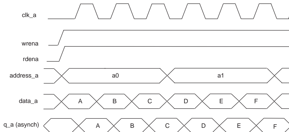
Figure 3-14. Same Port Read-During Write: New Data Mode
