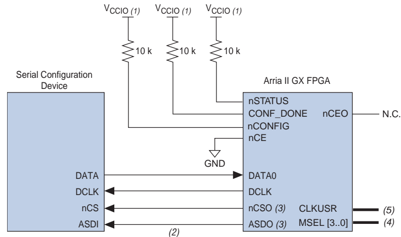
Figure 9-6. Single Device Fast AS Configuration
