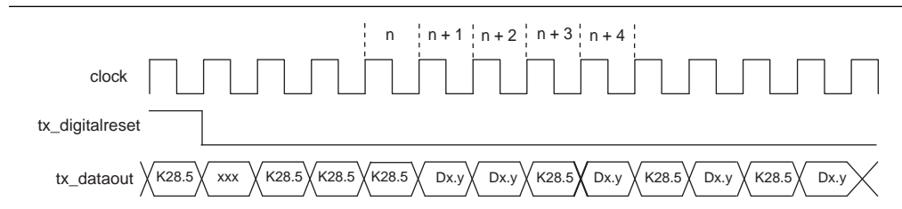
Figure 1-95. Example of Reset Condition in GIGE Mode
