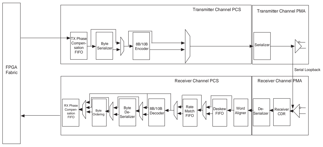
Figure 1-109. Serial Loopback Datapath
