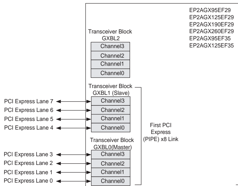
Figure 2-9. Two PCI Express (PIPE) ×8 Link in Three Transceiver Block Devices (Note 1)
