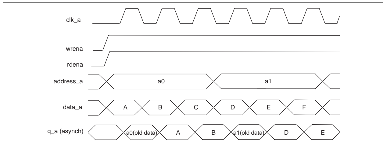
Figure 3-7. Timing Waveform for Read-Write Operations (Single-Port Mode)
