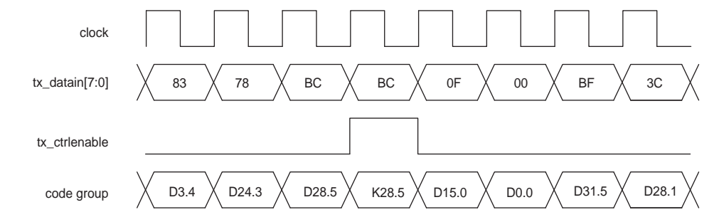
Figure 1-19. Control Word and Data Word Transmission
