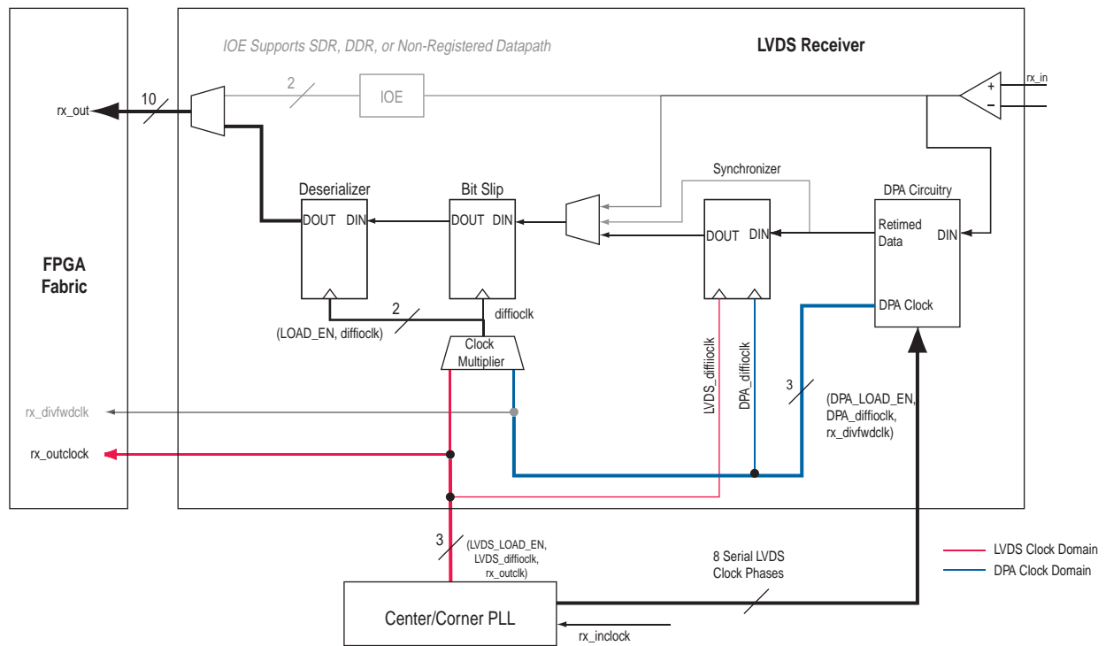
Figure 8-12. Receiver Datapath in DPA Mode (Note 1), (2), (3)
