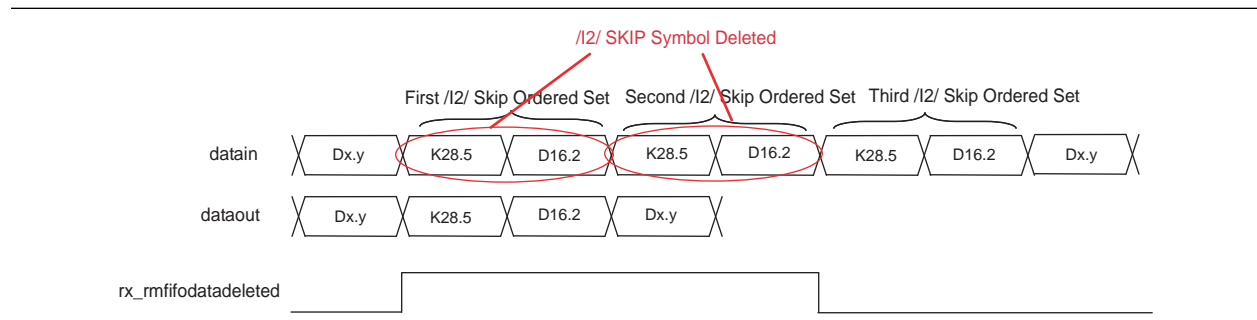
Figure 1-97. Example of Rate Match Deletion in GIGE Mode
