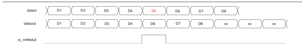
Figure 1-60. Rate Match FIFO Full Condition in Basic Single-Width Mode
