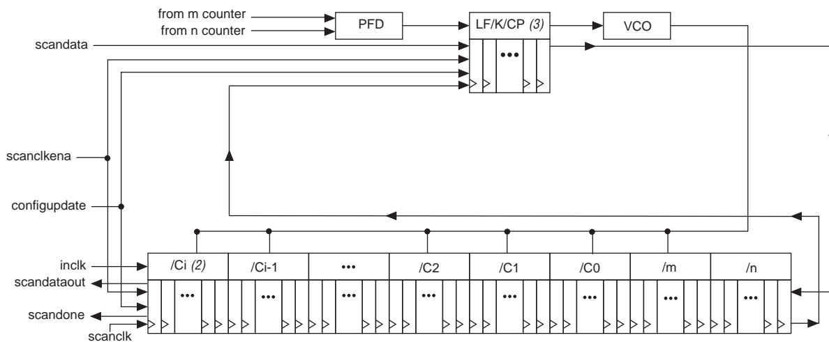
Figure 5-27. PLL Reconfiguration Scan Chain
