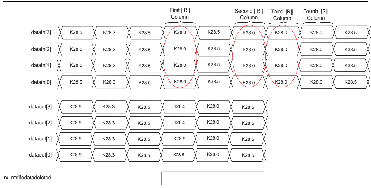
Figure 1-54. Example of Rate Match Deletion in XAUI Mode
