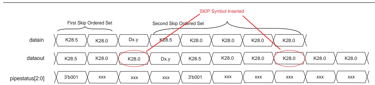
Figure 1-51. Example of Rate Match Insertion in PCI Express (PIPE) Mode
