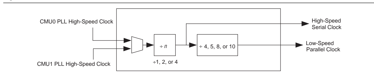
Figure 1-28. Transmitter Local Clock Divider Block
