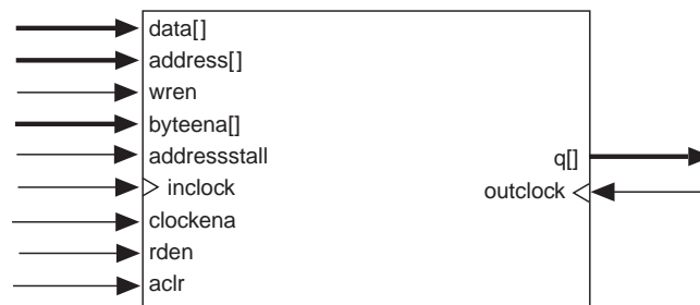
Figure 3-6. Single-Port Memory (Note 1)
