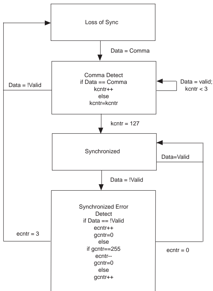
Figure 1-108. Synchronization State Machine in Serial RapidIO Mode
