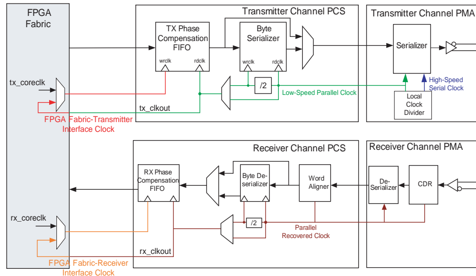
Figure 1-105. SDI Mode Datapath
