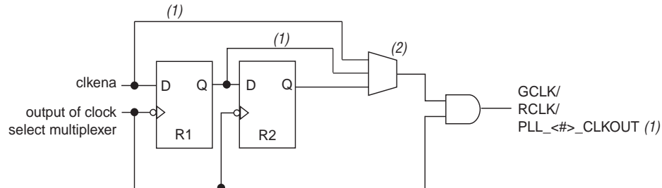
Figure 5-10. clkena Implementation
