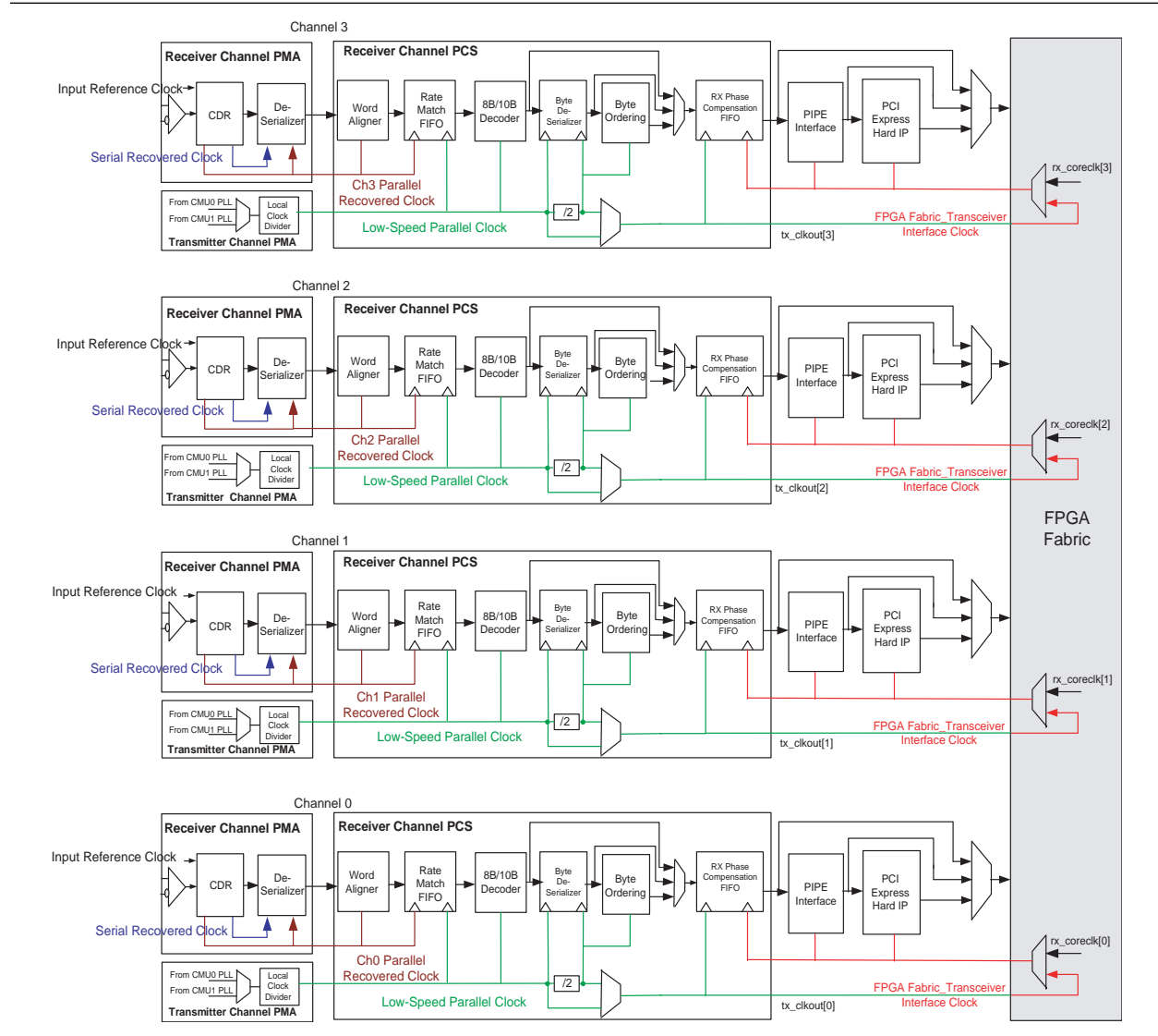
Figure 2-12. Receiver Datapath Clocking in Non-Bonded Configurations with Rate Matcher
