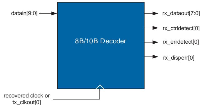
Figure 1-62. 8B/10B Decoder in Single-Width Mode
