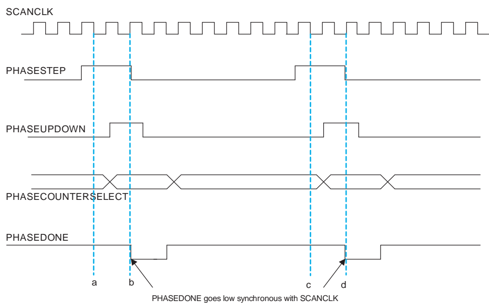
Figure 5–31. Dynamic Phase Shifting Waveform
