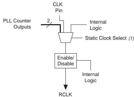
Figure 5-8. Regional Clock Control Block
