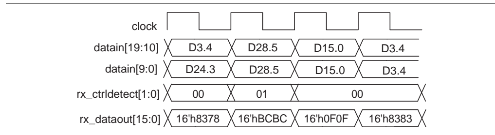
Figure 1-65. 8B/10B Decoder 10-Bit Control Code Group
