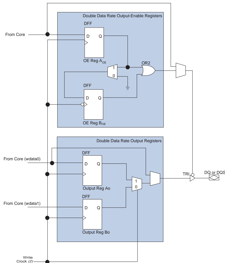
Figure 7-18. Arria II GX IOE Output and Output-Enable Path Registers (Note 1)
