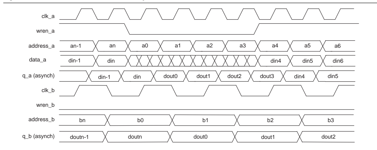
Figure 3-11. Arria II GX True Dual-Port Timing Waveform
