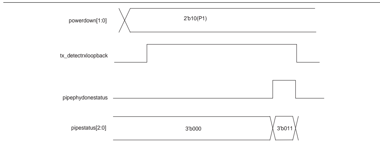
Figure 1-75. Receiver Detect, Successfully Detected
