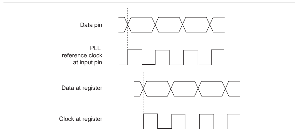
Figure 5-15. Phase Relationship Between Clock and Data in Source-Synchronous Mode
