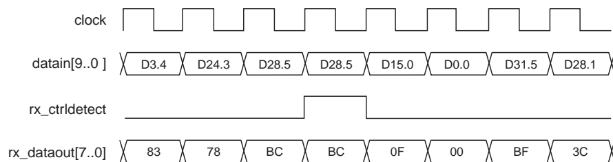
Figure 1-64. 8B/10B Decoder in Control Code Group Detection
