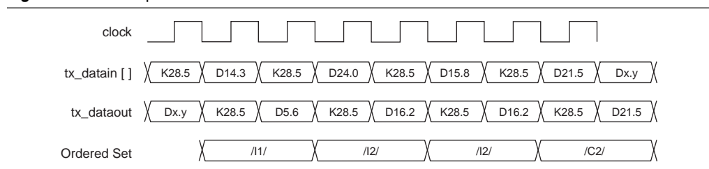
Figure 1-94. Example of Automatic Ordered Set Generation
