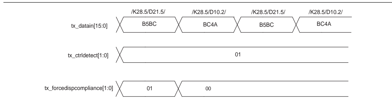
Figure 1-78. Compliance Pattern Transmission Support, 16-Bit Wide Channel Configurations
