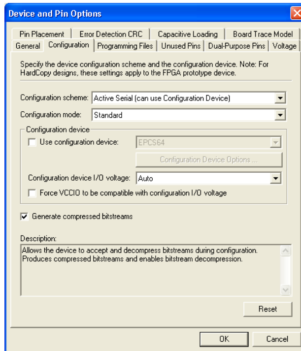
Figure 10-2. Enabling the Error Detection CRC Feature in the Quartus II Software
