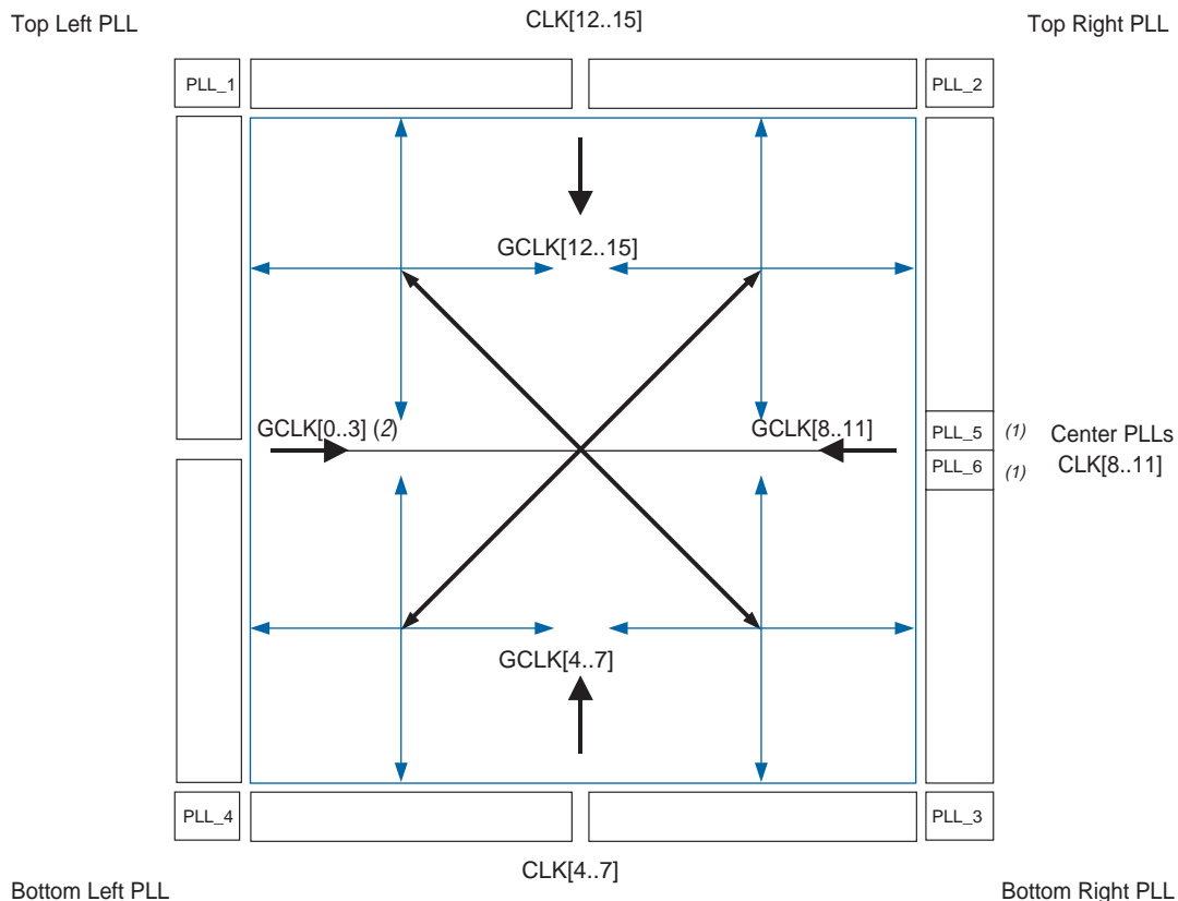
Figure 5-1. Global Clock Networks
