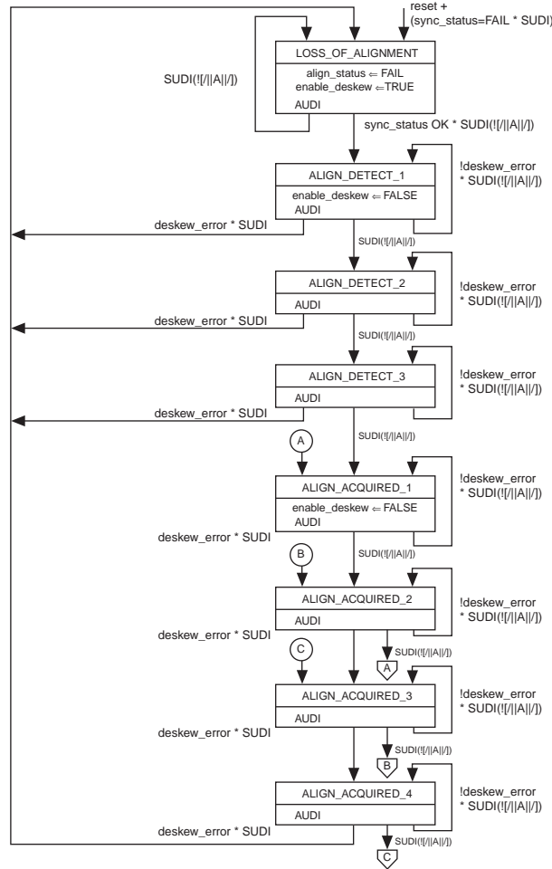
Figure 1-88. Deskew FIFO in XAUI Mode (Note 1)
