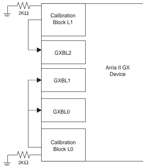
Figure 1-114. Calibration Three-Transceiver Blocks
