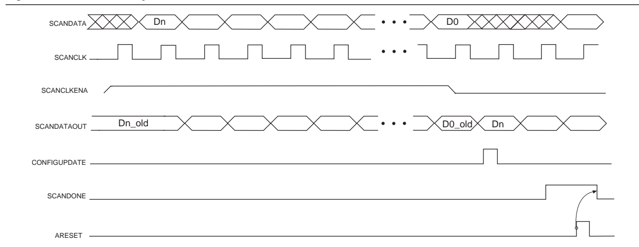
Figure 5–28. PLL Reconfiguration Waveform
