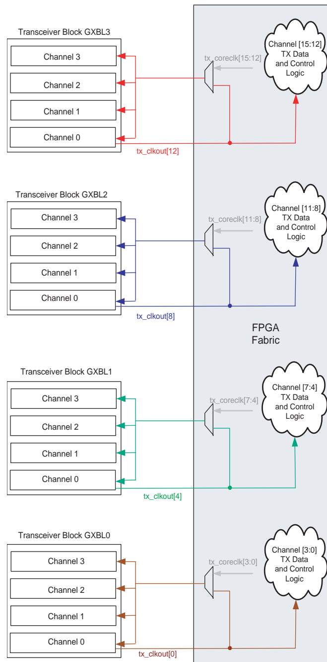
Figure 2-19. Sixteen Identical Channels across Four Transceiver Blocks for Example 3
