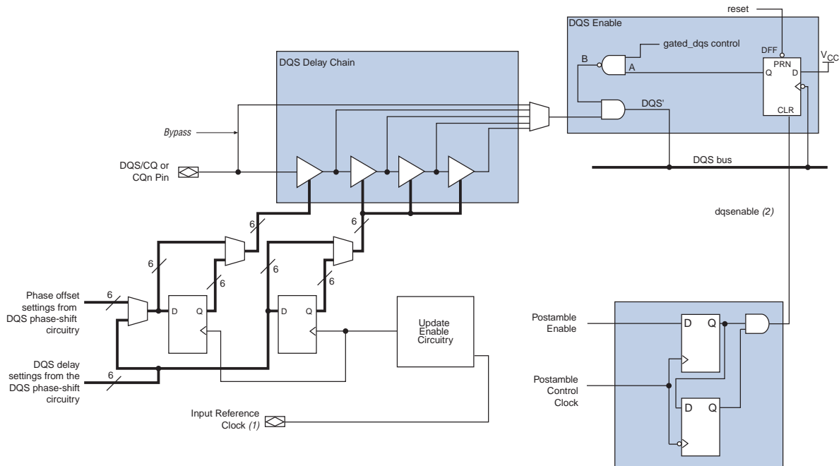
Figure 7-13. Arria II GX DQS Logic Block
