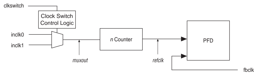
Figure 5–25. Manual Clock Switchover Circuitry in Arria II GX PLLs
