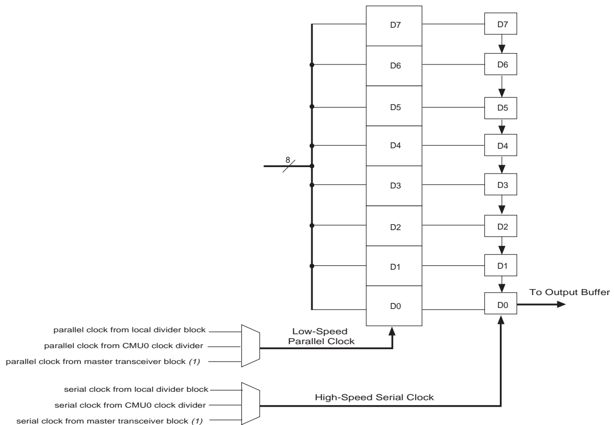
Figure 1-24. Serializer Block in an 8-Bit PCS-PMA Interface
