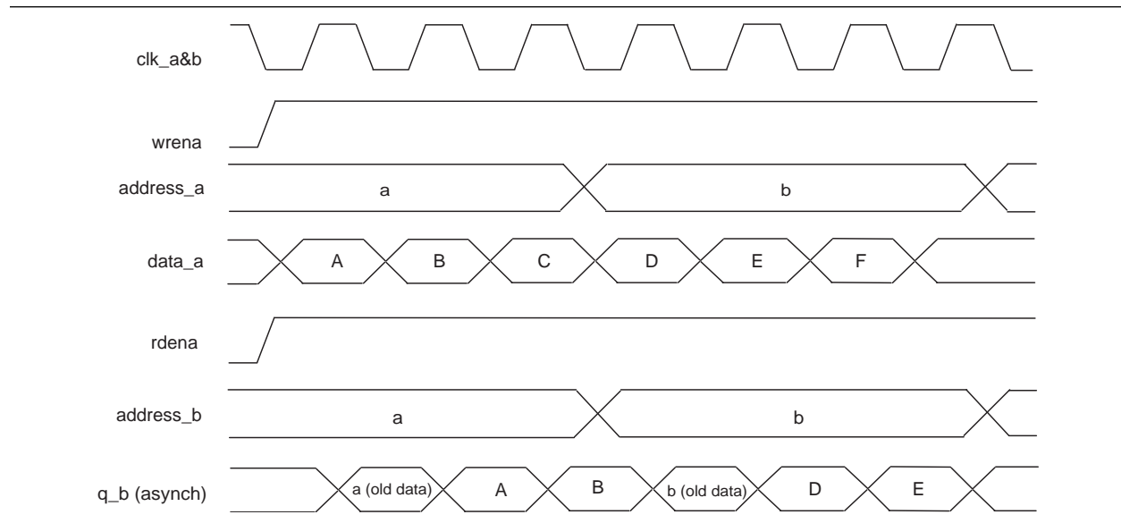
Figure 3-16. Mixed Port Read During Write: Old Data Mode
