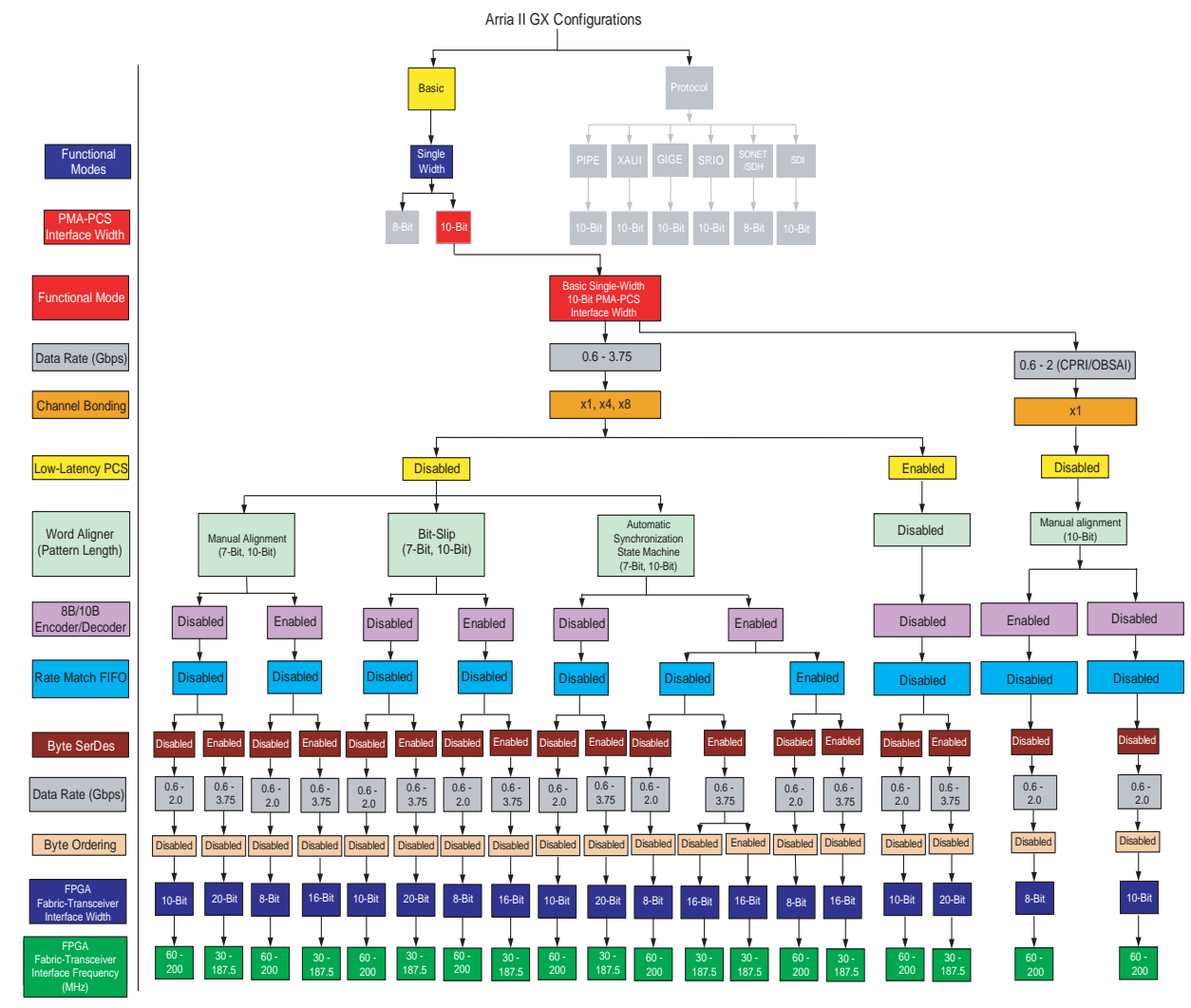
Figure 1-70. Transceiver Configurations in Basic Single-Width Mode with a 10-Bit Wide PMA-PCS Interface
