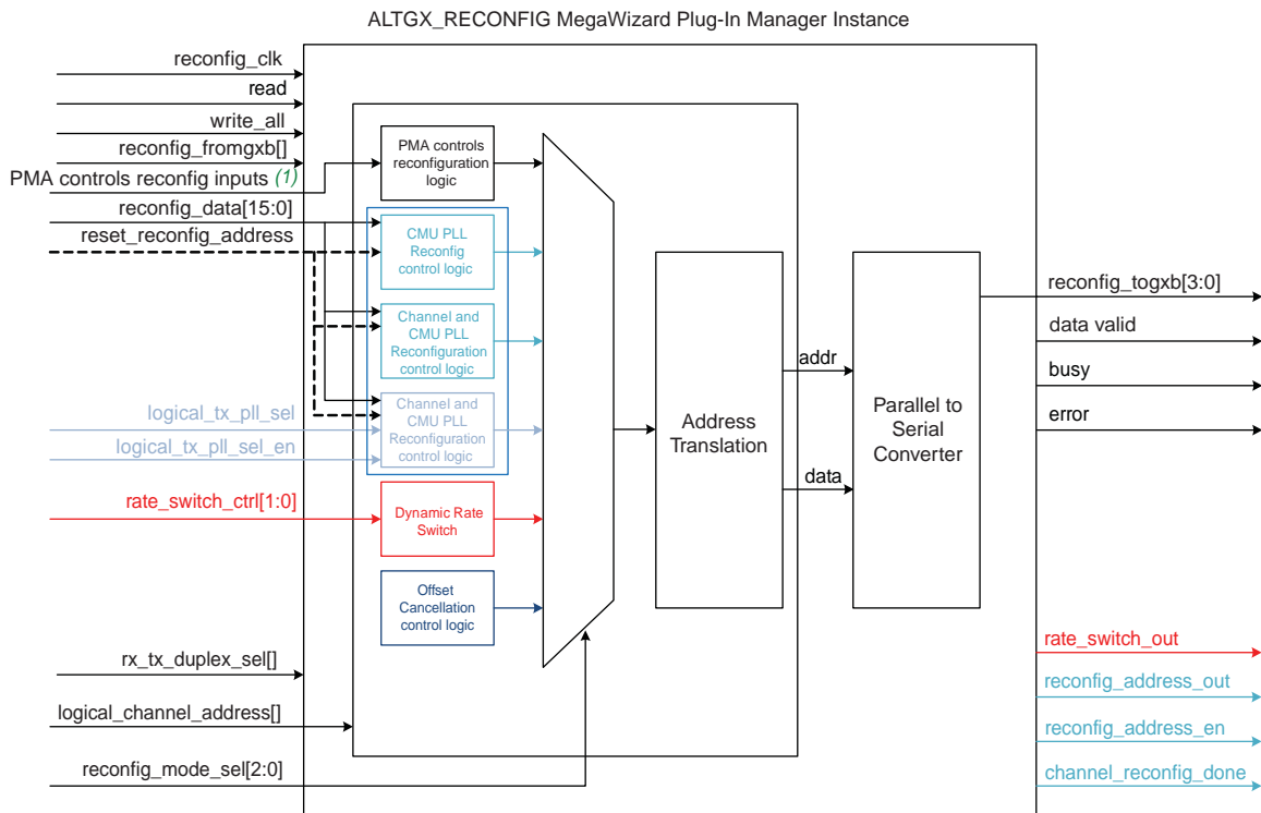
Figure 1-6. Block Diagram of the Dynamic Reconfiguration Controller
