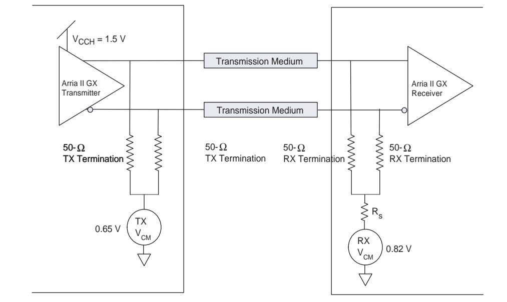
Figure 1-33. Arria II GX Transmitter (PCML) to Arria II GX Receiver (PCML) DC-Coupled Link
