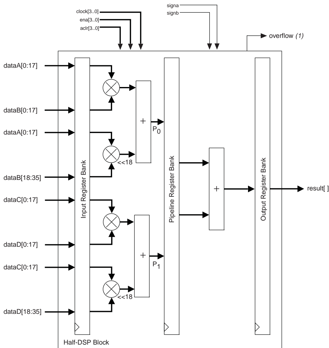
Figure 4-14. High-Precision Multiplier Adder Configuration for Half-DSP Block
