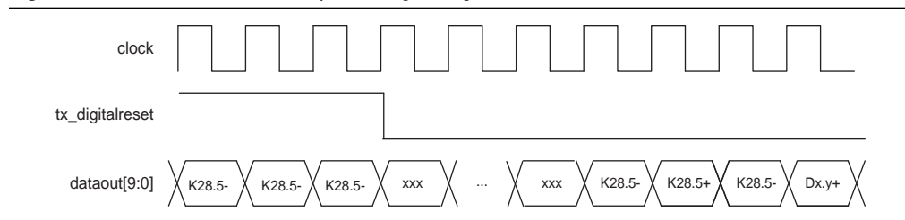
Figure 1-20. 8B/10B Encoder Output during tx\_digitalreset Assertion
