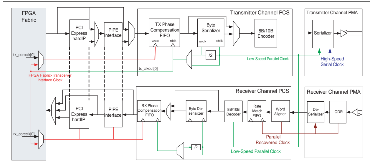
Figure 1-73. Arria II GX Transceiver Datapath in PCI Express (PIPE) Mode
