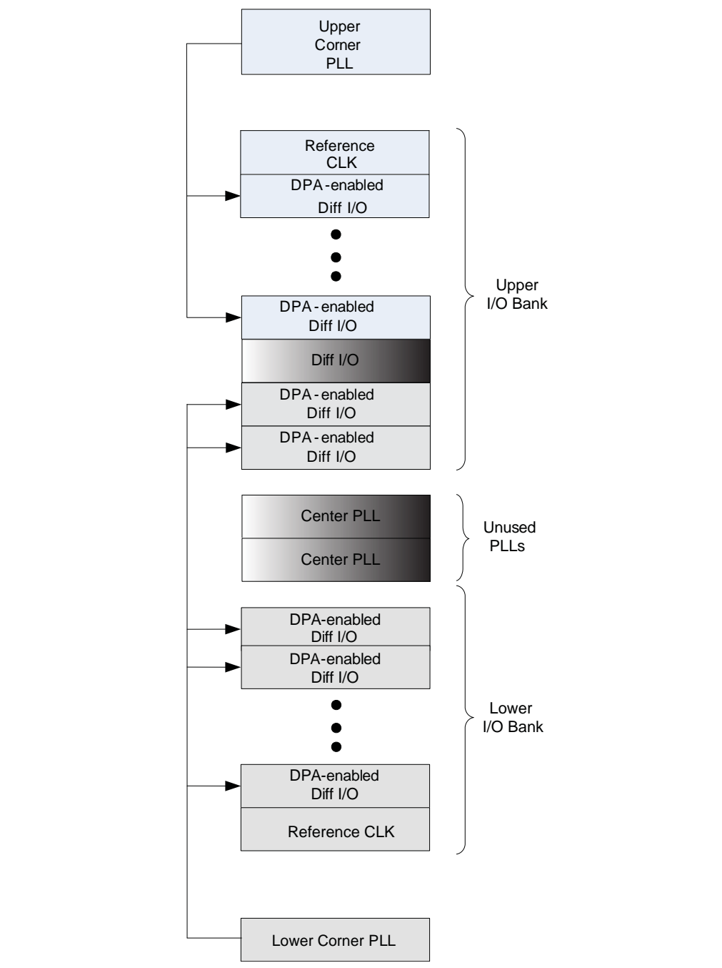
Figure 8-24. Corner PLLs Driving DPA-Enabled Differential I/Os
