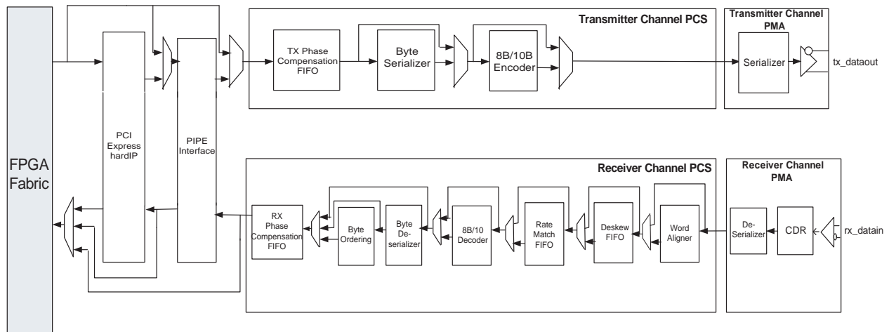
Figure 1-12. Arria II GX Transceiver Datapath
