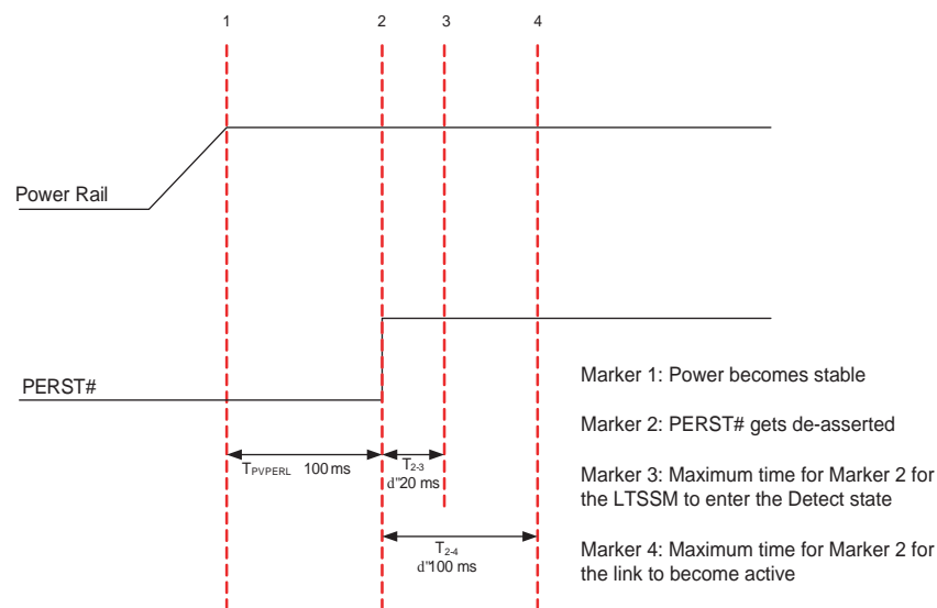
Figure 1-80. PCI Express Cold Reset Requirements
