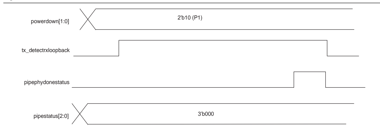
Figure 1-76. Receiver Detect, Unsuccessful
