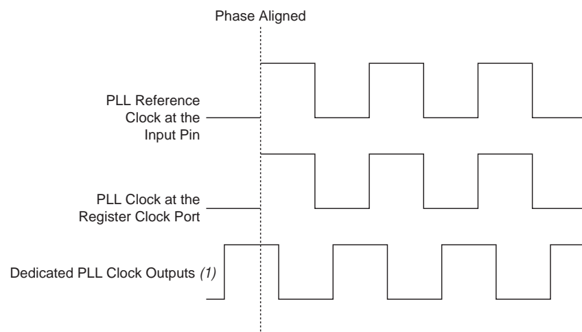
Figure 5-18. Phase Relationship Between PLL Clocks in Normal Mode
