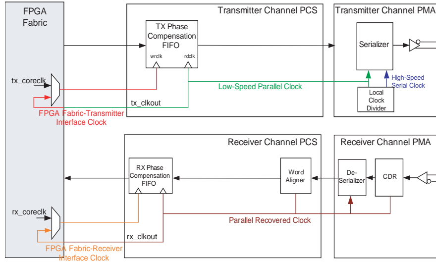
Figure 1-101. SONET/SDH OC-12 Datapath
