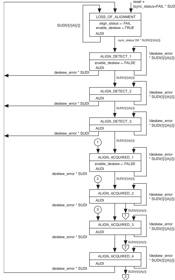
Figure 1-49. Deskew FIFO Operation in XAUI Functional Mode (Note 1)
