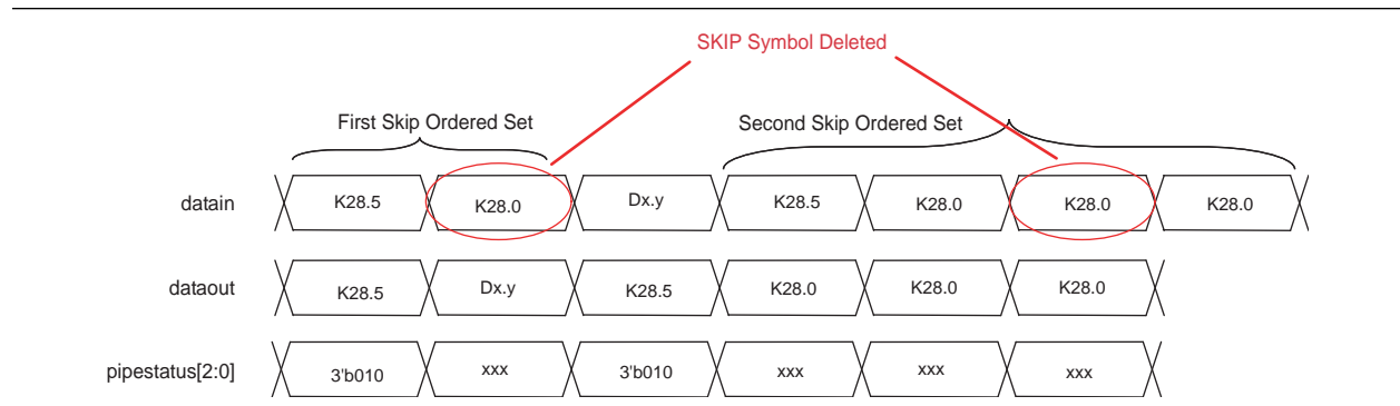
Figure 1-50. Example of Rate Match Deletion in PCI Express (PIPE) Mode
