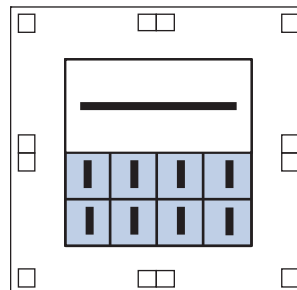
Figure 5-5. Eight Independent Sub-Regional + One Dual-Regional Clock Region (Note 1)
