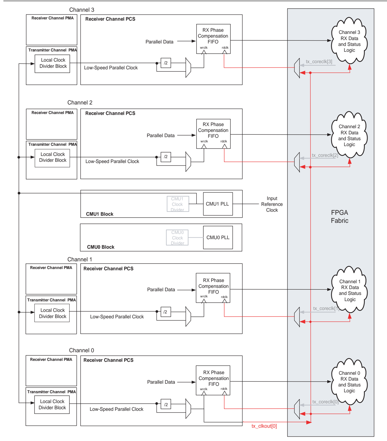
Figure 2-22. Four Identical Channels in a Transceiver Block for Example 6
