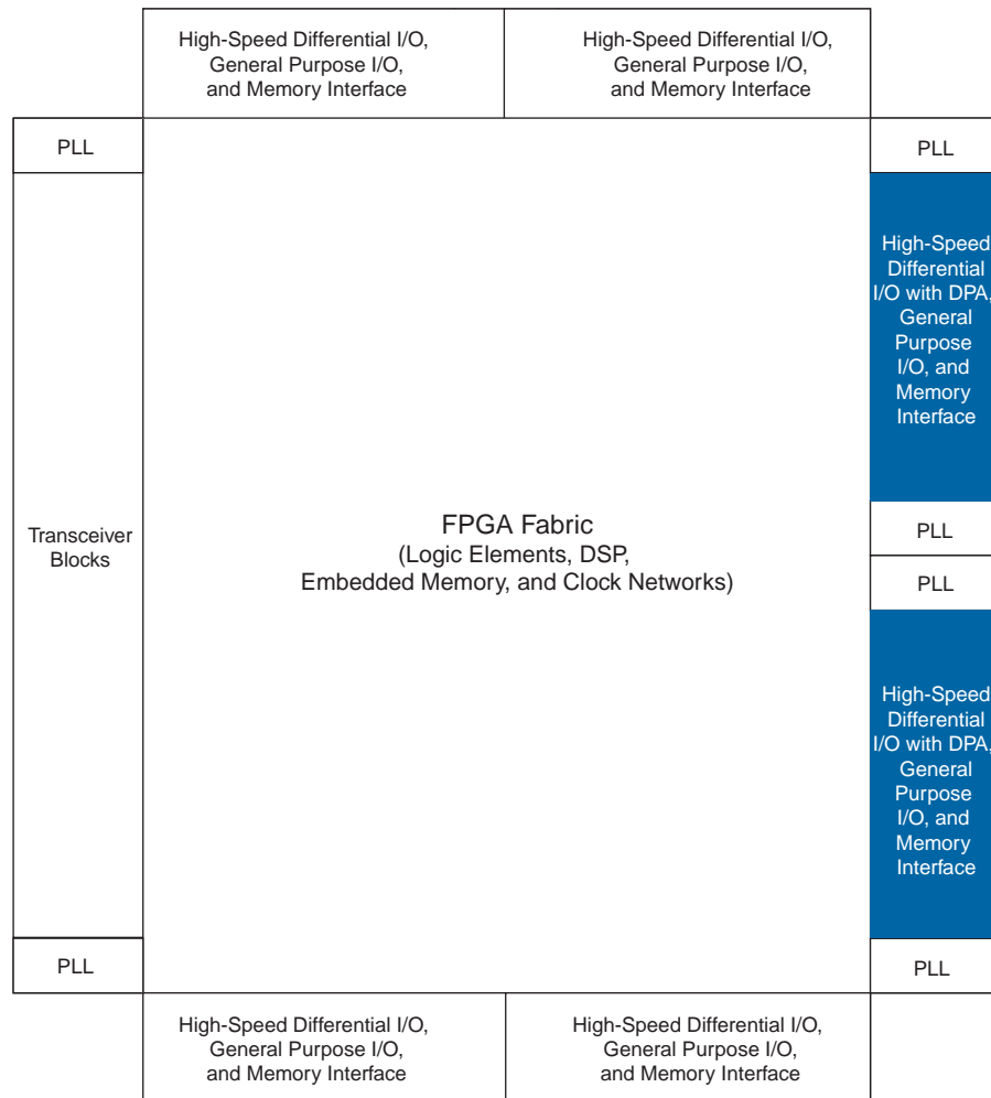
Figure 8-1. High-Speed Differential I/Os with DPA Locations in an Arria II GX Device (Note 1), (2), (3)
