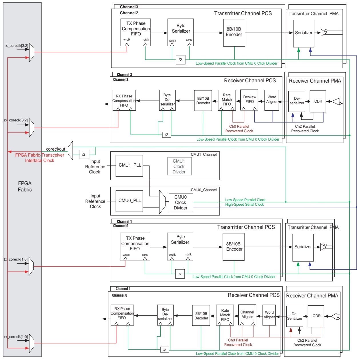
Figure 1-84. Transceiver Datapath in XAUI Mode
