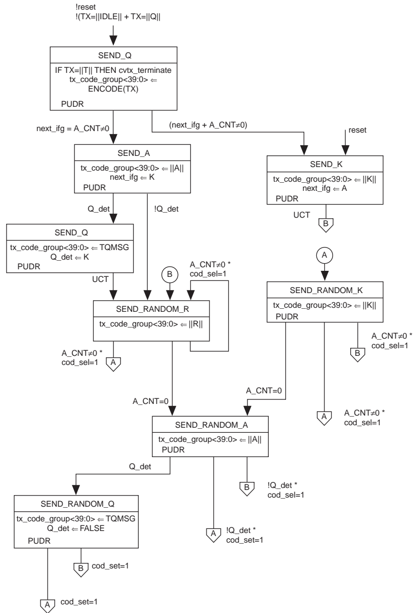
Figure 1-85. XGMII-To-PCS Code Conversion in XAU1 Mode (Note 1)
