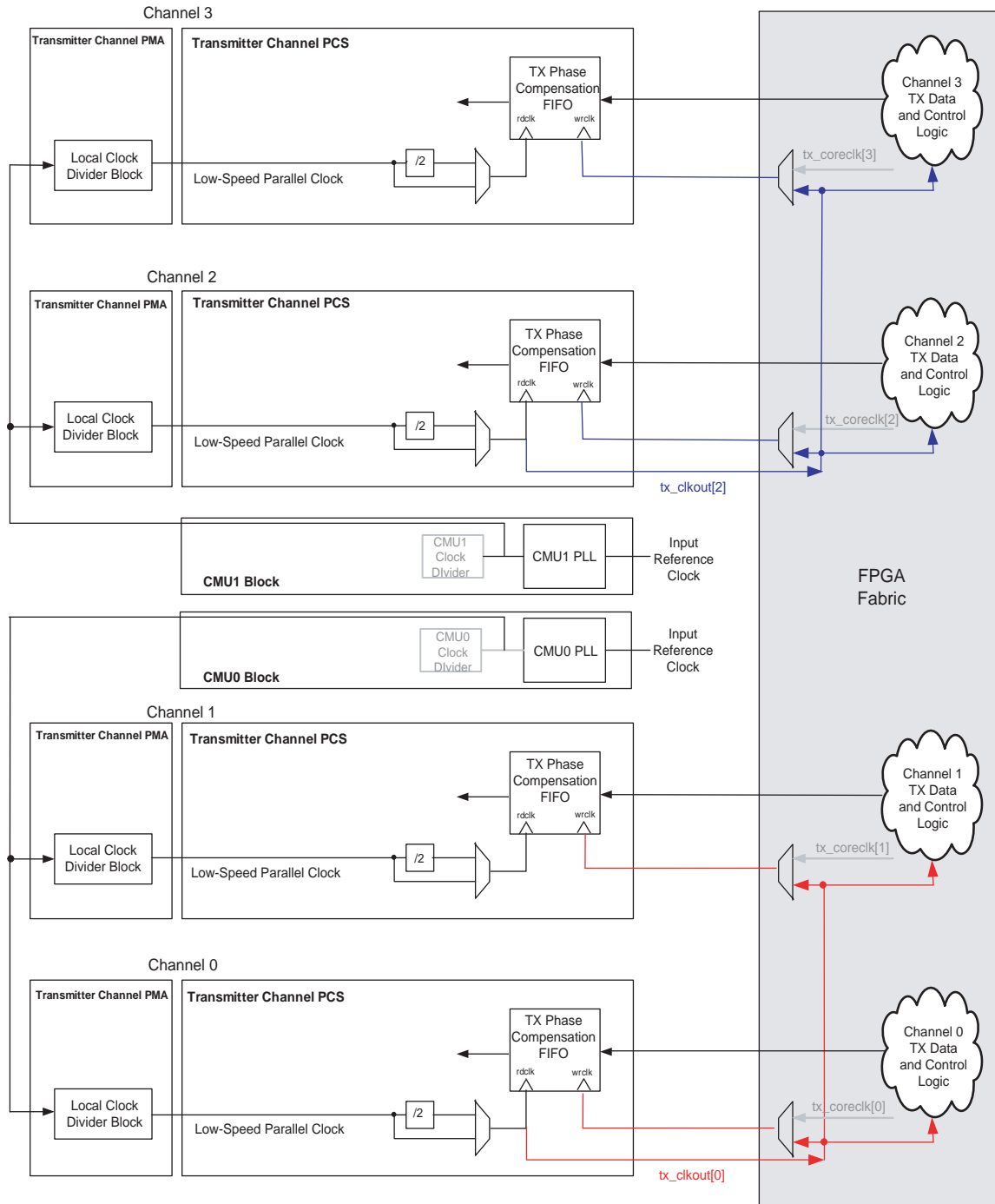
Figure 2-17. FPGA Fabric-Transmitter Interface Clocking for Example 2
