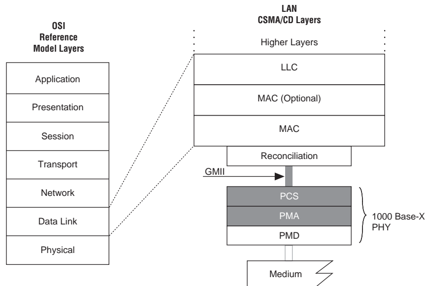
Figure 1-91. 1000 Base-X PHY in a Gigabit Ethernet OSI Reference Model
