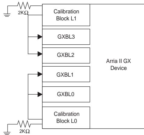
Figure 1-115. Calibration Four-Transceiver Blocks
