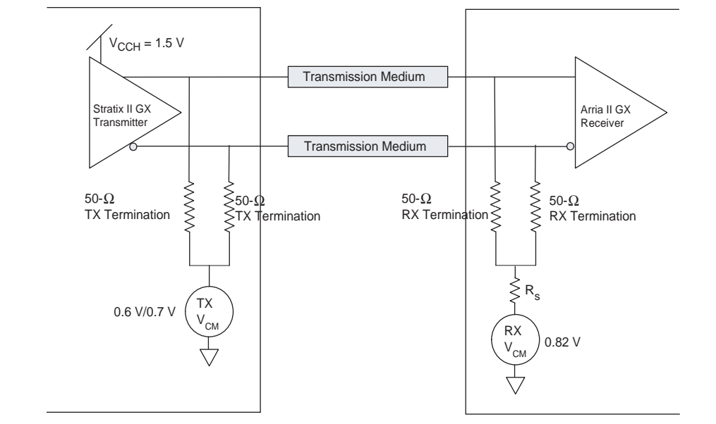
Figure 1-34. Stratix II GX Transmitter (PCML) to Arria II GX Receiver (PCML) DC-Coupled Link
