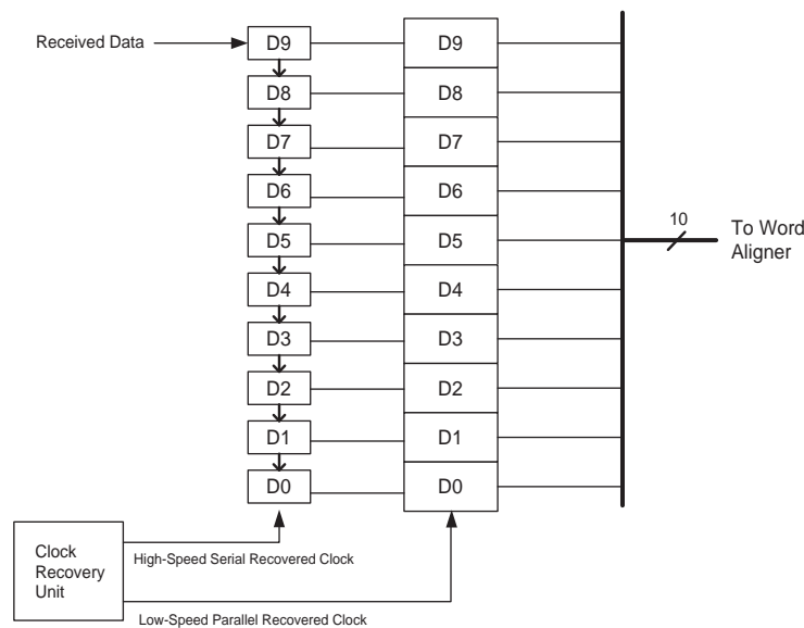
Figure 1-40. 10-Bit Deserializer Operation in Single-Width Mode
