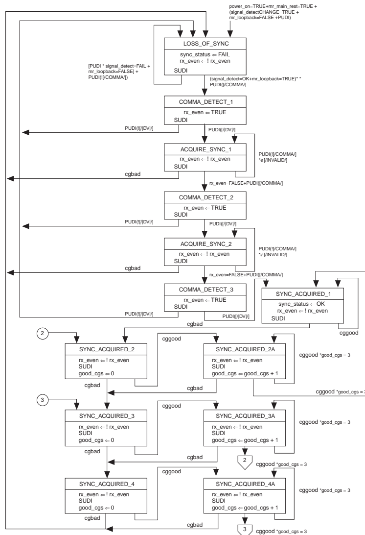
Figure 1-96. Synchronization State Machine in GIGE Mode (Note 1)
