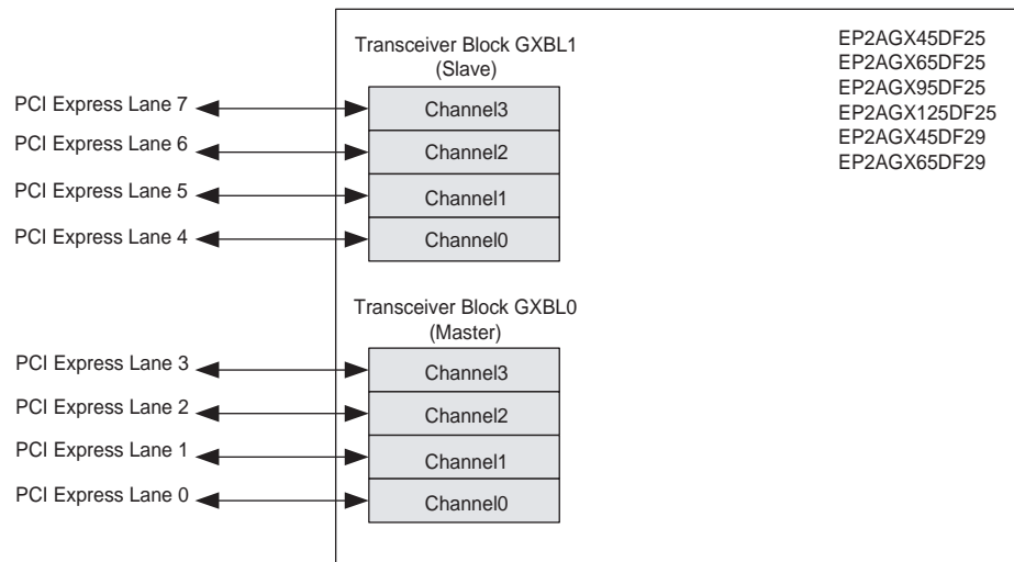
Figure 2-8. One PCI Express (PIPE) ×8 Link in Two Transceiver Block Devices
