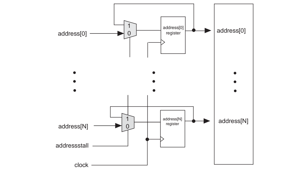
Figure 3-2. Arria II GX Address Clock Enable Block Diagram
