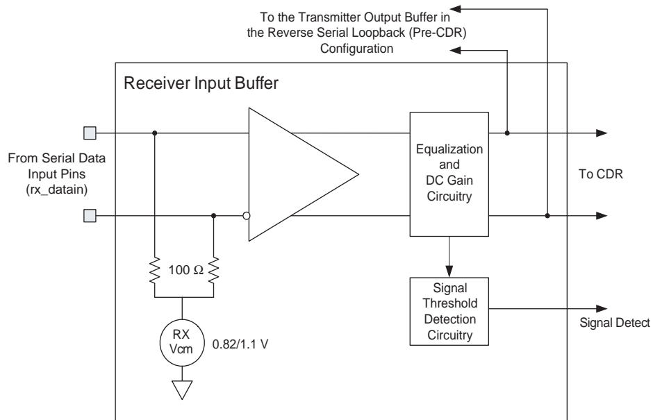
Figure 1-30. Receiver Input Buffer
