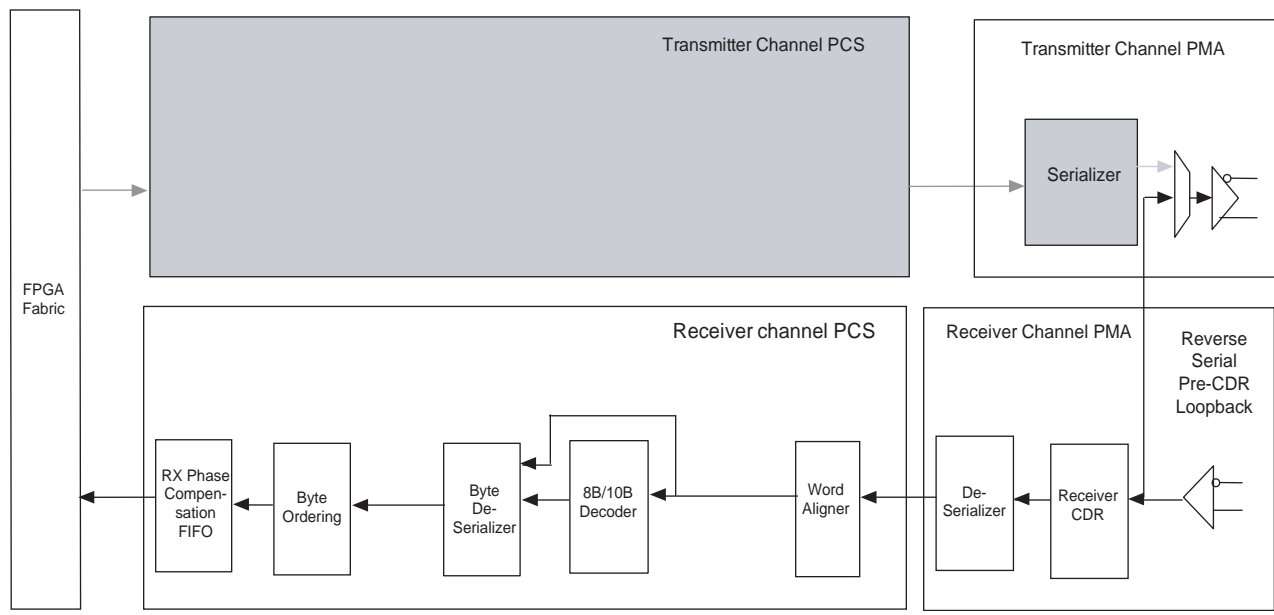
Figure 1-111. Reverse Serial Pre-CDR Loopback Datapath
