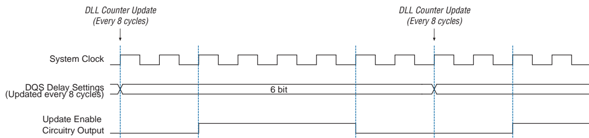
Figure 7-14. DQS Update Enable Waveform
