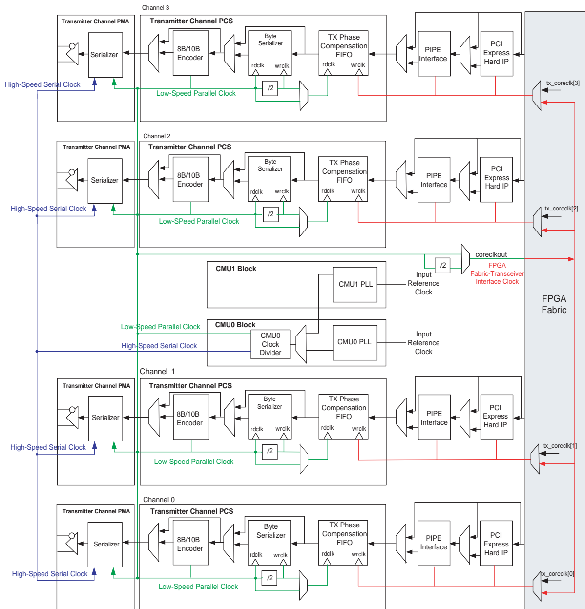
Figure 2-6. Transmitter Datapath Clcking in \times 4 Bonded Configurations
