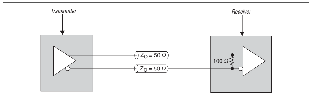
Figure 6-5. Differential Input On-Chip Termination
