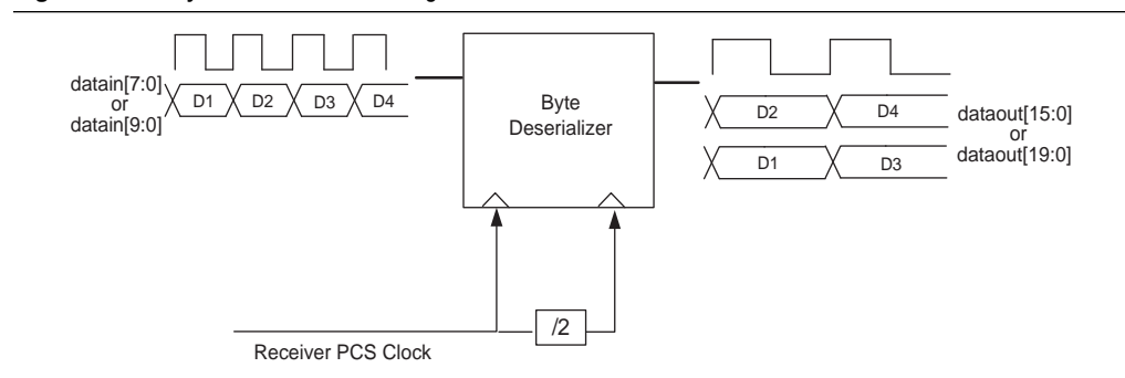
Figure 1-66. Byte Deserializer in Single-Width Mode
