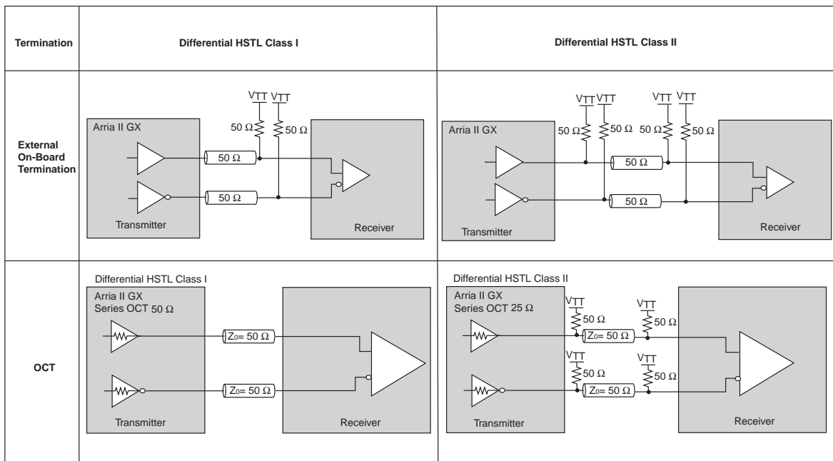
Figure 6-9. Arria II GX Differential HSTL I/O Standard Termination
