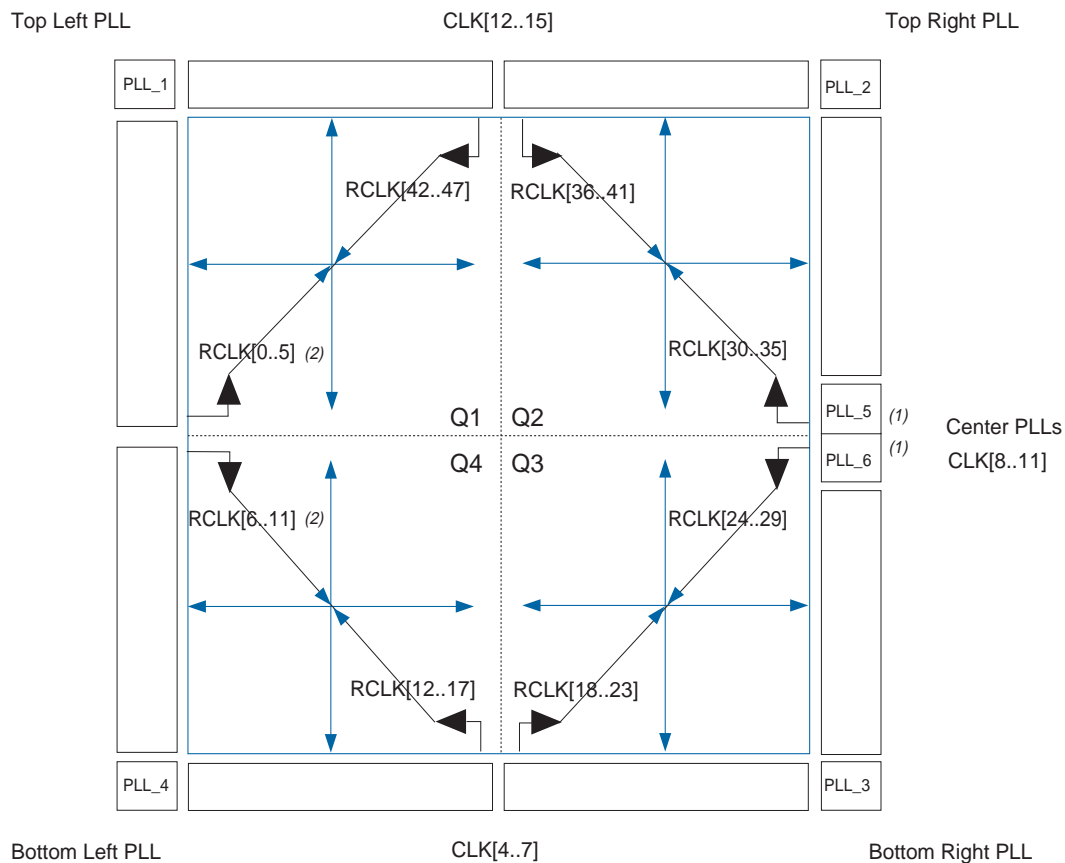
Figure 5–2. Regional Clock Networks in Arria II GX Devices
