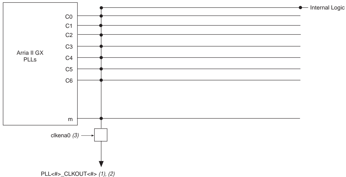
Figure 5-14. External Clock Outputs for Arria II GX PLLs
