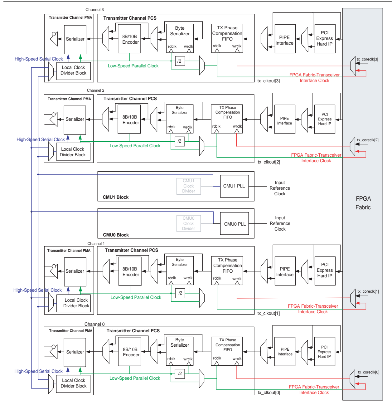
Figure 2-5. Transmitter Datapath Cloning in a Non-Bonded Configuration
