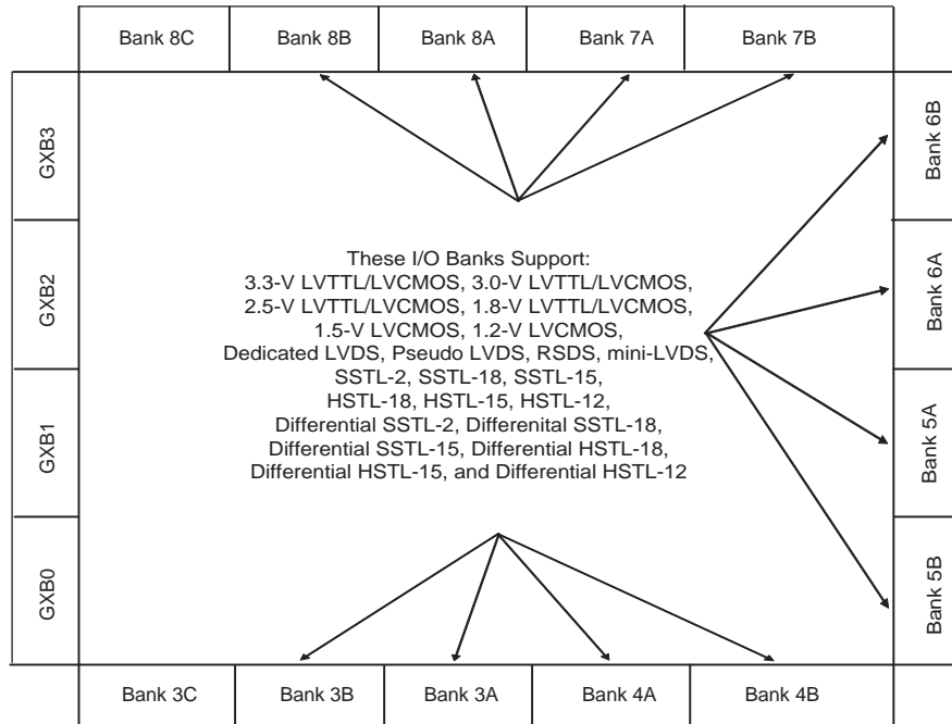
Figure 6-1. Arria II GX Devices I/O Banks (Note 1), (2), (3), (4), (5), (6)
