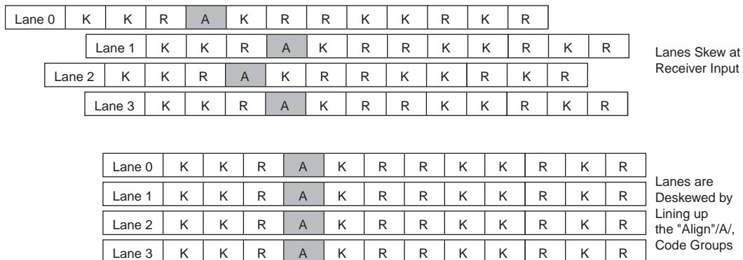
Figure 1-48. Deskew FIFO—Lane Skew at the Receiver Input
