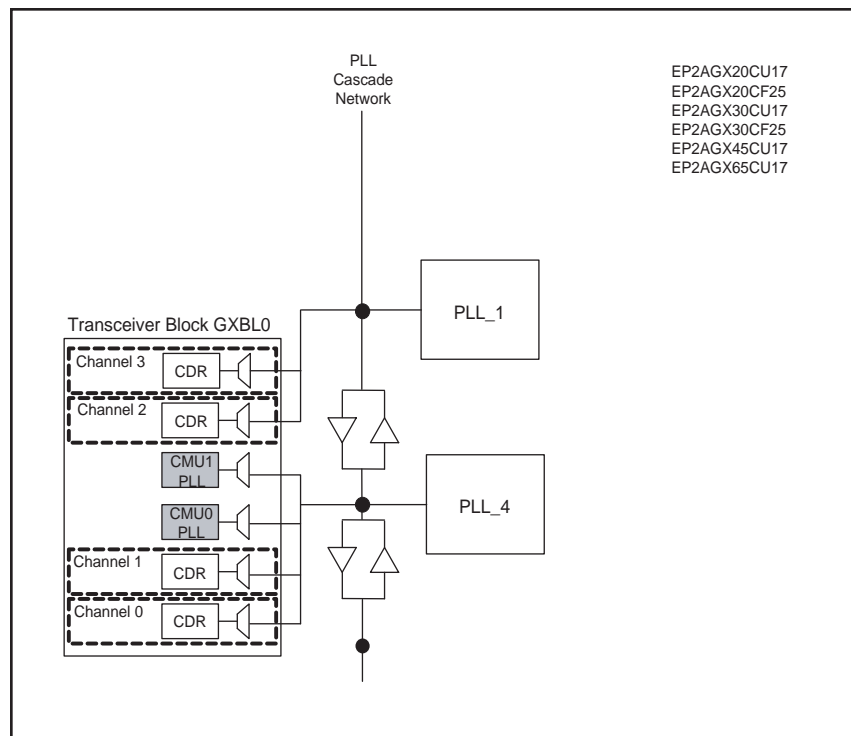
Figure 2-29. FPGA Fabric PLLs-Transceiver PLLs Cascading Option Allowed in the EP2AGX20CU17, EP2AGX20CF25, EP2AGX30CF25, EP2AGX45CU17, and EP2AGX65CU17 Devices
