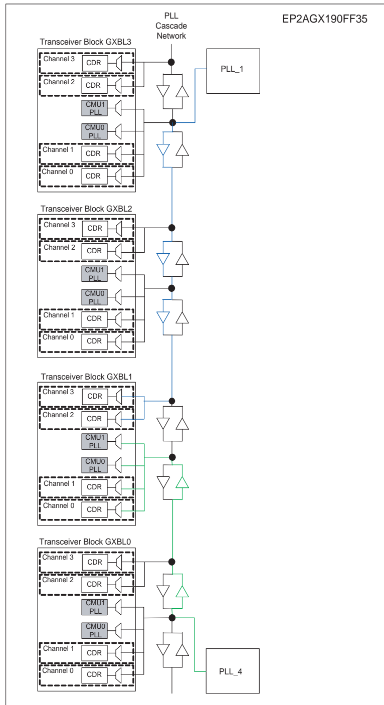
Figure 2-34. Legal FPGA Fabric-Transceiver PLL Cascading Configuration
