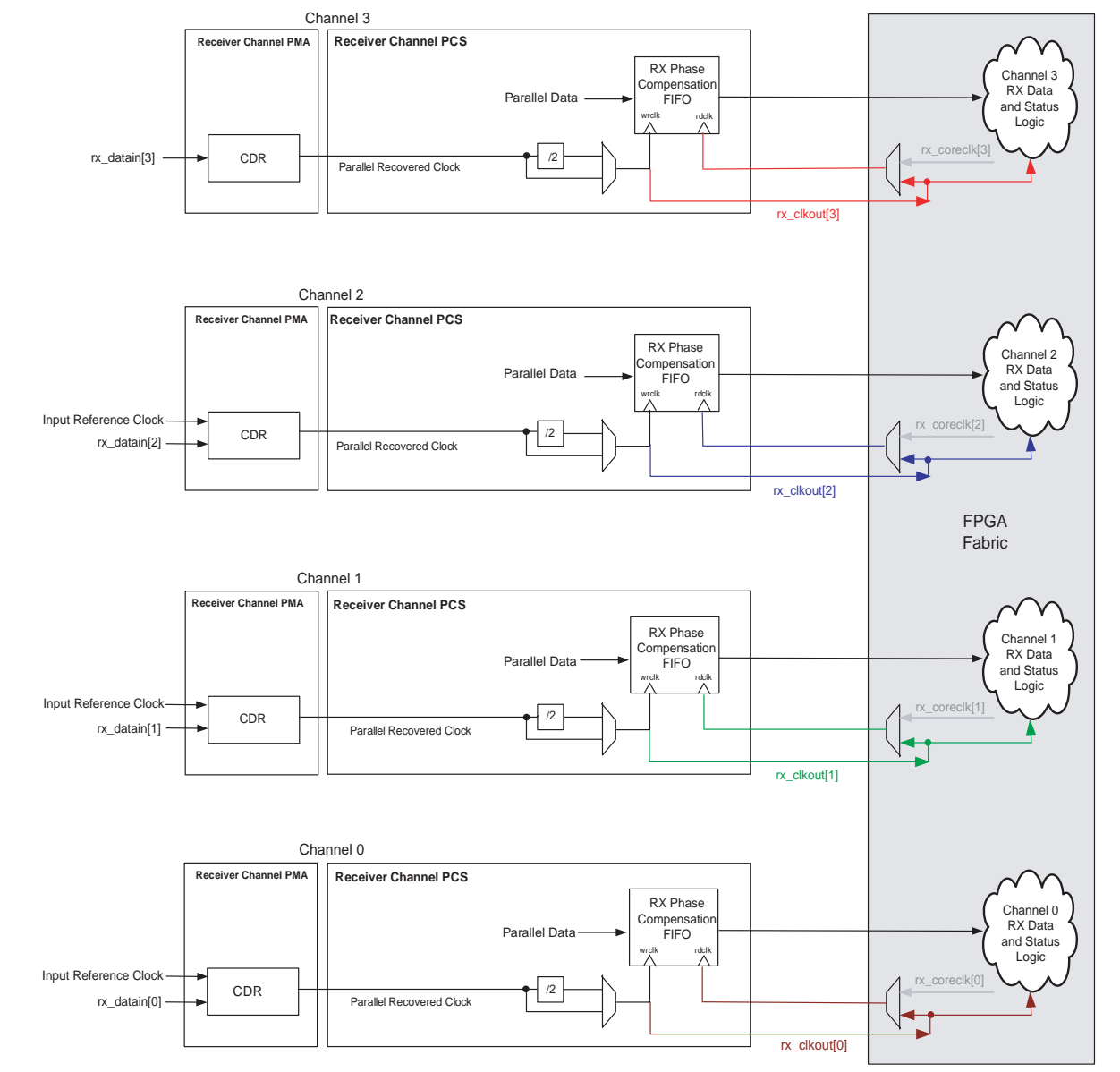
Figure 2-24. FPGA Fabric-Receiver Interface Clocking for Non-Bonded Channel Configurations without Rate Matcher
