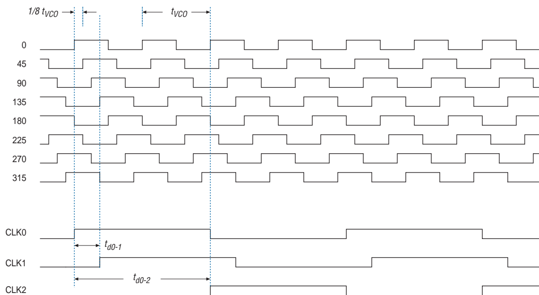
Figure 5–21. Delay Insertion Using VCO Phase Output and Counter Delay Time
