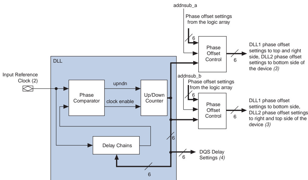
Figure 7-12. Simplified Diagram of the DQS Phase-Shift Circuitry (Note 1)
