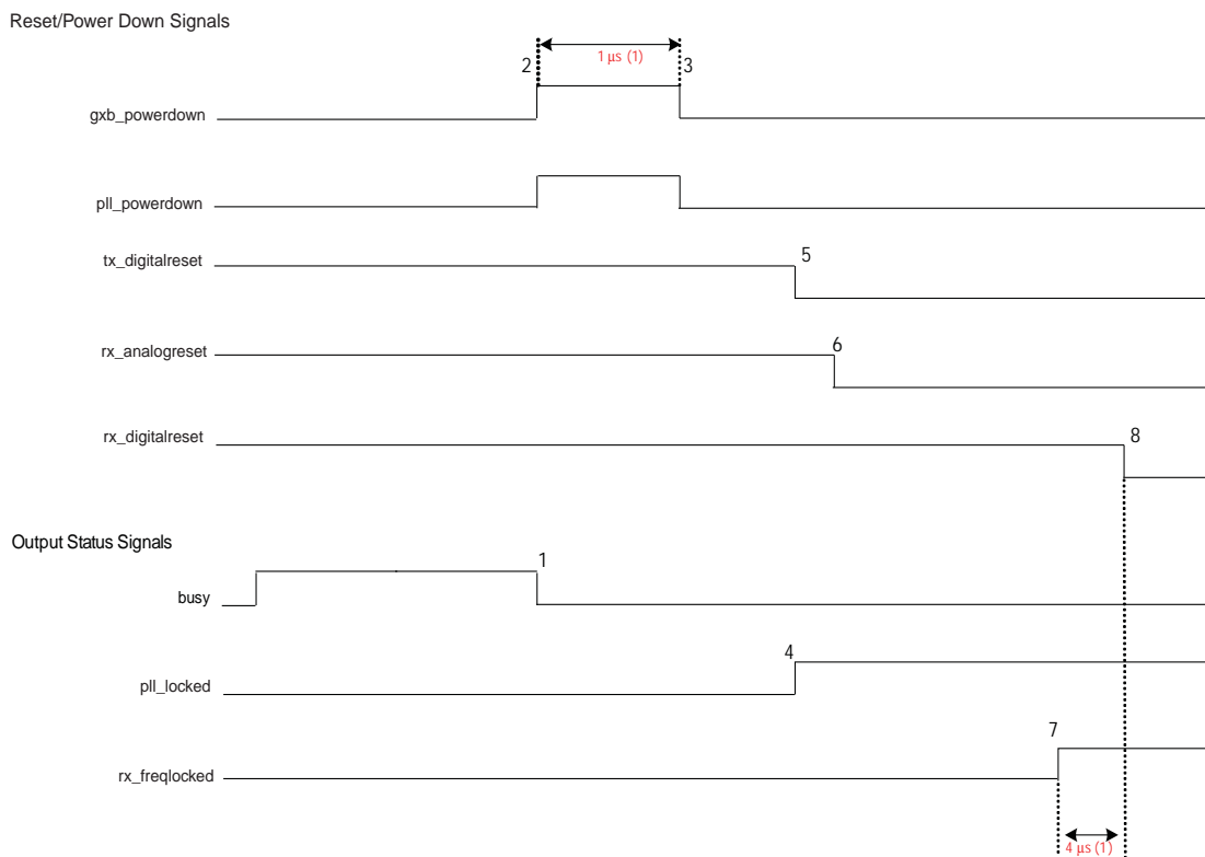
Figure 4-13. Sample Reset Sequence of Four Receiver and Transmitter Channels—Receiver CDR in Automatic Lock Mode with Optional gxb_powerdown Signal
