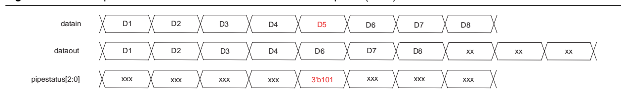
Figure 1-52. Example of Rate Match FIFO Full Condition in PCI Express (PIPE) Mode
