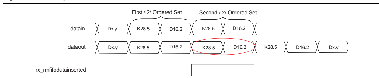
Figure 1-98. Example of Rate Match Insertion in GIGE Mode
