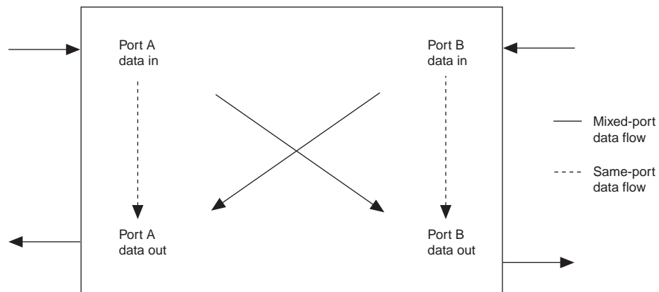
Figure 3-13. Arria II GX Read-During-Write Data Flow
