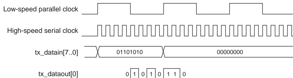
Figure 1-25. Serializer Bit Order (Note 1)
