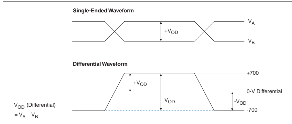
Figure 1-27. V_{OD} (Differential) Signal Level
