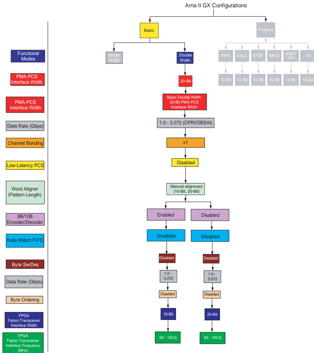
Figure 1-71. Transceiver Configurations in Basic Double-Width Mode with a 20-Bit Wide PMA-PCS Interface
