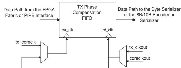
Figure 1-15. TX Phase Compensation FIFO
