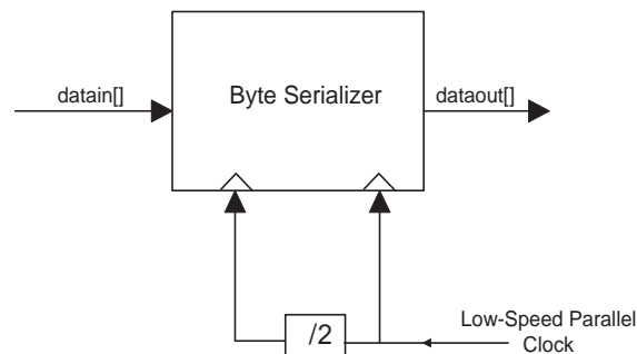
Figure 1–16. Byte Serializer Datapath in Single-Width Mode (Note 1), (2)
