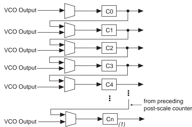
Figure 5-20. Counter Cascading
