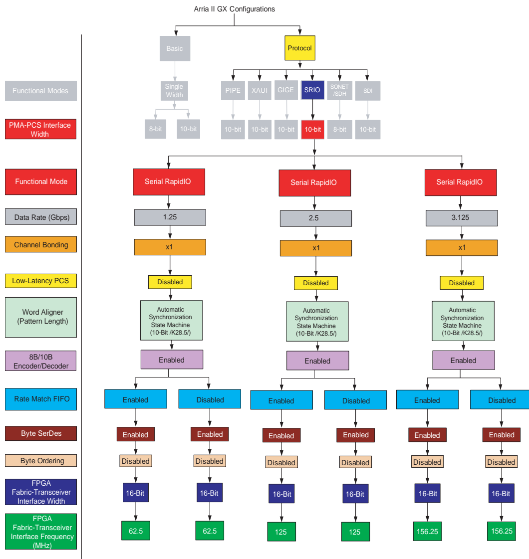
Figure 1-107. Serial RapidIO Mode
