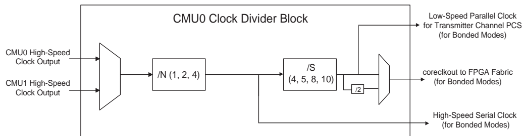
Figure 1-10. Diagram of the CMUO Clock Divider Block
