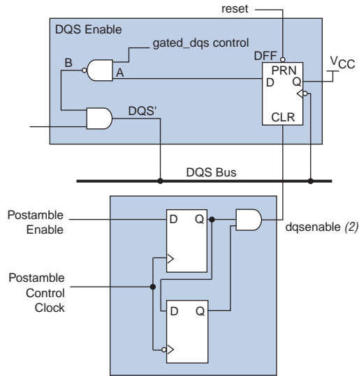
Figure 7-15. Arria II GX DQS Postamble Circuitry (Note 1)
