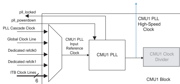
Figure 1-11. CMU1 Block (Grayed Area Shows the Inactive Block)
