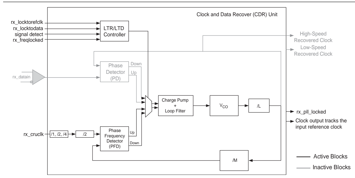
Figure 1-38. CDR in Lock-To-Reference Mode
