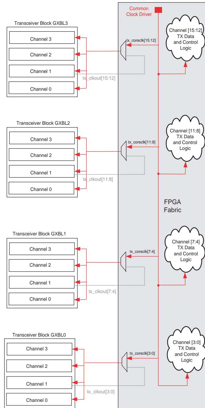
Figure 2–20. Sixteen Identical Channels across Four Transceiver Blocks for Example 4
