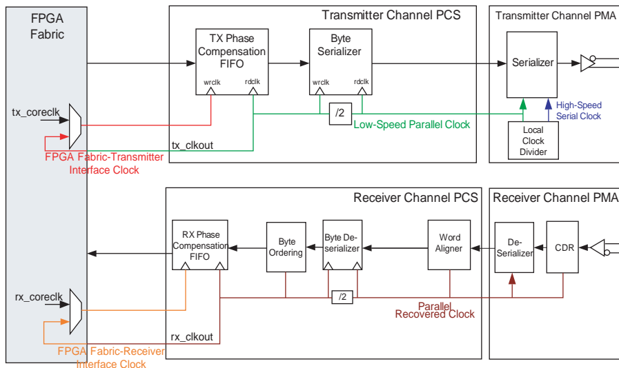
Figure 1-102. SONET/SDH OC-48 Datapath
