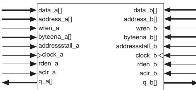
Figure 3-10. Arria II GX True Dual-Port Memory (Note 1)
