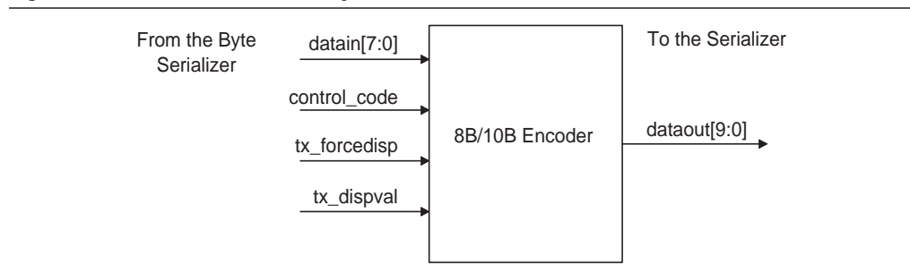
Figure 1-17. 8B/10B Encoder in Single-Width Mode
