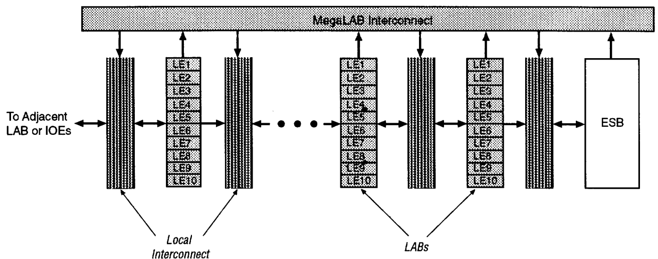
Figure 2. MegaLAB Structure
