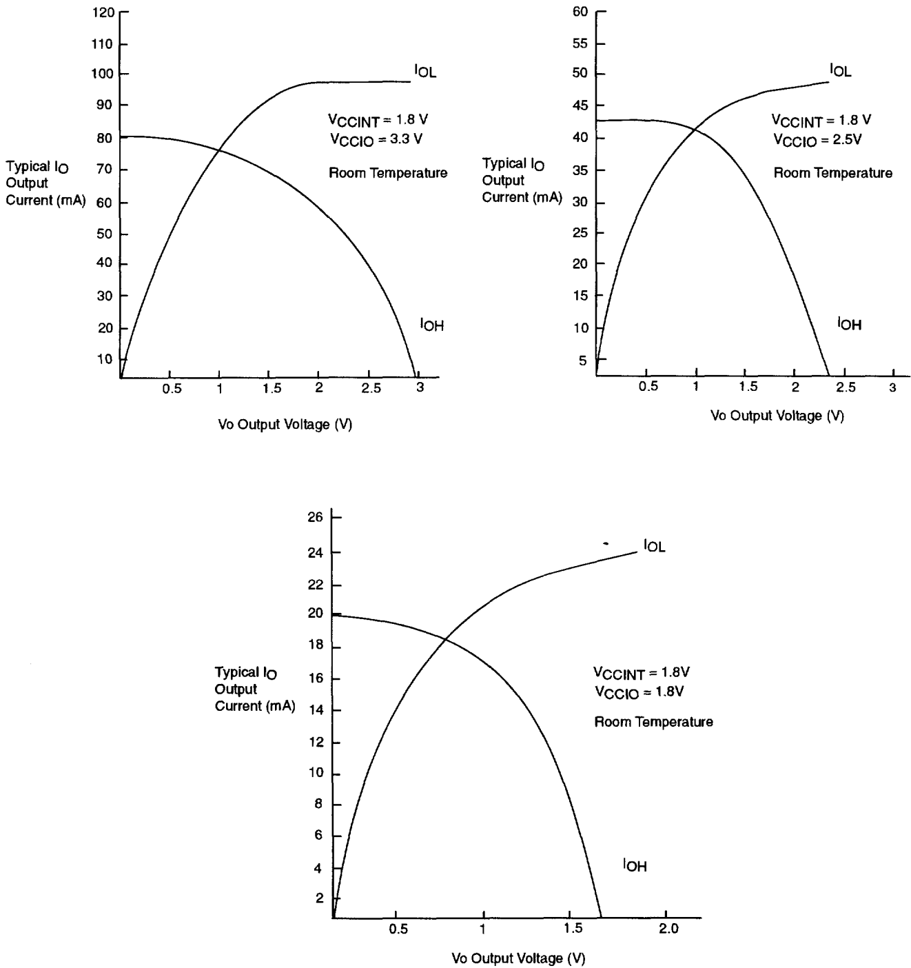
Figure 32. Output Drive Characteristics of APEX 20KC Devices
