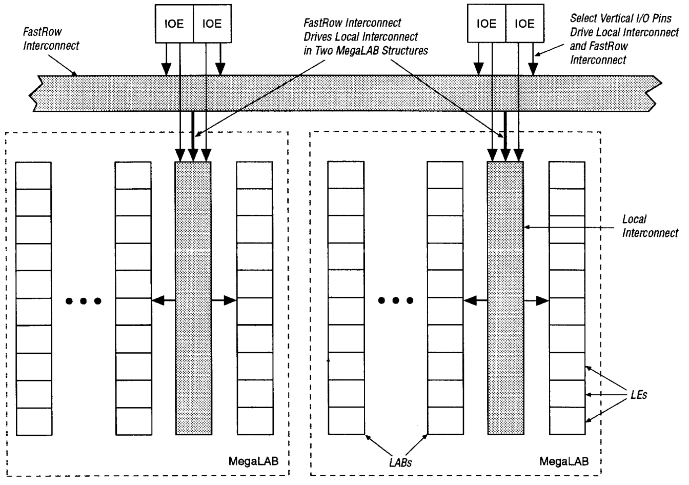
Figure 12. APEX 20KC FastRow Interconnect
