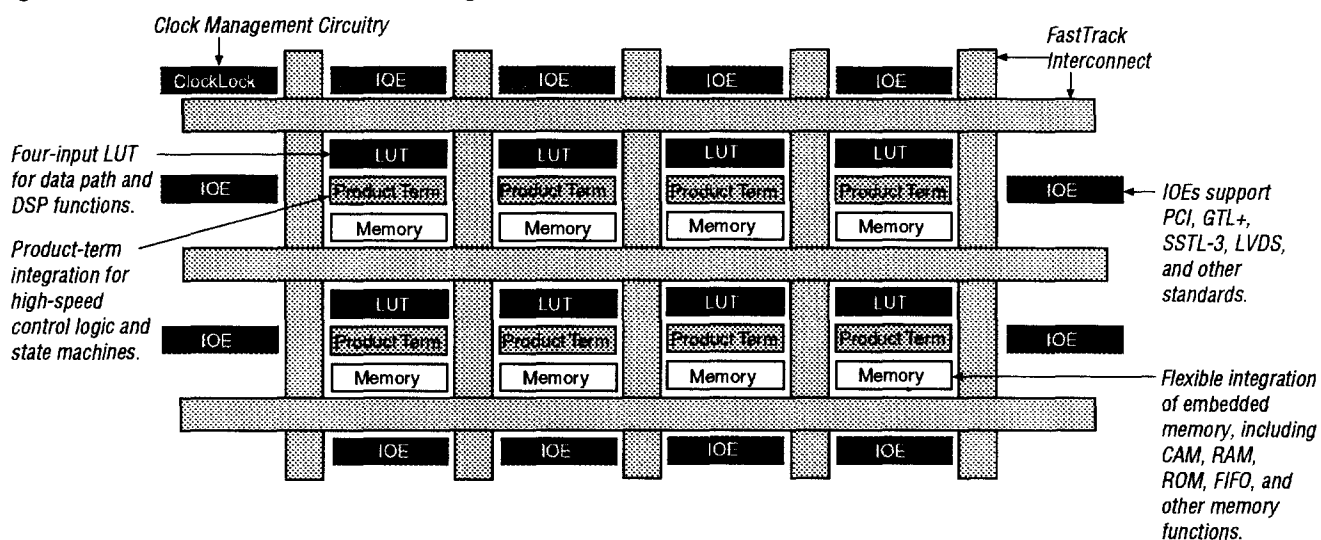
Figure 1. APEX 20KC Device Block Diagram
