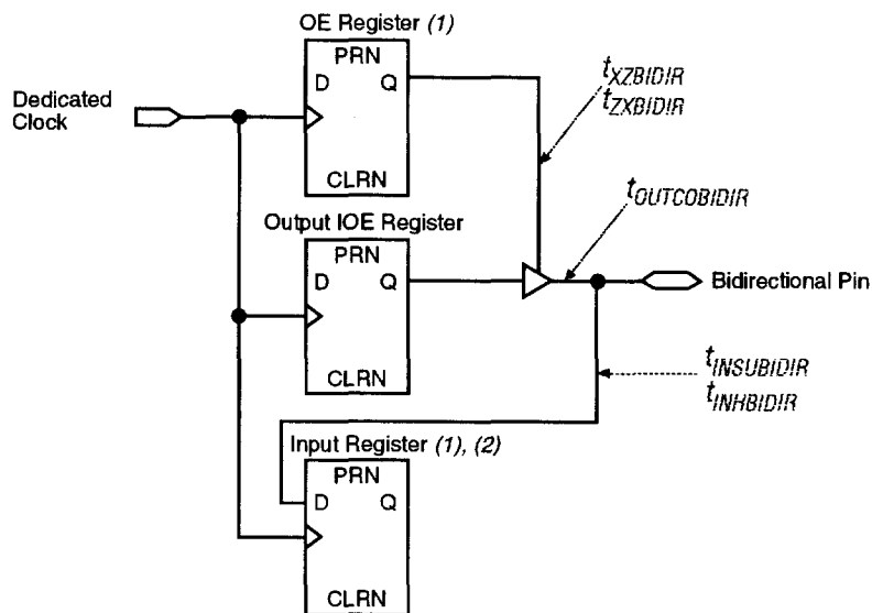
Figure 34. Synchronous Bidirectional Pin External Timing
