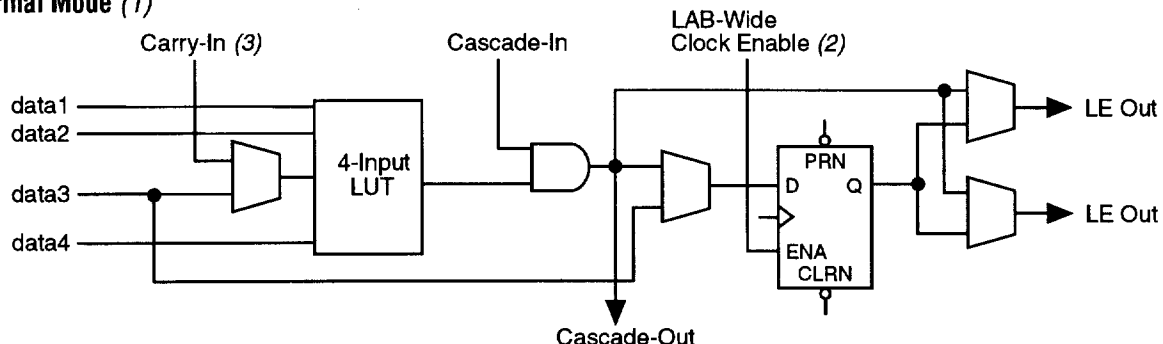
Figure 8. APEX 20KC LE Operating Modes
