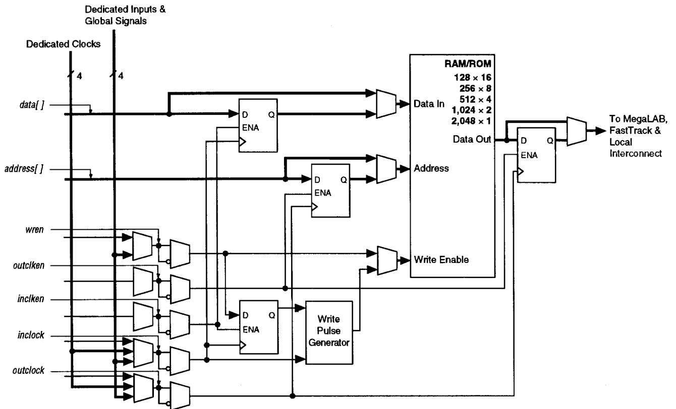
Figure 22. ESB In Single-Port Mode Note (1)
