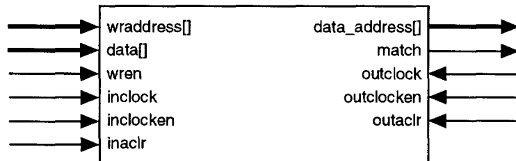
Figure 23. APEX 20KC CAM Block Diagram
