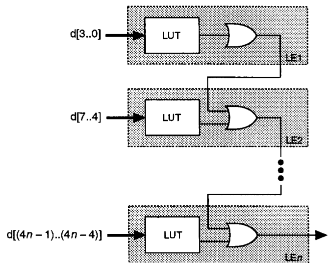
OR Cascade Chain
