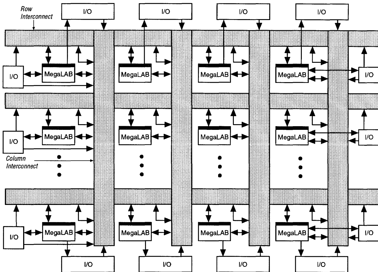
Figure 9. APEX 20KC Interconnect Structure
