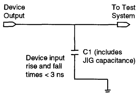
Figure 31. APEX 20KC AC Test Conditions
