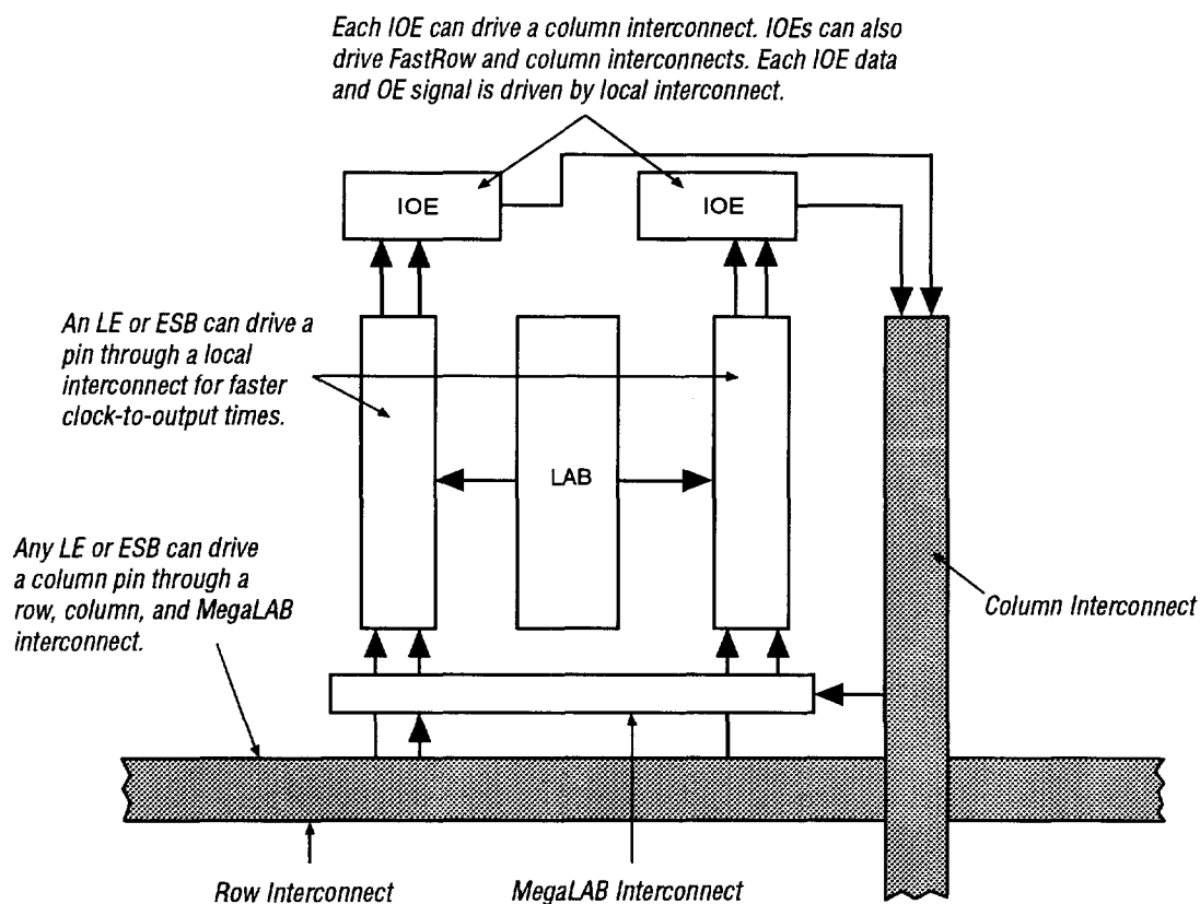
Figure 27. Column IOE Connection to the Interconnect
