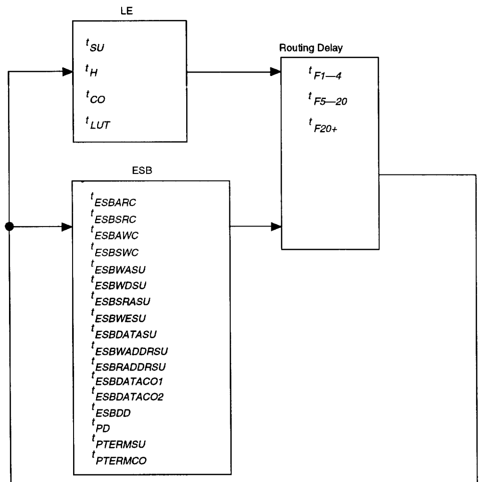
Figure 33. f_{MAX} Timing Model
