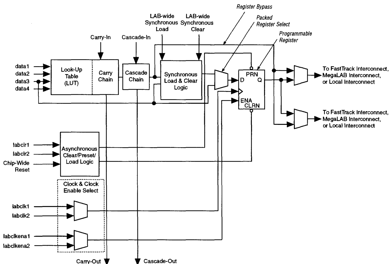
Figure 5. APEX 20KC Logic Element
