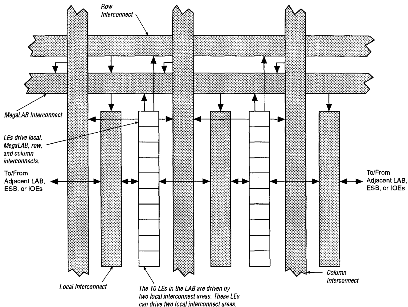
Figure 3. LAB Structure
