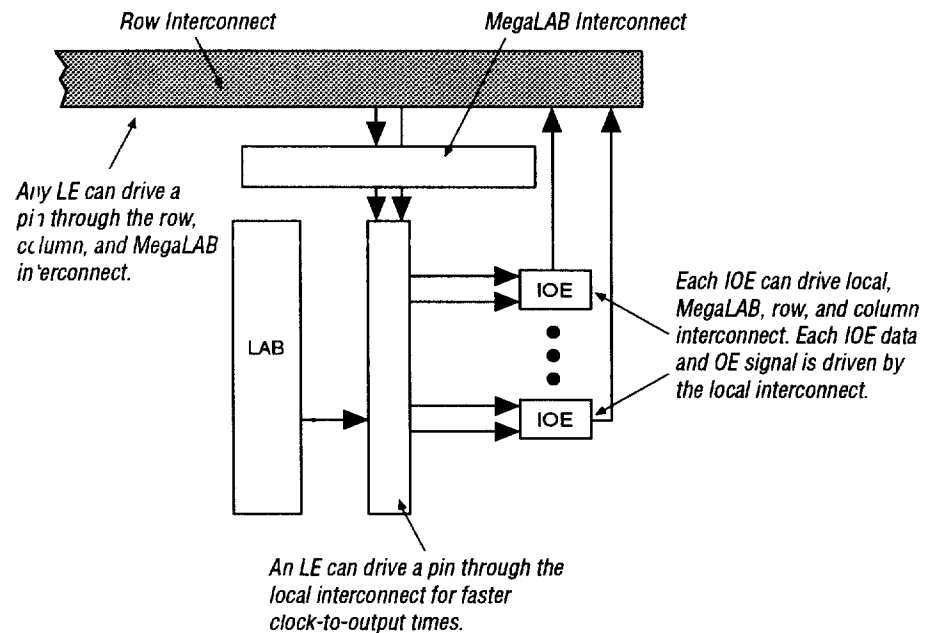
Figure 26. Row IOE Connection to the Interconnect
