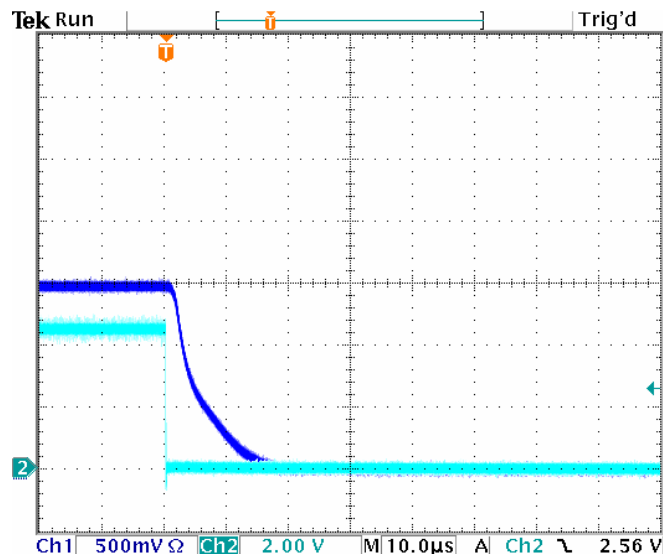
Shutdown, V_{IN} = 3.6V , V_{OUT} = 1.5V , Load = 500mA
