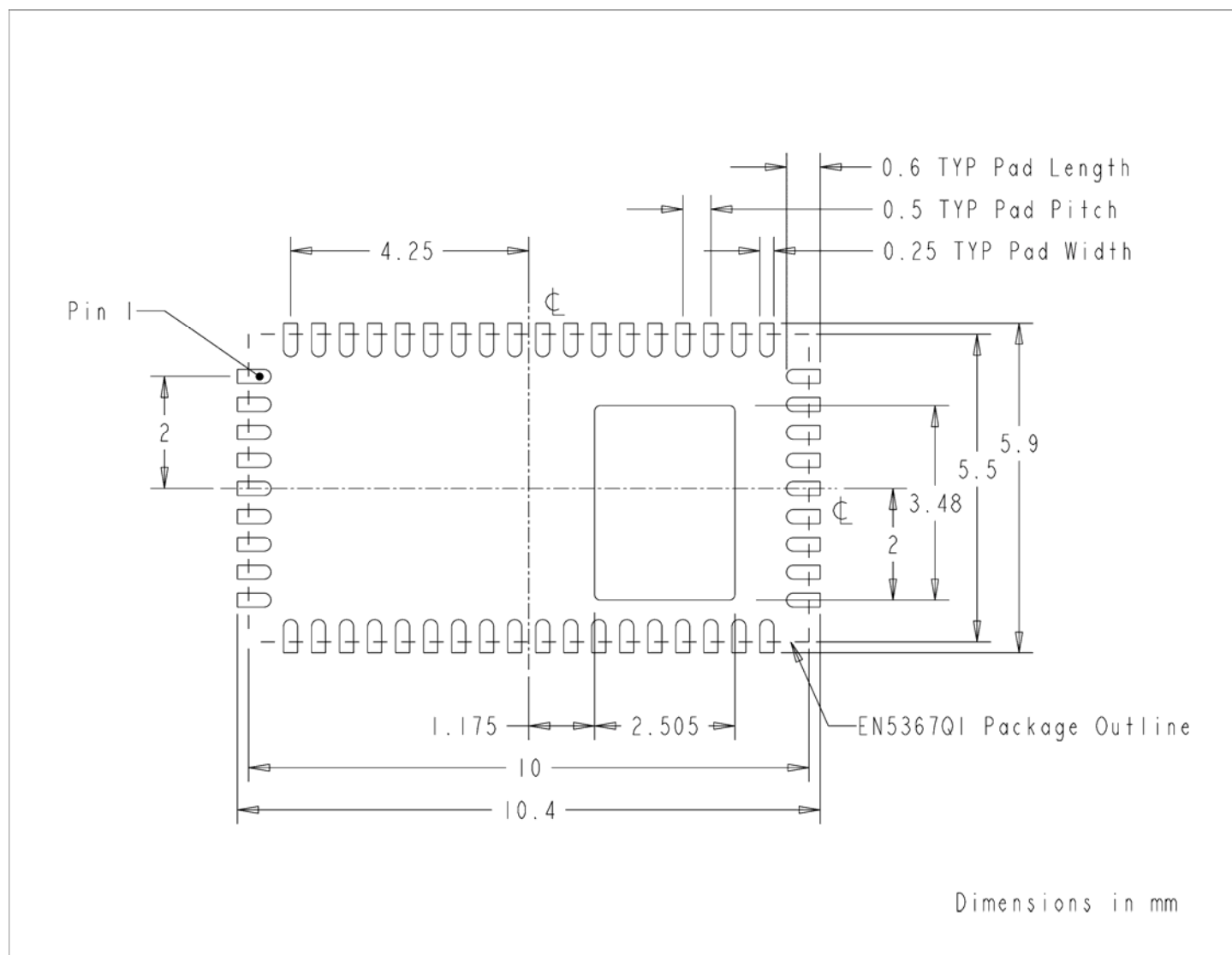
Figure 10: EN5367QI PCB Footprint (Top View)
