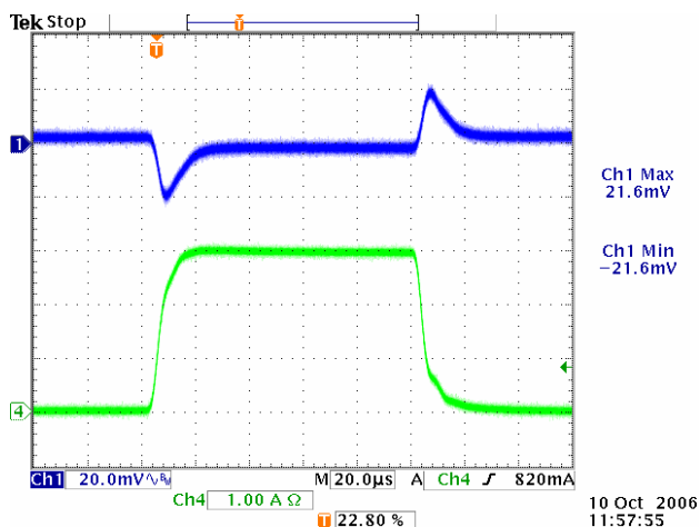
Load transient, 0 – 3A, V_{\text{IN}}/V_{\text{OUT}} = 5.5\text{V}/1.2\text{V}
