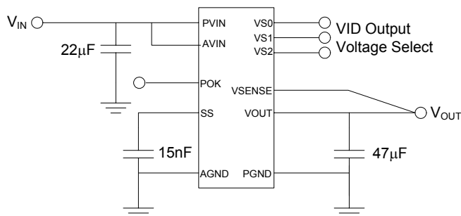
Figure 1. Simple Layout.
