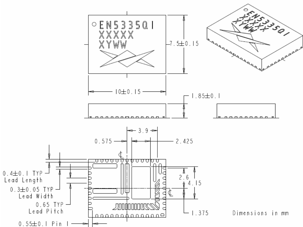
Figure 6. Package dimensions.
