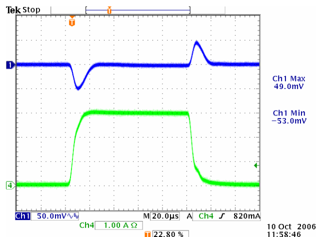
Load transient, 0 – 3A, V_{\text{IN}}/V_{\text{OUT}} = 5.5\text{V}/3.3\text{V}
