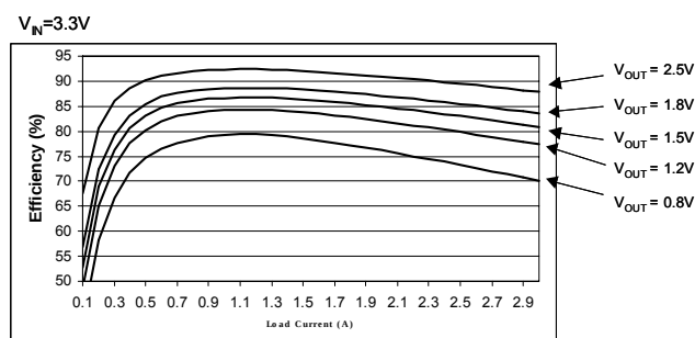
Efficiency versus Load, V_{\text{IN}} = 3.3\text{V}
