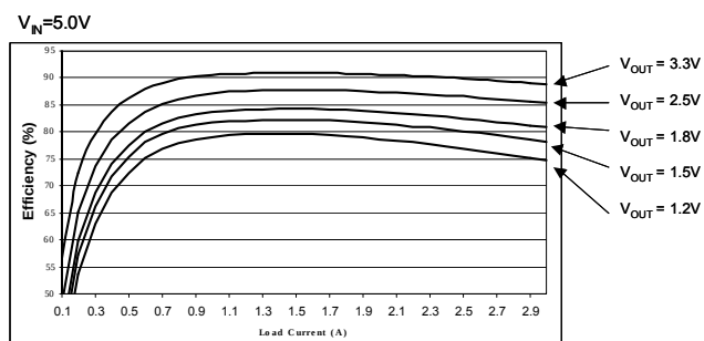
Efficiency versus Load, V_{\text{IN}} = 5.0\text{V}
