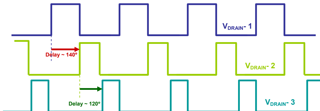
Figure 7: Example of a possible way to synchronize and use delays advantageously to minimize input ripple. R1 ~ 39kΩ, R2 ~ 33kΩ. (Refer to Figure 6 for R1 and R2.) R3 does not matter in this case.
