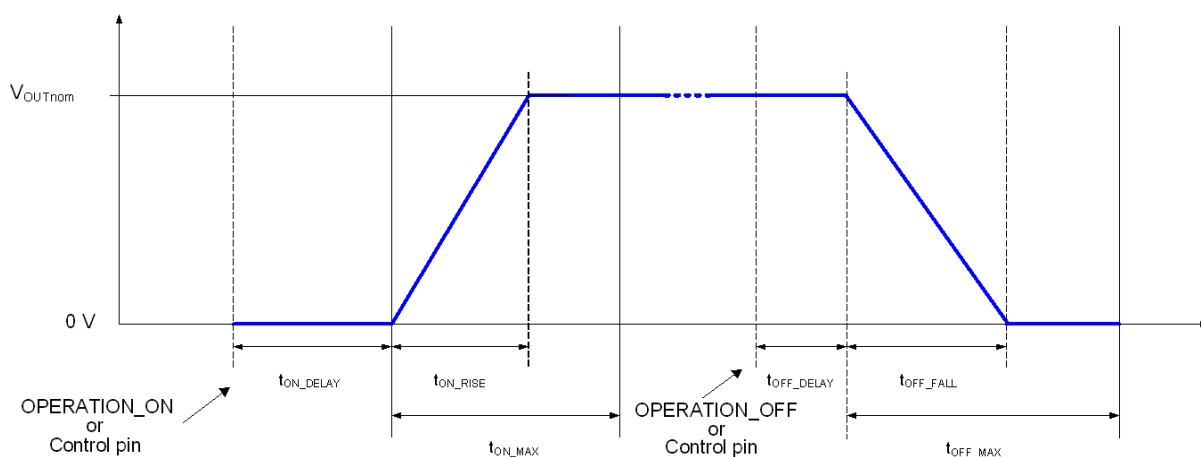
Figure 6: Power Sequencing
