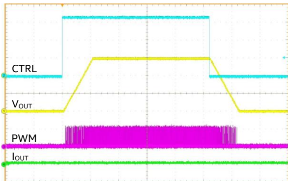
Start-up/Shutdown, CTRL At No Load, 5 ms/div
