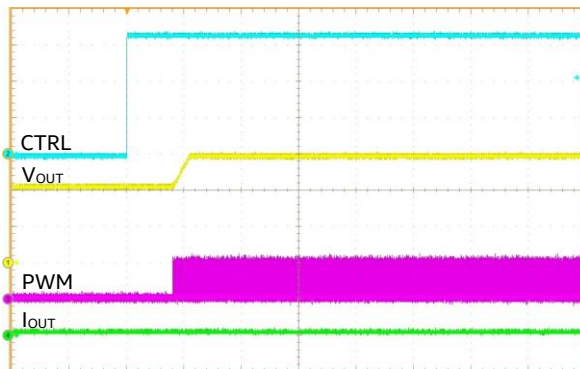
Start-up Into 0.6V Pre-Bias With CTRL, 5 ms/div
