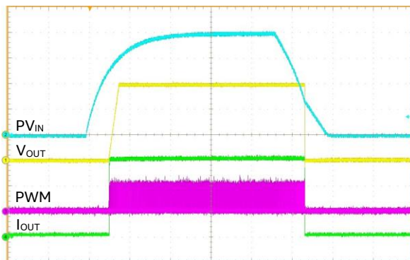
Start-up/Shutdown, PVIN At 30A Load, 20 ms/div
