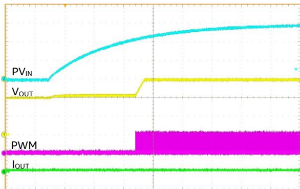
Start-up Into 0.6V Pre-Bias With PVIN, 5 ms/div
