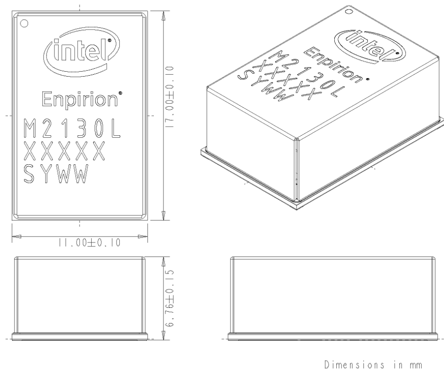
Figure 23: Package Dimensions
