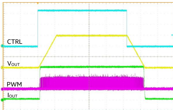
Start-up/Shutdown, CTRL At 30A Load, 5 ms/div
