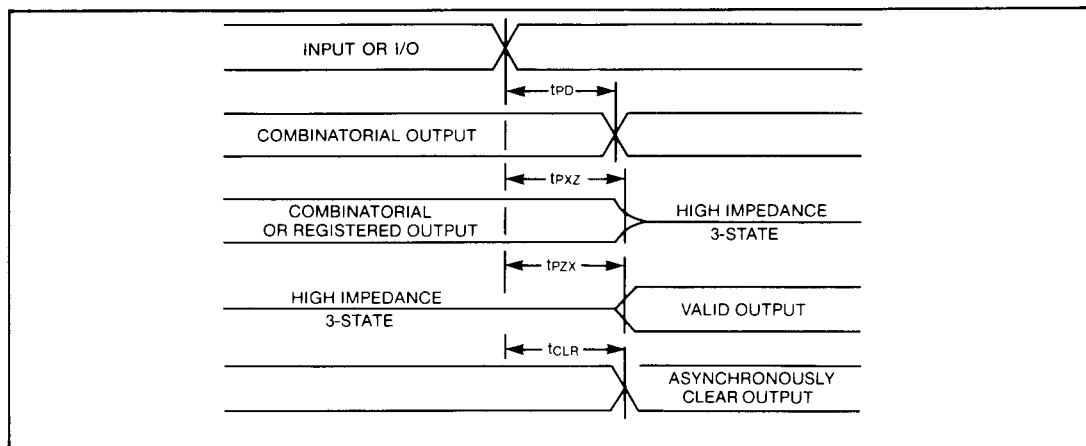
Figure 5. Switching Waveforms
