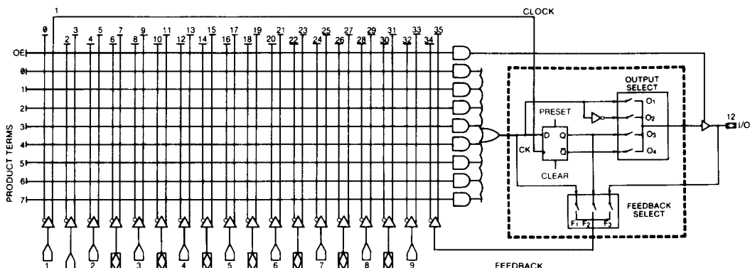
Figure 2. EP310 Macrocell
