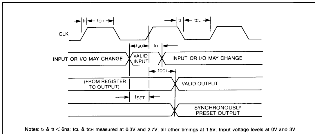
Figure 6. AC Test Conditions
