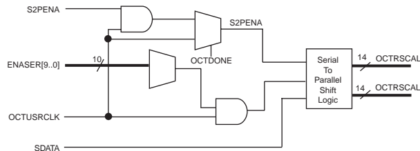
Figure 7–20. OCT Calibration Block
