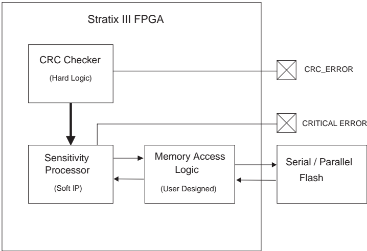
Figure 15-1. Critical Error Detection Implementation Block Diagram
