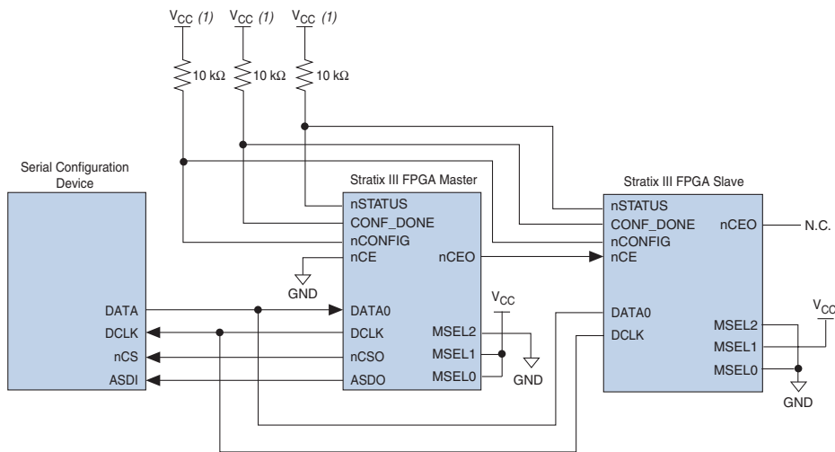
Figure 11–13. Multi-Device Fast AS Configuration
