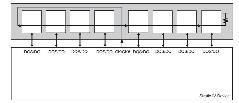
Figure 7-27. DDR3 SDRAM Unbuffered Module Clock Topology
