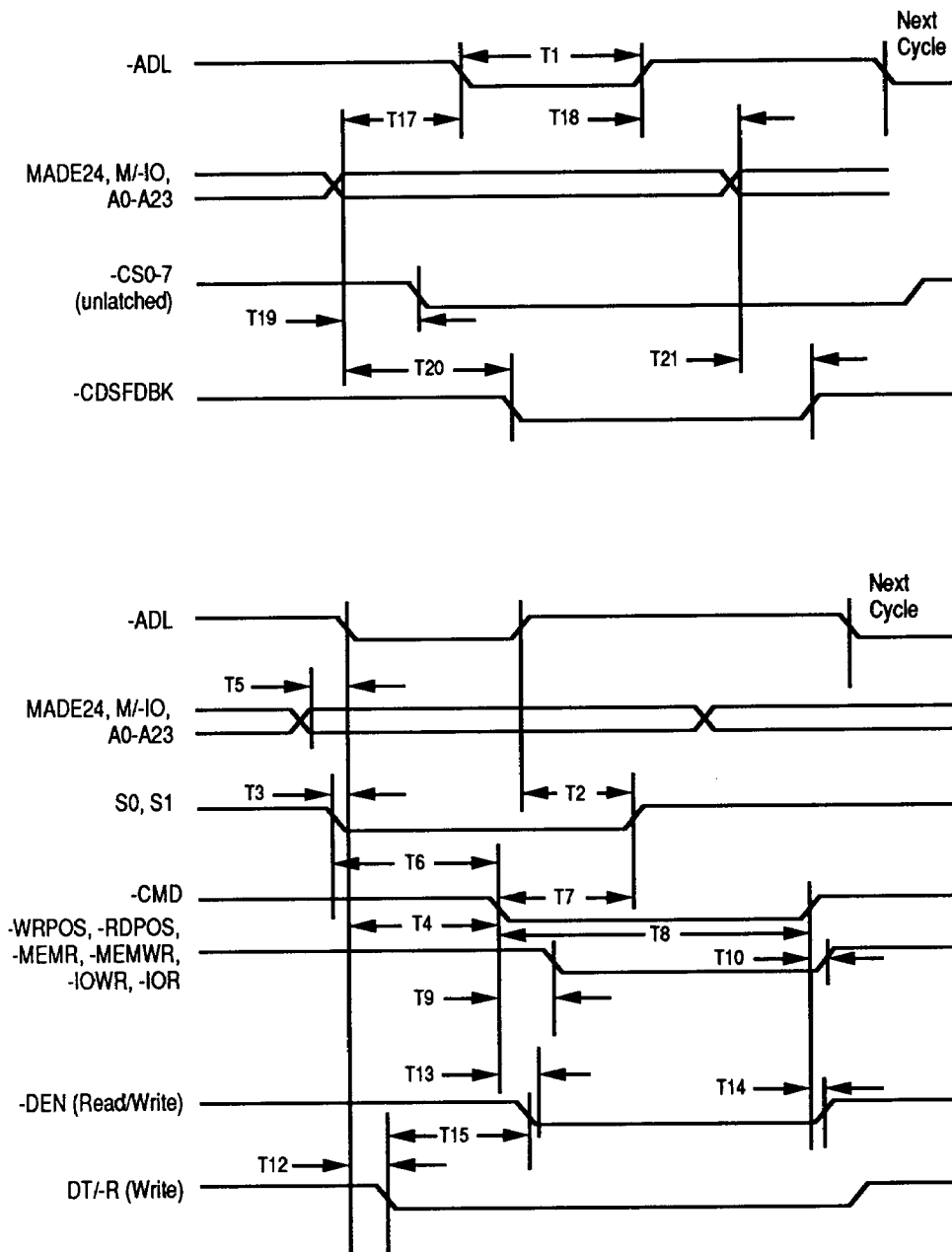
Figure 7. EPB2001 Waveforms
